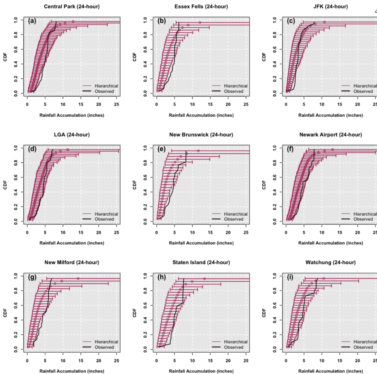
415 Figure A2: Empirical cumulative distribution function of the 24-hr ten-year return period event from SF hierarchical models for the nine stations (Central Park, LGA, New Milford – top to bottom left panel; Essex Fells, New Brunswick, Staten Island - top to bottom, middle panel; JFK, Newark, Watchung - top to bottom, right panel). The Empirical cumulative distribution function derived from the observed 24-hr ten-year return period field is also shown. The band depicts the 99% credible interval of the posterior simulations.
