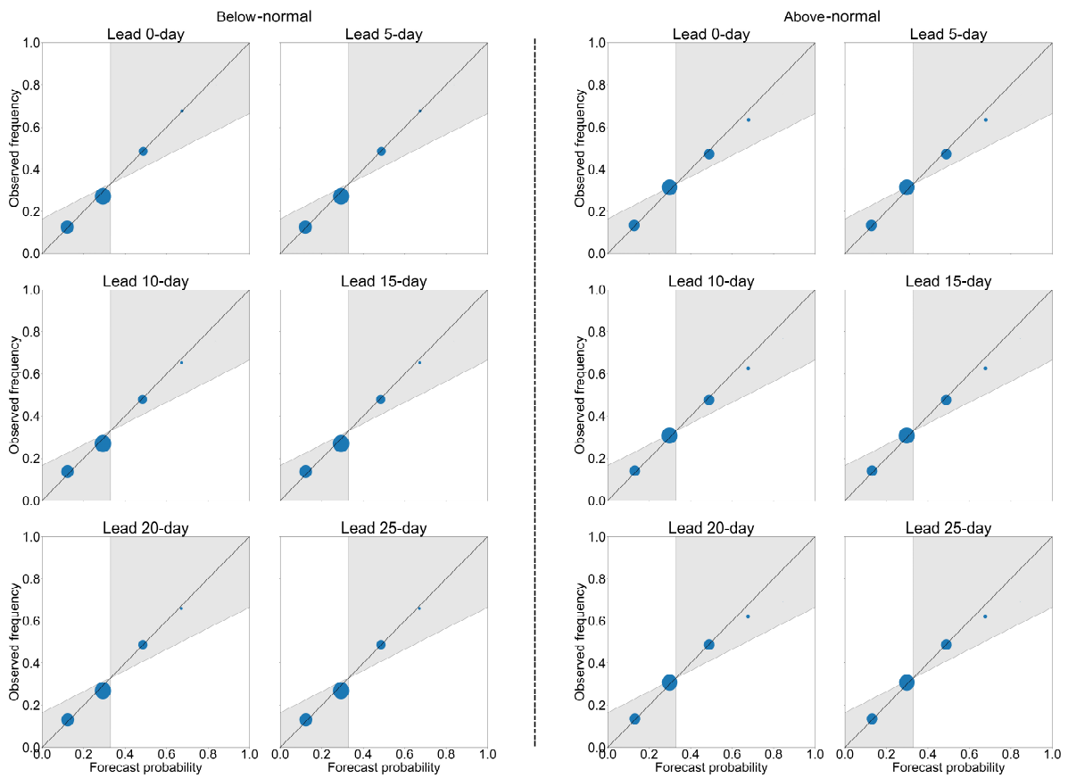
Figure 8. The attribute diagram of the STP-BHM model for the prediction of below-normal and above-normal events of pentad mean precipitation amount at different lead times. Forecast probability is binned with width of 0.2. The size of each dot represents the fraction of forecasts that fall into a particular probability bin.
