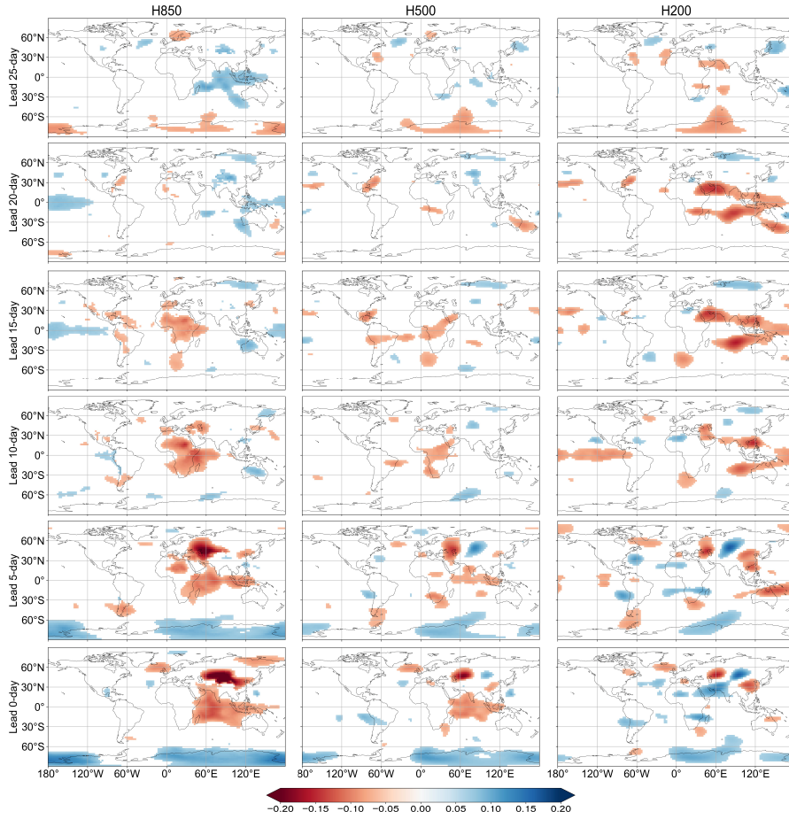
245 Figure 4. Same as Figure 3, but for H850, H500, and H200.
