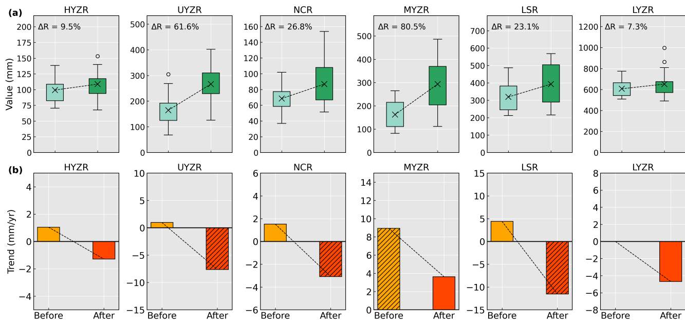
Figure 4. Water yield regime shifts in the entire UBR basin. (a) Magnitude of water yield changes. Black "x" signal shows the mean of water yield in each boxplot. (b) Direction of water yield changes. The black hatching represents the statistically significant trend ( p < 0.05 ). The color of boxes represents before (light color) and after (dark color) Tp period.
