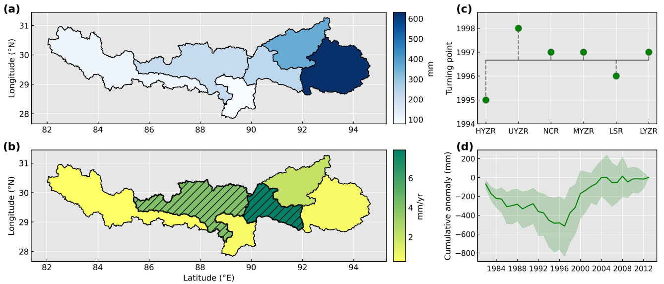
Figure 3. Long-term water yield changes in the entire UBR basin. (a) The mean annual values by averaging water yield from 1982 to 2013. (b) The temporal trends detected by the Mann-Kendall Sen's slope method. The black hatching represents statistically significant ( p < 0.05 ) trends. (c) The turning points detected by the Pettitt method. (d) The cumulative anomaly curve of water yield. The solid green line represents the ensemble expectation of cumulative anomaly curves of water yield for the entire UBR basin (green shading).
