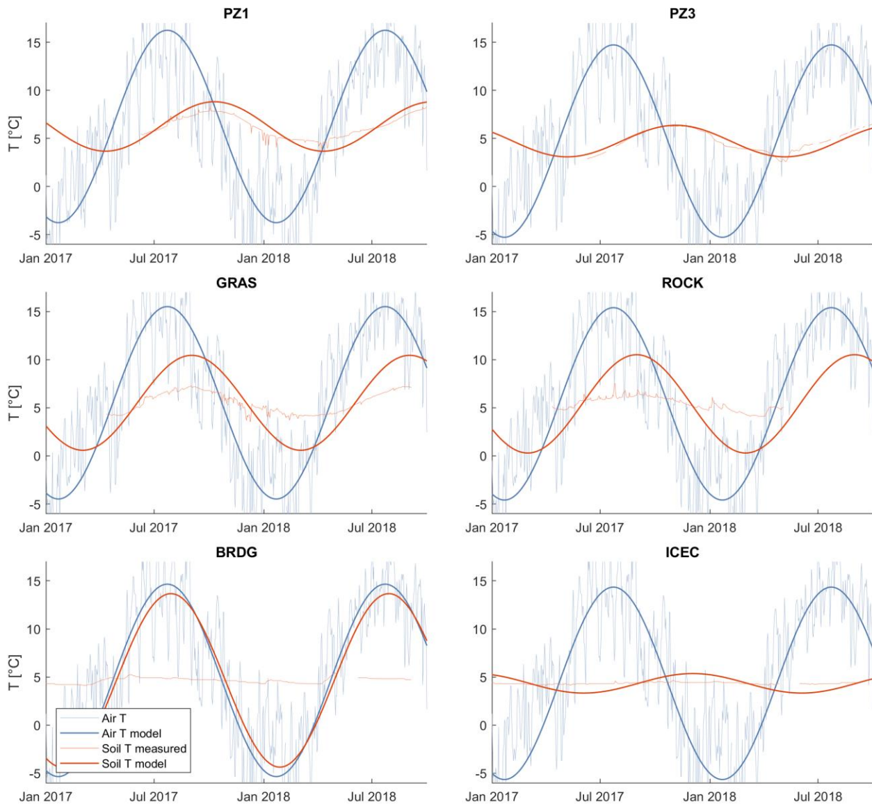
Figure 9. Measured and modeled air and soil temperature for 2 piezometers (PZ1 and PZ3) and 4 springs (GRAS, ROCK, BRDG and ICEC).
