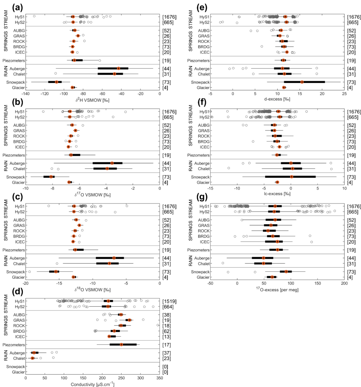
410 Figure 4. Range of \delta^2\text{H} , \delta^{17}\text{O} , \delta^{18}\text{O} , conductivity, d-excess, lc-excess and ^{17}\text{O} -excess for stream, springs, groundwater, rainfall, snowpack, glacier, and vegetation water samples. For measurements of the same water type (STREAM, SPRINGS, RAIN), the lowest sampling elevation is given on top, the highest on the bottom. The left and right end of each box show the 25 th and 75 th percentiles and the middle point is the median. The whiskers go up to 1.5 times the interquartile range; values beyond the whiskers (outliers) are marked with circles. The values on the right y-axis of the figures are the number of samples in each category. Note that there are no conductivity measurements for snowpack and vegetation water samples. For ^{17}\text{O} -excess the values of vegetations samples are out of the box (median 572 ‰, 25 th and 75 th percentiles are 374 ‰ and 742‰, resp., and whiskers are from 31 ‰ to 8329 ‰). 415
