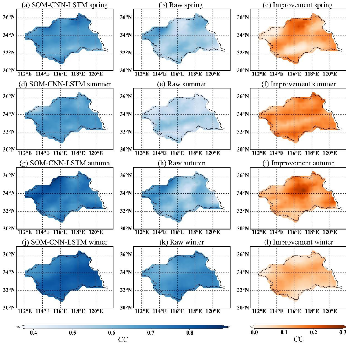
285 Figure 8 Spatial distributions of the CC for SOM-CNN-LSTM method and raw forecasts at the lead time of 1 day. The third column is the improvement of CC in spring, summer, autumn and winter.
