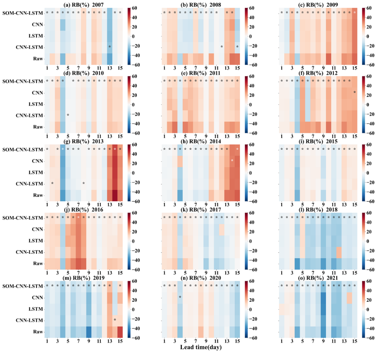
Figure 9 RB of different methods for each summer over 1-15 lead days from 2007 to 2021. The “*” indicates the best method with the lowest RB for each lead time.
