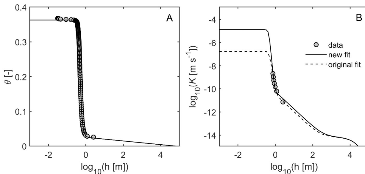
Figure 8: Same data as in Fig 1 (bottom). New scheme with vGmn as basic retention function and \tau_s fixed at 0.094 was fitted to the data (new fit). For comparison, the original fit using Ks as adjustable parameter is given by dashed lines. Note that the new scheme has one adjustable parameter less.
