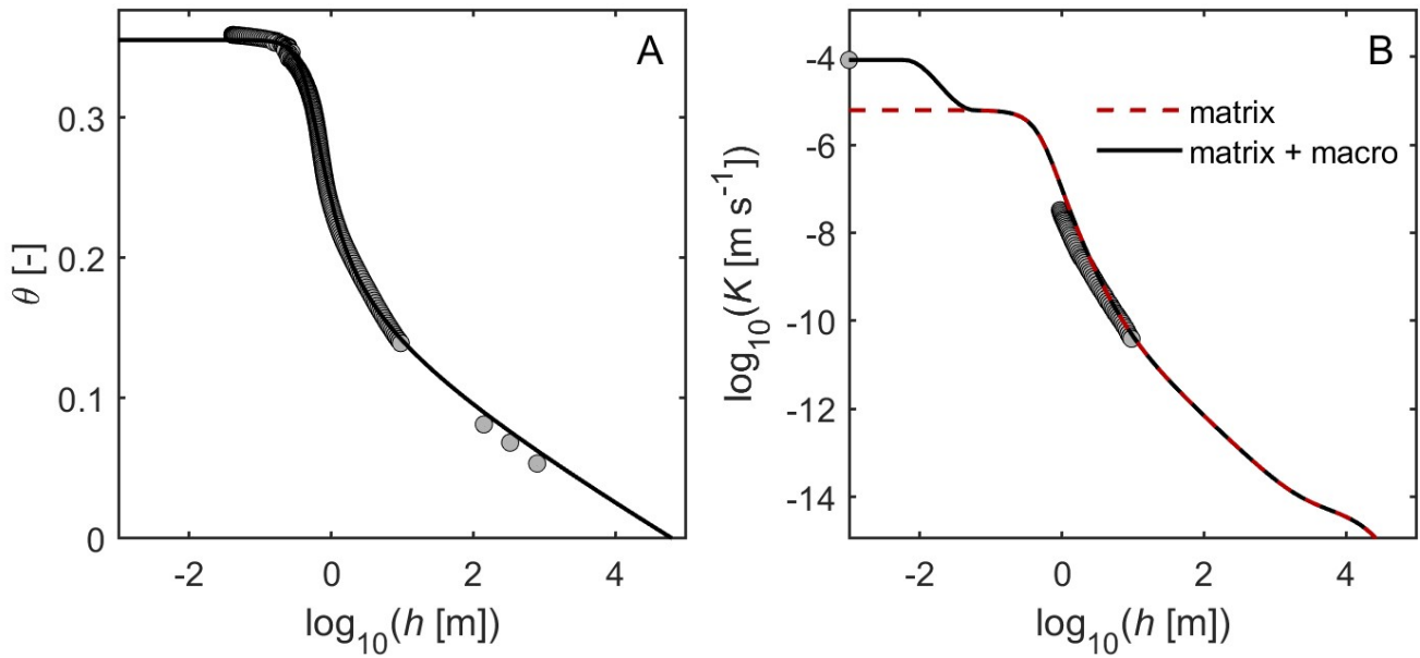
Figure 10: Application of the interpolation scheme given by Eq. (24) to the data set shown in Fig. 1 (top). The FX-PDI model was fitted to the water retention data and K(h) was predicted from dryness to h = 0.06 m.
