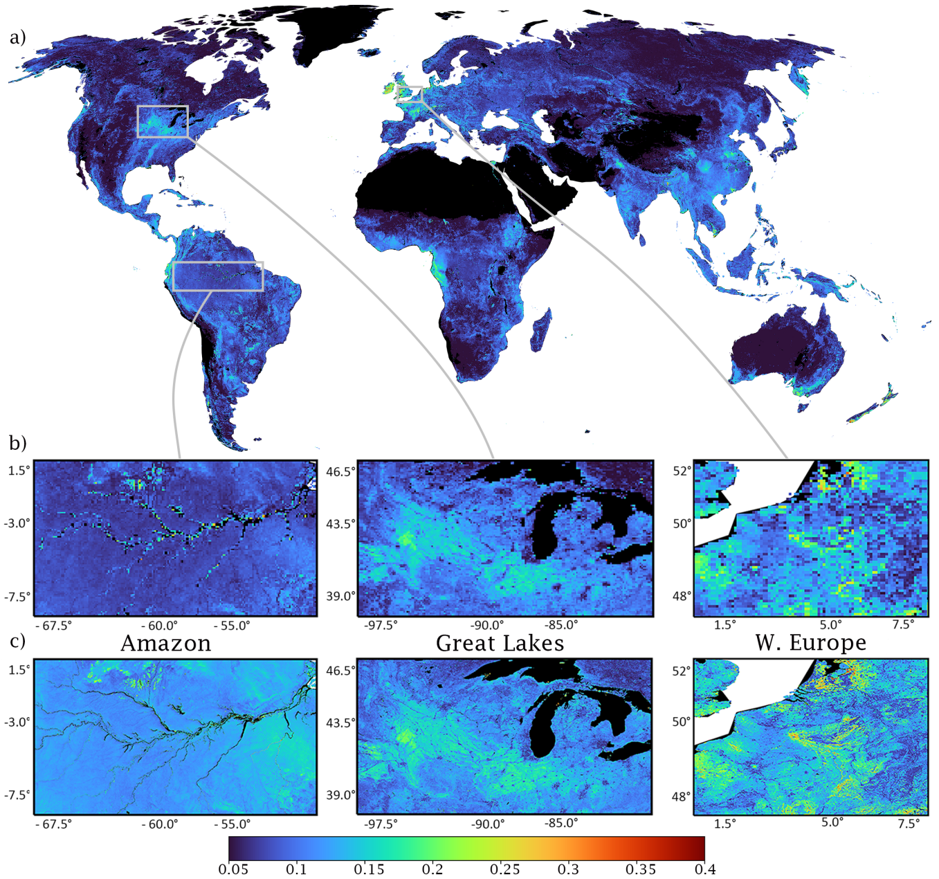
Figure 5. (a) RMSE calculated for the predicted evi using a RF model. Zoomed in inserts show Amazon Basin as representative of forest land cover, Great Lakes as a representative of croplands and Western Europe for predicted evi values by the model representative of urban land cover over at the (ab) 0.1° and (bc) 0.01°.
