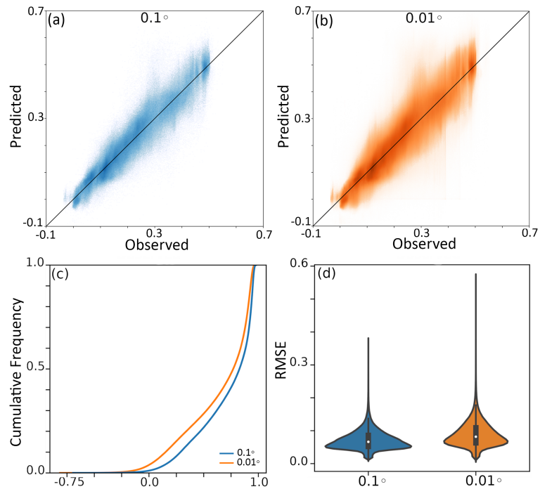
Figure 7. : (a) Scatter plot of observed and predicted evi at 0.1^\circ and (b) 0.01^\circ ; Cumulative distribution function for (c) Pearson Correlation Coefficients overall for all grid points at 0.1^\circ (blue) and 0.01^\circ (orange) , (d) violin plot of RMSE for all grid points at 0.1^\circ and 0.01^\circ
