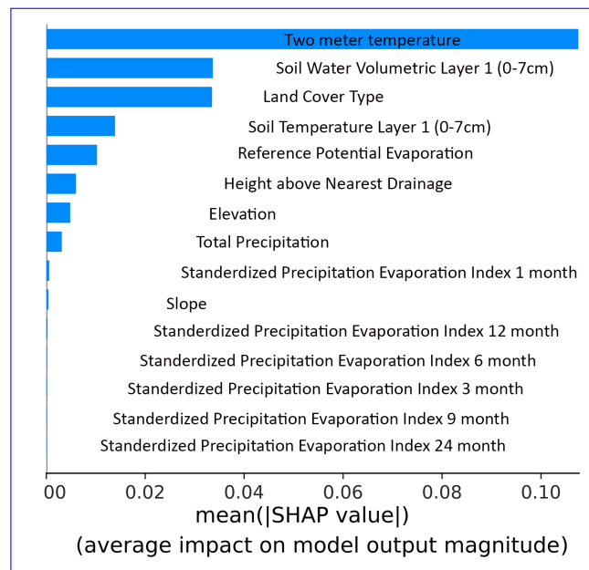
Figure 4. Feature importance for the RF based predicted evi at 0.1^\circ . The features are ordered by level of importance, with higher mean SHAP values indicating higher importance.
