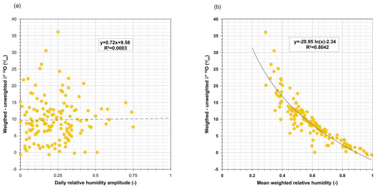
365 Figure A4: Dependence of the differences between the daily limiting \delta^* values obtained with-time averaged meteorological conditions (unweighted) and those weighted by PET (weighted) on a) the daily amplitudes of relative humidity and b) the weighted daily relative humidity (b). Equations are shown only to demonstrate the dependences.
