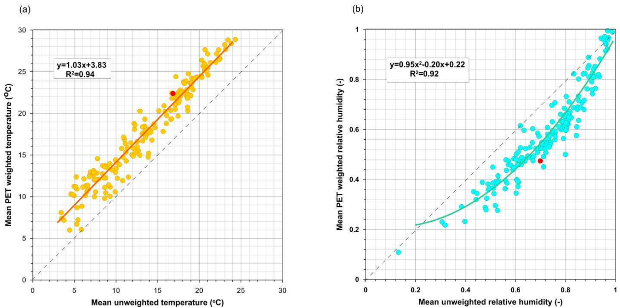
355 Figure A2: Comparison of the differences in daily a) temperature and b) relative humidity when 5-minute readings were time-averaged (unweighted) or weighted with potential evapotranspiration. The red dots represent the conditions on the date shown in Figure 5. The dashed line shows the 1:1 relationship.
