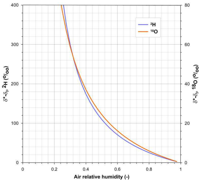
320 Figure 3: Relationship between air relative humidity and the differences between the limiting isotopic compositions ( \delta^* ) and the isotopic composition of precipitation ( \delta_p ), for ^2\text{H} and ^{18}\text{O} calculated using equation (2). Temperature is set at 20^\circ\text{C} .
