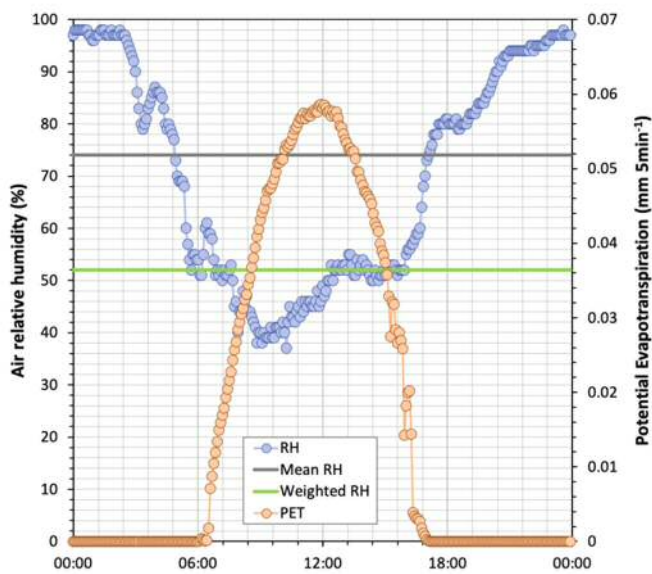
325 Figure 4: Time series of air relative humidity and potential evaporation for 4 September, 2020 (five-minute time steps). The mean relative humidity and relative humidity weighted by evaporation flux are also shown.
