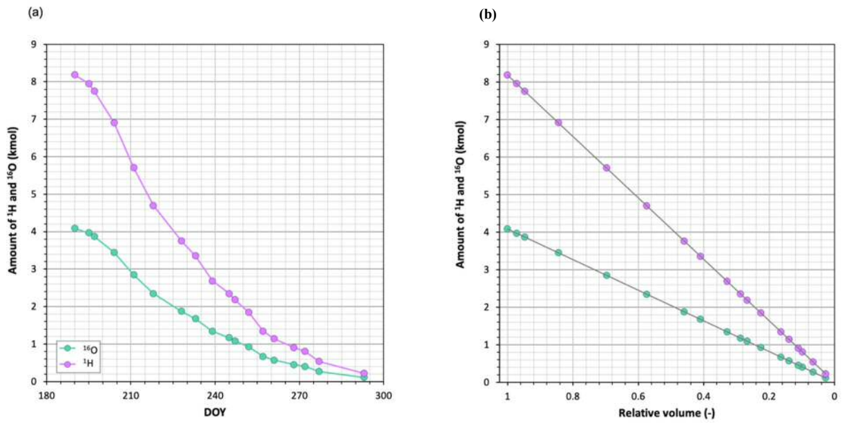
350 Figure A1: Amount of light isotopes in the water during the experiment, a) for the date and b) for the relative residual volume, calculated using Equation (10). Evaporation rates always exceeded condensation ones, even during the late periods of heavy isotope depletion.
