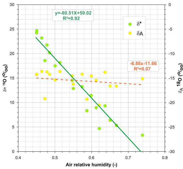
Figure 6: Weekly estimates of ^{18}\text{O} isotopic composition, limiting ( \delta^* ) and in air moisture ( \delta_A ), in relation to relative humidity. Vertical scales are offset 30 \text{ }^0/_{00} from each other.
