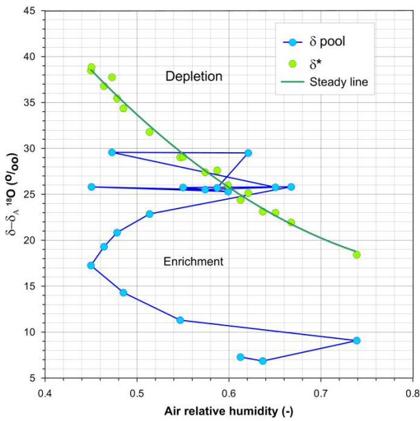
Figure 7: Evolution of the weekly differences between the isotopyisotopic composition of water and air, plotted in relation to air relative humidity (from bottom to top). The green line that connects the \delta^*-\delta_A points is a second order polynomial, shown only as visual reference.
