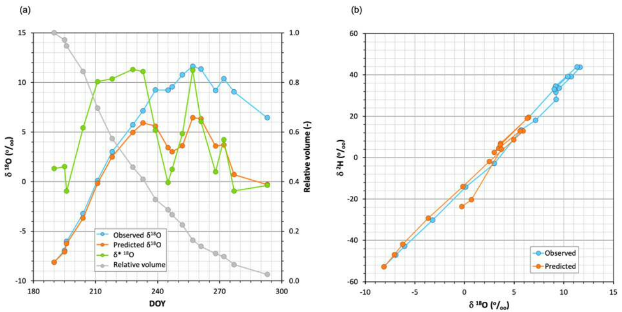
315 Figure 2: a) Time series of \delta^{18}\text{O} observed in the pan water together with (unweighted) predicted and limiting \delta^*^{18}\text{O} values when equation (1) was applied, using the weekly-averaged air temperature and relative humidity of the period studied. The relative residual volume curve is also indicated. b) Dual plot of the \delta^{18}\text{O} observed and predicted during the period studied. Predictions were clearly poor here where unweighted meteorological data were used.
