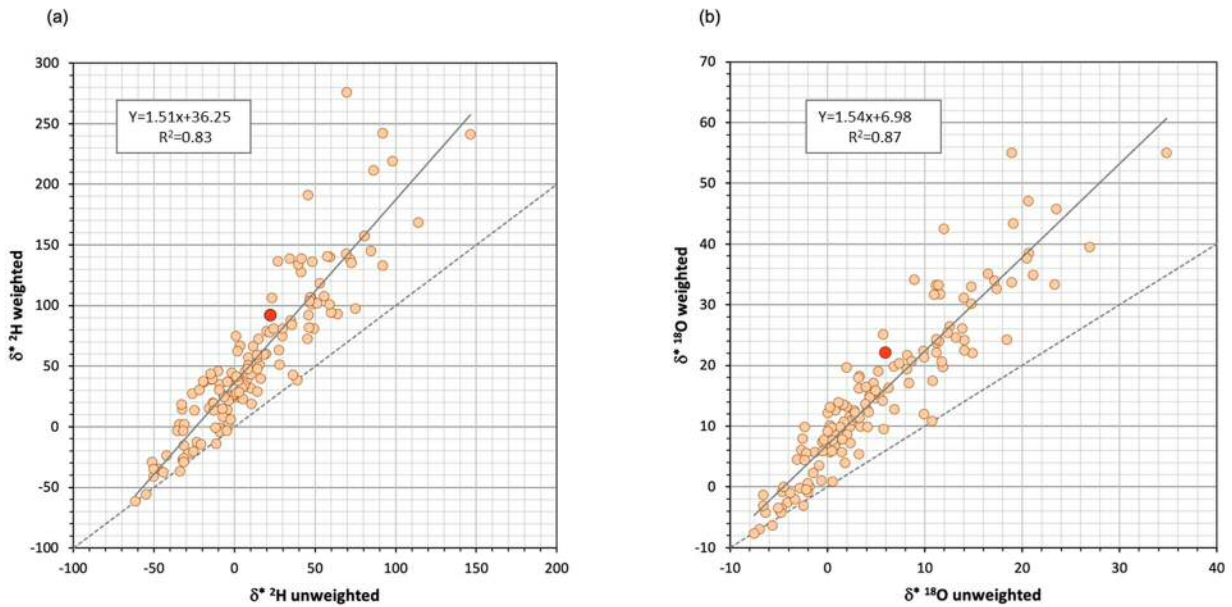
360 Figure A3: Comparison of the daily limiting compositions \delta^* for a) ^2\text{H} and b) ^{18}\text{O} when 5-minute readings were time-averaged (unweighted) or weighted with potential evapotranspiration. Low \delta^* values show the least differences because these correspond to days with high relative humidity, as shown in Figure 3 and A4. The red dots represent the conditions on the date shown in Figure 5. The dashed line shows the 1:1 relationship.
