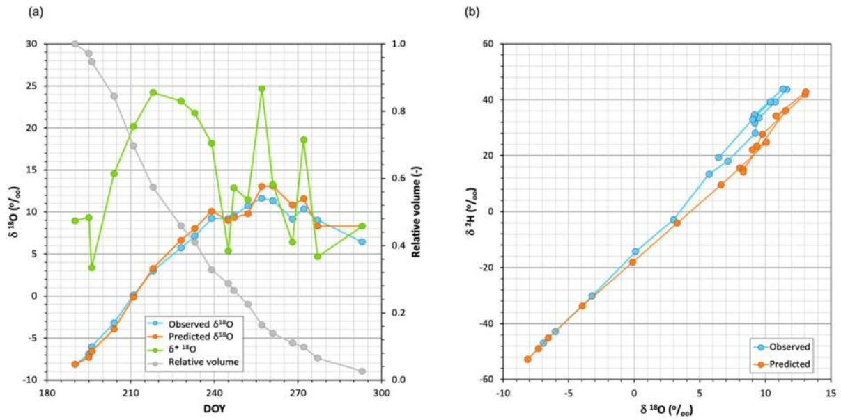
330 Figure 5: a) Time series of \delta^{18}\text{O} observed in the pan water together with (weighted) simulated and limiting \delta^* \text{ }^{18}\text{O} values when equation (1) was applied, using evaporation flux-averaged air temperature and relative humidity conditions. b) Dual plot of the \delta^{18}\text{O} observed and predicted during the period studied.
