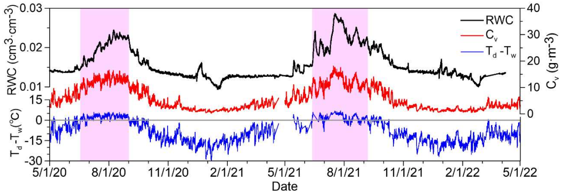
Figure 8. The fluctuating apparent rock moisture ( RWC ), vapor concentration ( C_v ), and the difference between dew point temperature and wall temperature ( T_d - T_w ). The zones in purple represent the periods with positive T_d - T_w and high rock moisture.
