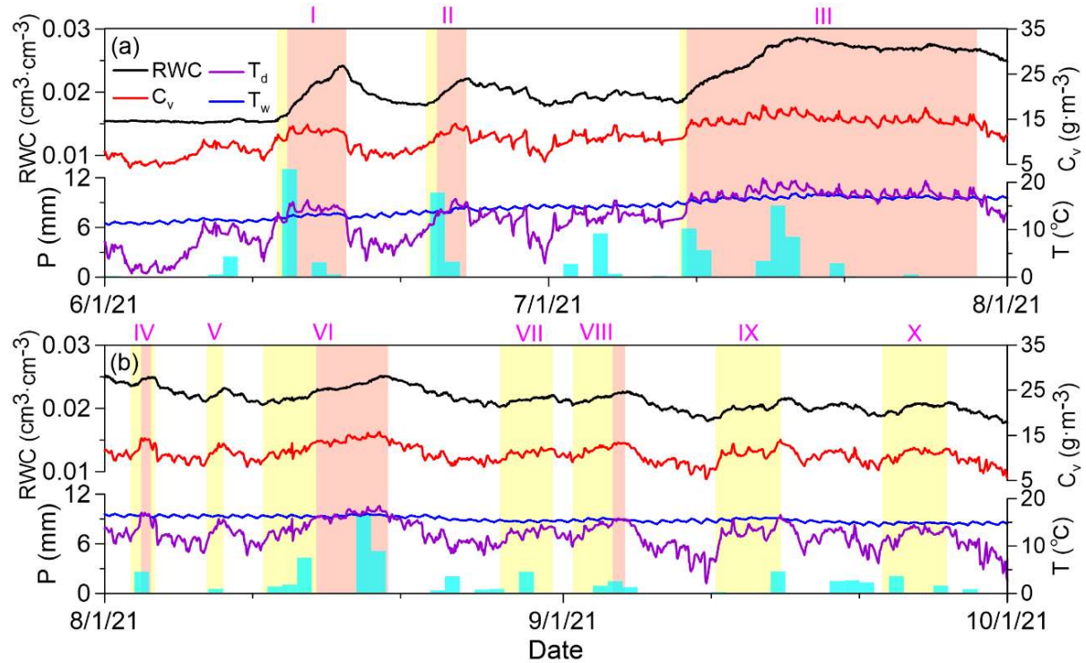
Figure 9. Plots showing the responses of rock water content ( RWC ) to precipitation ( P ), vapor concentration ( C_v ), dew point temperature ( T_d ) and wall temperature ( T_w ) in summer of 2021. The zones in yellow have increasing RWC, and zones in red have increasing RWC as well as positive T_d - T_w .
