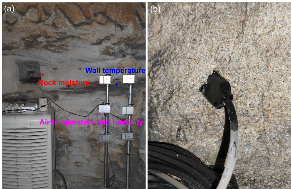
Figure 2. (a) The arrangements of sensors for rock moisture, wall temperature, air temperature and relative humidity in the north wall of Cave #9. (b) A photo showing the installed FDR sensor in Cave #9.
