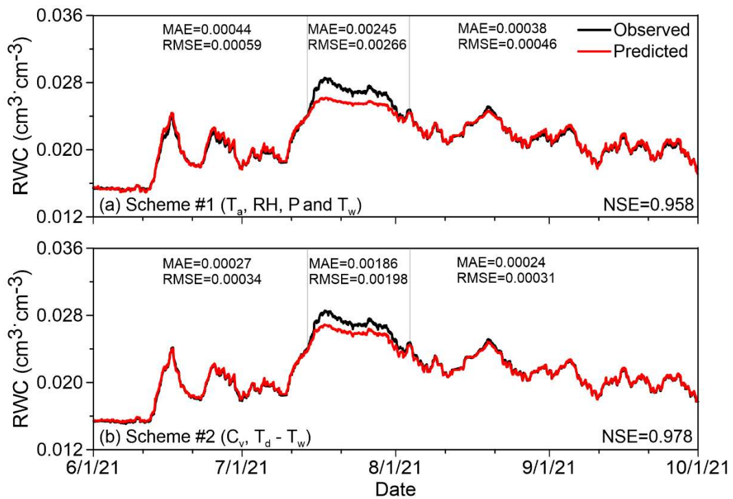
Figure 6. The predicted and measured RWC obtained by two schemes. (a) Scheme #1 using four directly measured variables; (b) Scheme #2 using two calculated variables controlling vapor condensation. Also shown are NSE of the whole time series, MAE and RMSE of three different stages.
