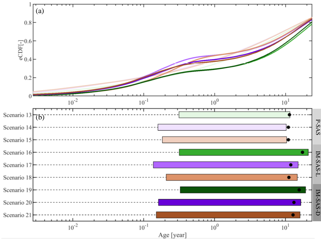
1275 Figure 9. Stream flow TTDs derived from the 9 model scenarios with the different associated calibration strategies of P-SAS (scenarios 13 – 15), IM-SAS-L 1280 scenarios 16 – 18) and IM-SAS-D model implementations (scenarios 19 – 21). The TTDs represent the volume weighted average daily TTDs for the modelling period 01/10/2001 – 31/12/2016. Green shades represent the TTDs inferred from \delta^{18}\text{O} (from lighter to darker for scenario 13, 16, 19), the purple shades represent TTDs inferred from ^3\text{H} (from lighter to darker for scenario 14, 17, 20), the brown lines represent TTDs inferred from combined \delta^{18}\text{O} and ^3\text{H} (brown shades from lighter to darker for scenario 15, 18, 21); the black dots in (b) indicate the mean transit time for each model scenario. Note that the mean transit time was estimated by fitting Gamma distributions to the volume-weighted mean TTDs of each individual scenario.
