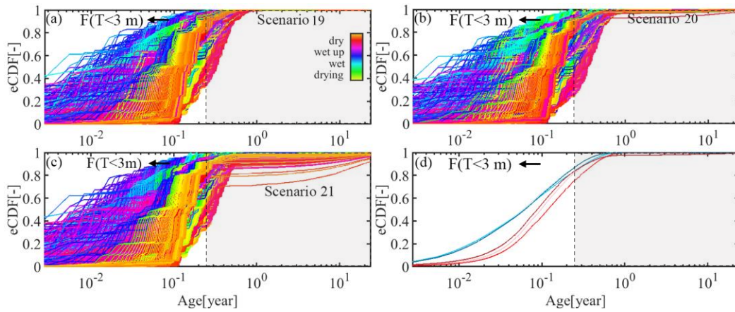
1300 Figure 11. Daily transpiration ( E_a ) TTDs extracted from the most balanced model solutions of the IM-SAS-D implementations (scenarios 19 – 21), based on (a) calibration strategy C_{\delta^{18}O, Q} (scenario 19), (b) calibration strategy C^3_{H, Q} (scenario 20) and (c) calibration strategy C_{\delta^{18}O, ^3H, Q} (scenario 21). The line colors represent the transition between dry and wet periods. Panel (d) shows the volume weighted average TTDs for the wet and dry periods, respectively. The light shades represent calibration strategy C_{\delta^{18}O, Q} (scenario 19), the intermediate shades indicate calibration strategy C^3_{H, Q} (scenario 20) and the dark shades are calibration strategy C_{\delta^{18}O, ^3H, Q} (scenario 21). For illustrative purposes, also the fraction of water younger than 3 months F(T < 3 \text{ m}) is indicated.
