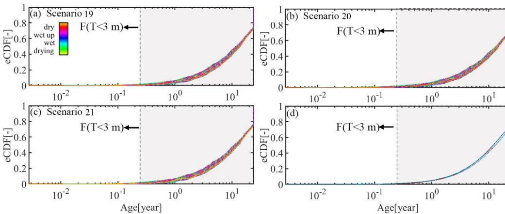
1305 1310 Figure 12. Daily groundwater ( S_s ) RTDs extracted from the most balanced model solutions of the IM-SAS-D implementations (scenarios 19 – 21), based on (a) calibration strategy C_{\delta^{18}O, Q} (scenario 19), (b) calibration strategy C^3_{H, Q} (scenario 20) and (c) calibration strategy C_{\delta^{18}O, ^3H, Q} (scenario 21). The line colors represent the transition between dry and wet periods. Panel (d) shows the volume weighted average RTDs for the wet and dry periods, respectively. The light shades represent calibration strategy C_{\delta^{18}O, Q} (scenario 19), the intermediate shades indicate calibration strategy C^3_{H, Q} (scenario 20) and the dark shades are calibration strategy C_{\delta^{18}O, ^3H, Q} (scenario 21). For illustrative purposes, also the fraction of water younger than 3 months F(T < 3 \text{ m}) is indicated.
