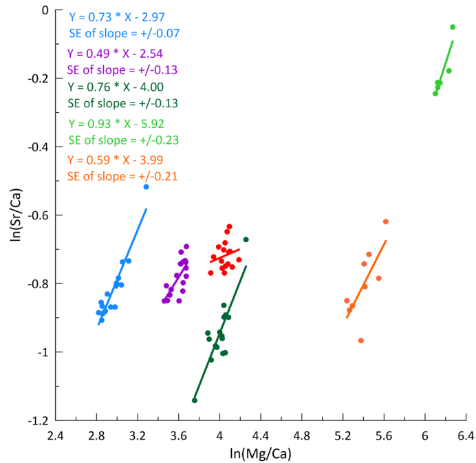
745 Fig. A1: Sinclair plot showing a clear relationship between Mg/Ca and Sr/Ca affected by PCP. The data set of Playground does not yield a statistically significant (p-value too large) slope to be reported. Slope error (SE) is also given and often overlaps with the proposed slopes (Sinclair et al., 2012; Wassenburg et al., 2020). Additionally, varying partitioning coefficients affect the slopes.
