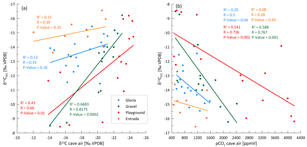
775 Fig. A5: a) Correlation of drip water \delta^{13}\text{C}_{\text{DIC}} and cave air \delta^{13}\text{C}_{\text{air}} to test potential gas exchange with cave air. Pearson correlation coefficient (R), R^2 and p-value suggest reasonable correlations for Playground and Gravel but not for Entrada and Gloria; b) modest inverse correlation of \text{pCO}_2 and \delta^{13}\text{C}_{\text{DIC}} suggests degassing during periods of low cave air \text{pCO}_2 . Significant correlations are found for Playground and Gravel.
