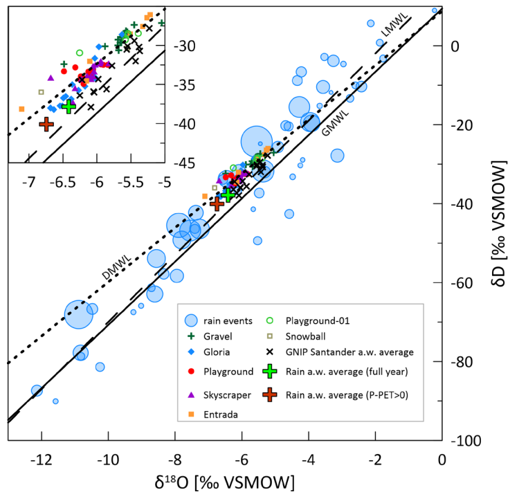
475 Fig. 9: Meteoric water lines of drip water and local rain events. The size of the blue bubbles indicates the rain amount of individual rain events between February 2015 to February 2016 (Moreno et al., 2021). The green cross represents the full annual amount weighted average of local precipitation. The brown cross accounts for positive P-PET months only (recharge). Black crosses reveal the interannual variability of rainfall represented by amount weighted annual average of GNIP station Santander for 2000-2015. For the 2019-2021 cave monitoring, drip water DMWL: \delta D = 7.01 \delta^{18}O + 9.72 , where R^2=0.83 ; stippled. Local rainwater LMWL \delta D = 8.5 \delta^{18}O + 15.1 , where R^2=0.92 ; dashed (data from Moreno et al. (2021)) and global meteoric water line (GMWL) \delta D = 8.0 \delta^{18}O + 480 10 (Craig, 1961). The MWL for GNIP Santander 2000-2015 (not shown) is fairly similar to the dashed line.
