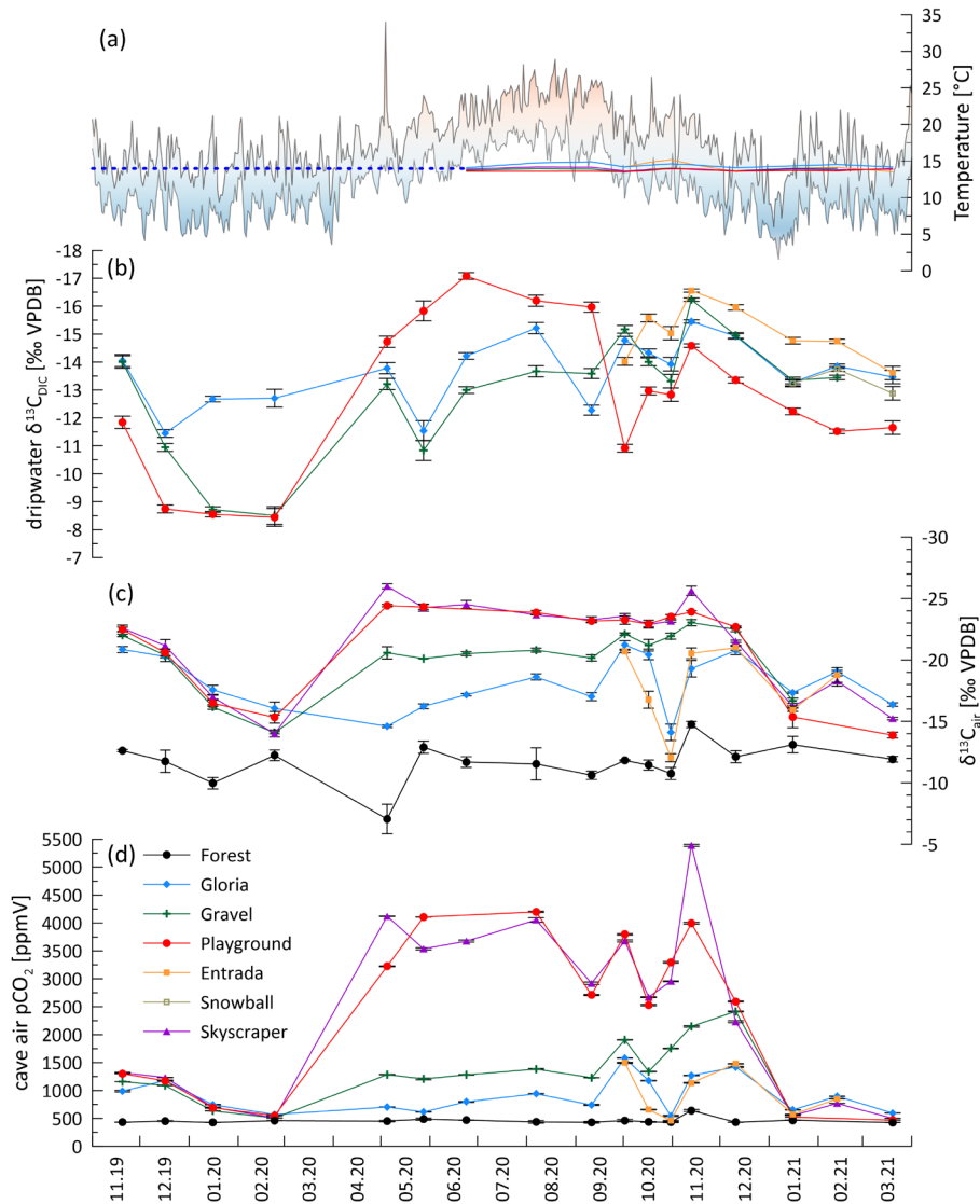
265 Fig. 2: Cave air conditions and drip water DIC over time. a) Daily outside temperature range (min-max) in Llanes (Aemet, 2021) and cave air temperature. The blue dashed line extrapolates the constant cave air temperature. b) drip water \delta^{13}C_{DIC} , c) cave air \delta^{13}C_{air} and d) cave air pCO_2 . Note the reversed y-axes for B and C.
