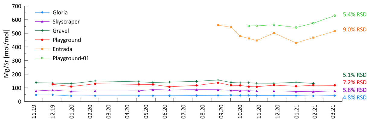
655 Fig. 12: Constant Mg/Sr ratio over monitoring period indicates congruent bedrock dissolution. Higher RSD is recorded at Entrada (orange) which might be influenced by aeolian marine aerosols input near the cave entrance (Fig. A7). Mg contributed from dolomitized zones might contribute to substantially higher Mg/Sr at sites like Entrada and Playground-01.
