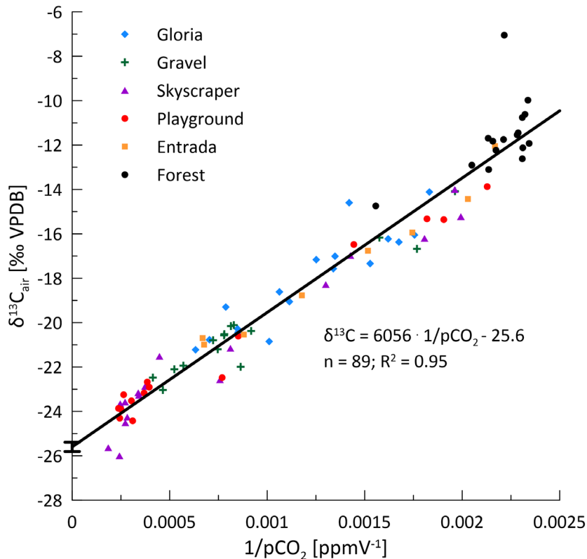
390 Fig. 8: Keeling plot based on cave air measurements. The mixing line (black line) suggests a mixture between the two endmembers of respired soil air (-25.6‰) and atmospheric air (-11.6‰).
