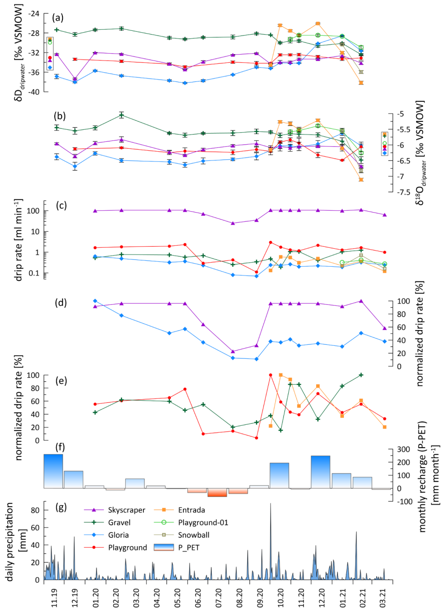
Fig. 3: Hydrological conditions and water chemistry. a) hydrogen isotopic drip water composition ( \delta D_{\text{dripwater}} ), b) oxygen isotopic drip water composition ( \delta^{18}O_{\text{dripwater}} ), c) absolute drip rate (log-scale) d) normalized drip rate of less responsive drip sites (Skyscraper and Gloria), e) normalized drip rate of strongly responsive drip sites with different lags to recharge (Playground, Gravel, Entrada), f) monthly recharge calculated by subtracting potential evapotranspiration (PET) from precipitation (P) and g) daily precipitation recorded in Llanes (Aemet, 2021). In a) and b) Data points in a box next to the y-axis represent amount weighted average values of each drip site.
