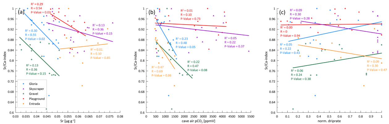
750 Fig. A2: Checking potential driver of PCP indicated by Sr/Ca-index. Weak relationships between Sr/Ca-index and a) the Sr concentration (representing soil \text{CO}_2 ) and b) cave air \text{pCO}_2 (Gloria and Gravel) emerge. However, c) drip rate is hardly related to the Sr/Ca index. A stronger \text{CO}_2 gradient between drip water and air in contact with drip water increases PCP potential. Also, longer exposure time at slower drip rates might increase degassing, thus favor PCP.
