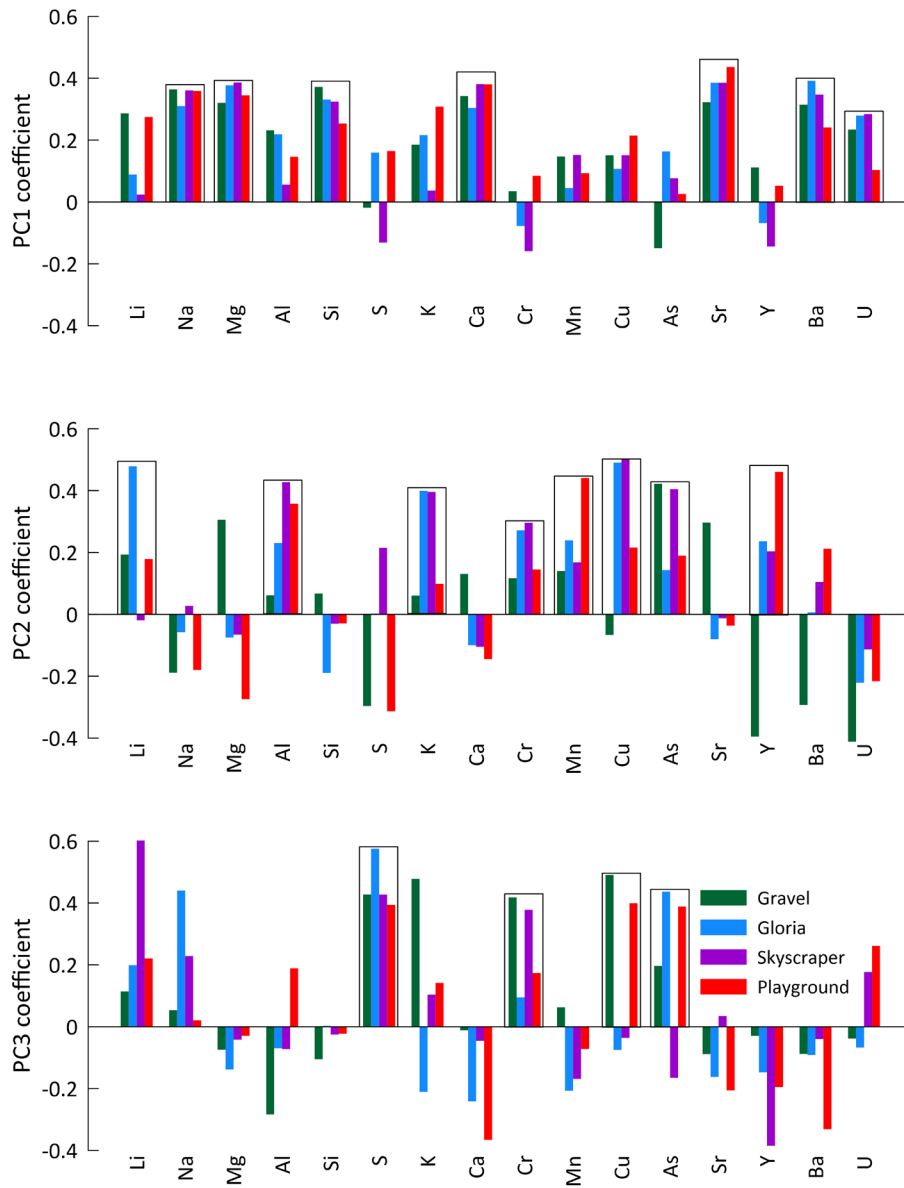
345 Fig. 5: First three principal components (PC 1-3) of the principal component analysis (PCA) applied on the element concentration of drip water from individual drip sites. Boxes indicate elements of generally similar behavior controlled by specific PCs.
