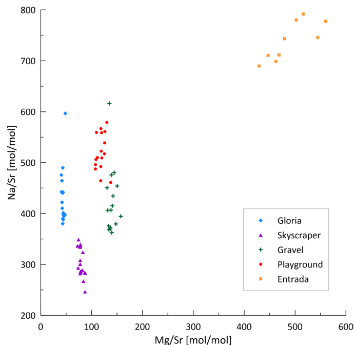
785 Fig. A7: Mg/Sr vs. Na/Sr scatter plot highlighting the likely marine aerosol contribution at Entrada as a positive correlation emerges. Drip sites deeper in the cave do not indicate a relationship between Na and Mg, thus are not affected by marine aerosols.
