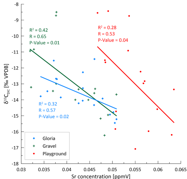
780 Fig. A6: Sr concentration is inversely correlated with \delta^{13}\text{C}_{\text{DIC}} . This is interpreted as a bedrock dissolution signal since higher soil \text{pCO}_2 with microbial (negative) imprint driven by temperature results in stronger dissolution.
