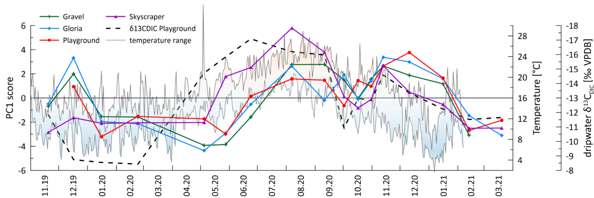
580 Fig. 11: The temporal evolution of the score of PC 1 (colored curves) suggests stronger bedrock dissolution in summer and early autumn as well as winter likely due to higher soil pCO 2 . A clear relationship with temperature (daily min-max with color shading) and δ 13 C DIC (dashed line, note inverted y-scale) emerges suggesting an interrelationship.
