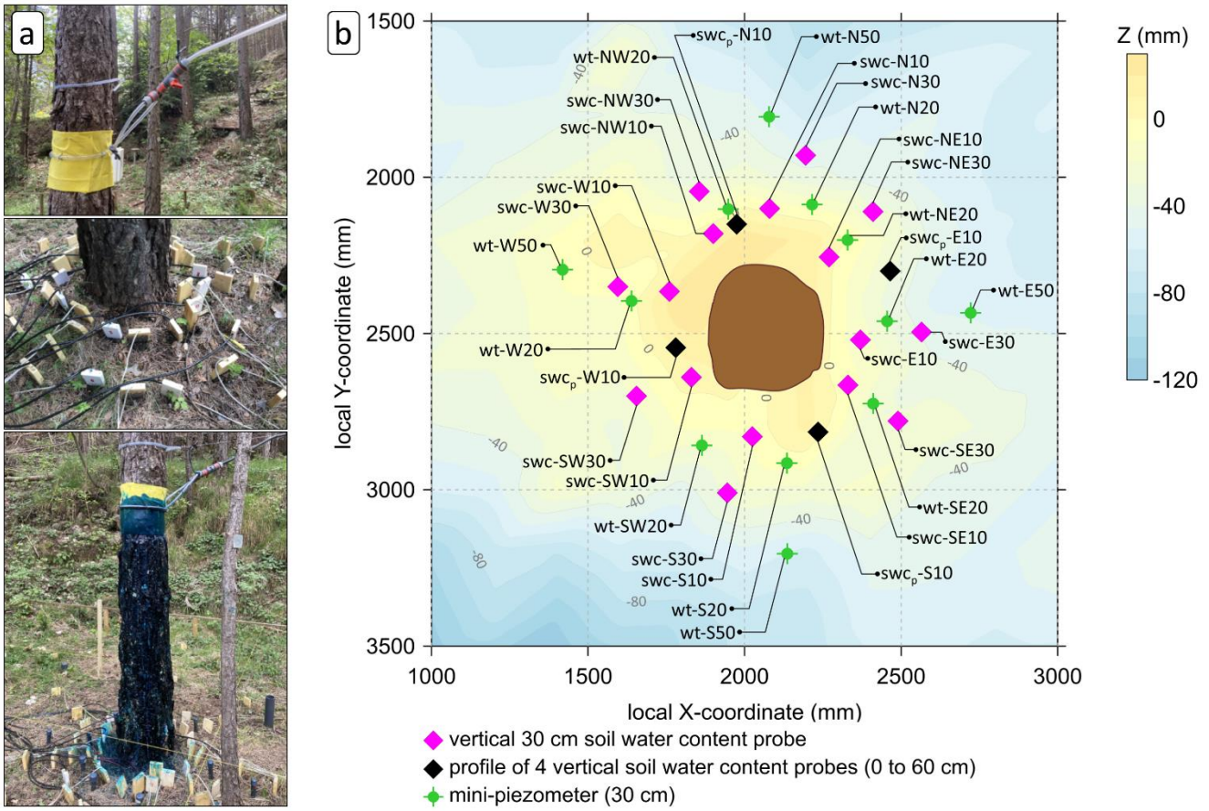
610 Figure 1. Tracer experiment set-up. (a) Photographs of the artificial stemflow set-up and soil instrumentation before and after (last picture) the tracer experiment. (b) Top view of the experimental area showing microtopography and location of instruments around the selected tree. swc = vertical 30 cm soil water content probe; swc p = profile of 4 vertical soil water content probes; wt = mini-piezometer (30 cm deep); N = North, E = East, S = South, W = West; number in the label of each location refers to the distance (cm) from the tree trunk.
