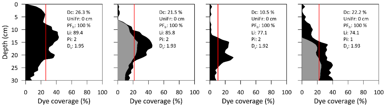
745 Figure 8. Dye coverage (black = soil-stained areas; grey = root-stained areas) of the different soil profiles at a distance of (a) 40 cm, (b) 25 cm and (c) 10 cm from the tree trunk. Root-stained areas refer to the area occupied by stained roots in line with the soil profile. Parameters to quantify the degree of preferential flow are shown within each graph (Dc = dye coverage (%), also shown as red line; UniFr = uniform infiltration depth (cm); PF fr = preferential flow fraction (%); Li = length index; Pi = peak index; D s = fractal dimension).
