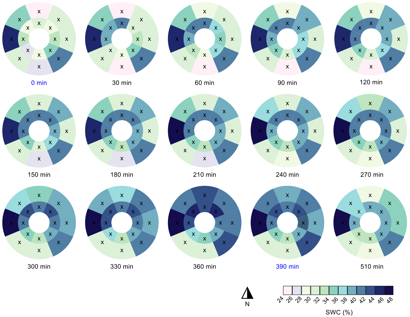
690 Figure 5. Time series of spatial patterns of volumetric soil water content (SWC) during the experiment. Artificial stemflow was initiated at t = 0 min and stopped after around t = 390 min (highlighted in blue). Cross marks denote TDR sensors (approximate location) and the white circle represents the tree trunk.
