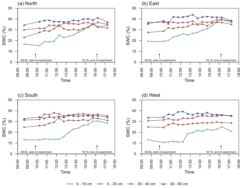
765 Figure 6. Temporal evolution of volumetric soil water content (SWC) in depth profiles of each cardinal direction during the stemflow experiment.
