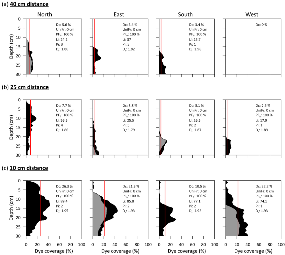
Figure 8. Dye coverage (black = soil-stained areas; grey = root-stained areas) of the different soil profiles at a distance of (a) 40 cm, (b) 25 cm and (c) 10 cm from the tree trunk. Root-stained areas refer to the area occupied by stained roots in line with the soil profile. Parameters to quantify the degree of preferential flow are shown within each graph ( D_c = dye coverage (%), also shown as red line; UniFr = uniform infiltration depth (cm); PF fr = preferential flow fraction (%); Li = length index; Pi = peak index; D s = fractal dimension).
