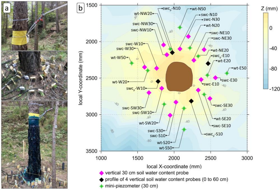
Figure 1. Tracer experiment set-up. Pictures(a) Photographs of the artificial stemflow set-up and soil instrumentation before and after (last picture) the tracer experiment. (b) Top view of the experimental area showing microtopography and location of instruments around the selected tree. swc = vertical 30 cm soil water content probe; swc p = profile of 4 vertical soil water
