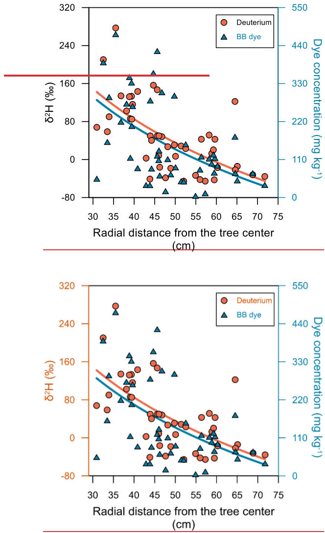
845 Figure 10. Relationships between travel distance (three-dimensional coordinate system) with deuterium isotopic composition and Brilliant Blue FCF dye concentration for the 63 soil samples. Solid lines indicate logarithmic fits.
