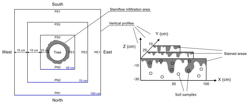
Figure 2. Top and vertical view of experimental plot with squares indicating the different location of the vertical soil profiles excavated and the sampling around the tree (left). Schematic of vertical soil profiles with dye patterns (right).
