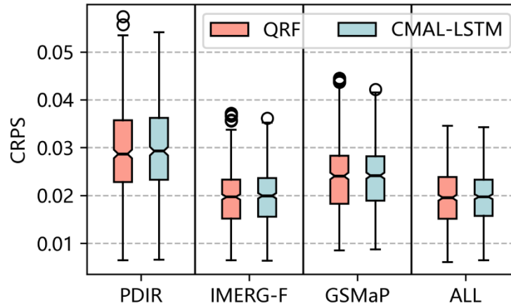
385 Figure 4. The boxplot of CPRS for different post-processing experiments.
