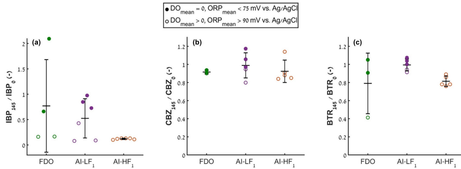
Fig. 6. Concentrations of IBP (a), CBZ (b) and BTR (c) at a depth of 145 cm during FDO, AI-LF 1 and AI-HF 1 . The concentrations are normalized to the inlet concentration of the same species. The horizontal line represents the arithmetic mean, and the error bars show plus and minus one SD. Values below detection limit (DL) were regarded with DL/2. DLs of the relevant species are available in the supplement (Table S7). Filled dots indicate samples taken when the mean DO throughout the column was zero and the mean ORP was lower than 75 mV, while unfilled dots indicate samples taken when the mean DO was higher than zero and the mean ORP was higher than 90 mV. In FDO, samples were taken and analyzed for only one replicate. In addition, for CBZ and BTR, the first sample from each experiment (taken at t \sim 4.3 h) was excluded as an outlier since it showed much lower concentrations than the others, apparently due to temporary retardation of the compound as a result of its interactions with soil components.
