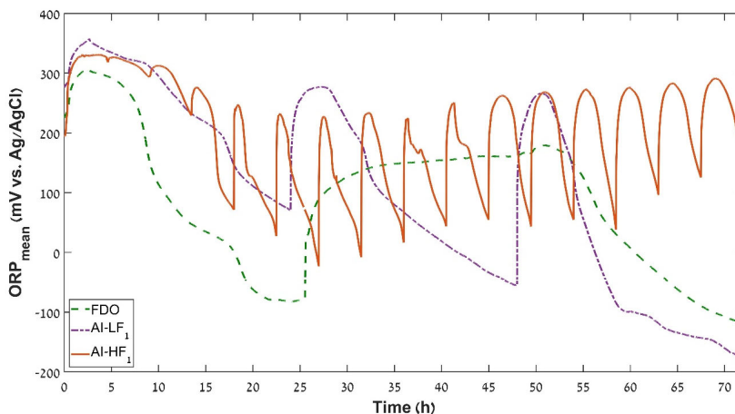
Fig. 4. ORP mean (arithmetic mean of the ORP measured at depths of 25, 65, 105 and 145 cm below soil surface) during FDO, AI-LF 1 and AI-HF 1 .
