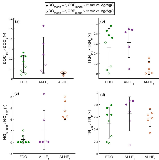
Fig. 5. Concentrations of DOC (a), TKN (b), \text{NO}_3^- (c) and TN (d) at a depth of 145 cm during FDO, AI-LF 1 and AI-HF 1 . All concentrations are normalized to the inlet concentration of the same species. The horizontal line represents the arithmetic mean and the error bars show plus and minus one SD. Values below quantitation limit (QL) were regarded with QL/2. QLs of the relevant species are available in the supplement (Table S7). Filled dots indicate samples taken when the mean DO throughout the column was zero and the mean ORP was lower than 75 mV, while unfilled dots indicate samples taken when the mean DO was higher than zero and the mean ORP was higher than 90 mV.
