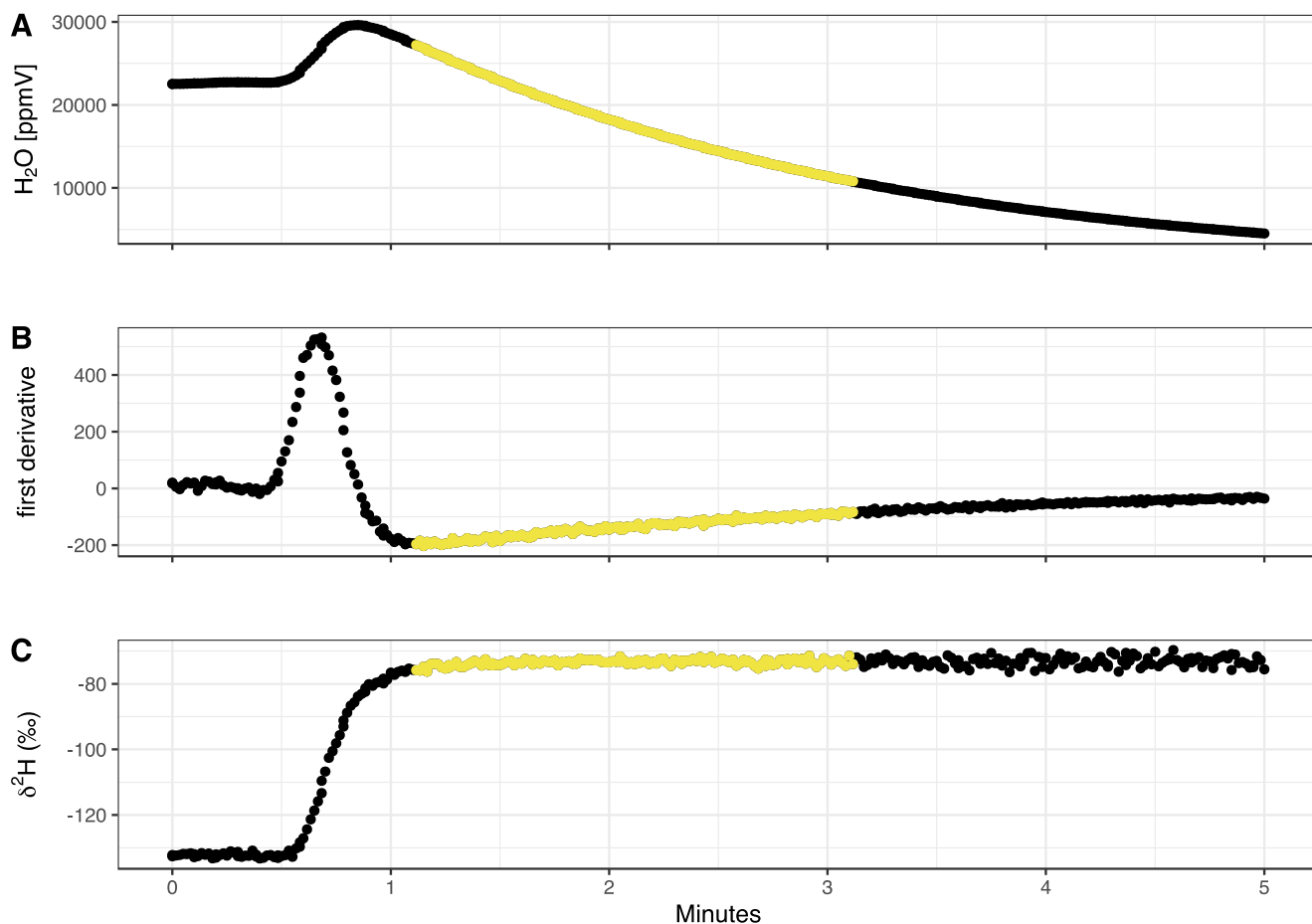
150 Fig. 2 Exemplified measurement data for the “heavy” source over a time period of five minutes. Vapour concentration (A), first 155 derivative of vapour concentration over time (B) and hydrogen isotopic composition (C). Following the criteria defined in the main text, we computed the mean of the isotopic composition ( \delta^2\text{H} and \delta^{18}\text{O} ) over the two minutes depicted by the yellow dots in the scheme.
