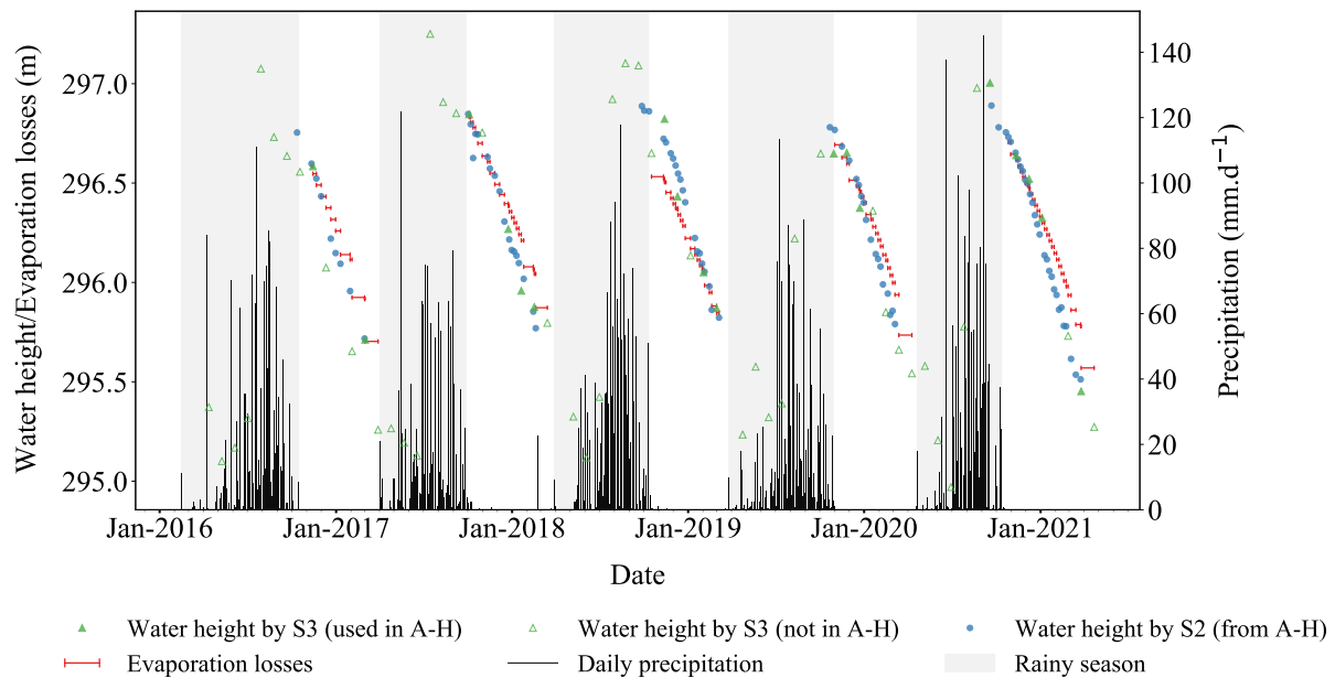
Figure 4. Water height time series from Sentinel-3 (S3) and Sentinel-2 (S2) data, along with the cumulated evaporation losses, daily rainfall and rainy season for Lake Tibin. The starting point to calculate evaporation losses is fixed to the water height at the first date in the dry season. The length of the red lines in the x-axis corresponds to the time between two successive water height samples.
