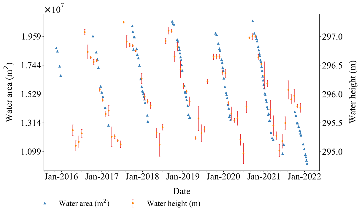
Figure 2. Time series of water areas (left y-axis, in blue) and water heights (right y-axis, in orange) with their associated median absolute deviation (orange bars), for the Tibin reservoir (see Table 1), located in the center north of the Burkina Faso.
