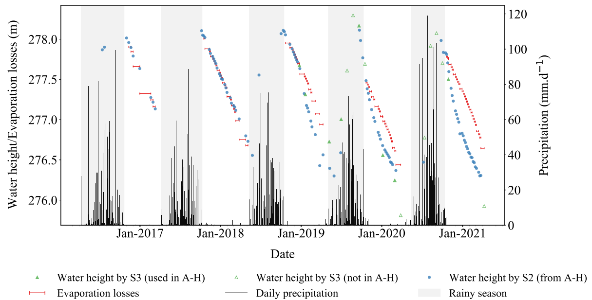
Figure 12. Water height time series from Sentinel-3 (S3) and Sentinel-2 (S2) data, along with the cumulative evaporation losses, daily rainfall, and rainy season for Lake Gomde. The starting point to calculate evaporation losses is fixed to the water height at the first date in the dry season. The length of the red lines in the x-axis corresponds to the time between two successive water height samples.
