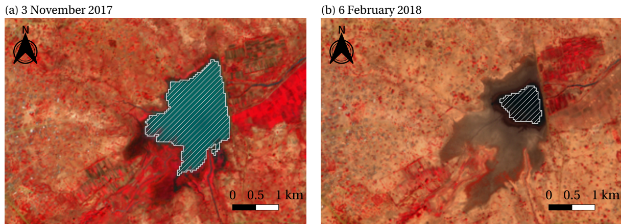
Figure 7. Sentinel-2 False Color images (NIR/Red/Green) of Manga reservoir surroundings with the lake contours (in white) obtained by thresholding on the MNDWI at (a) 3 November 2017 and (b) 6 February 2018. Active vegetation appears in red.
