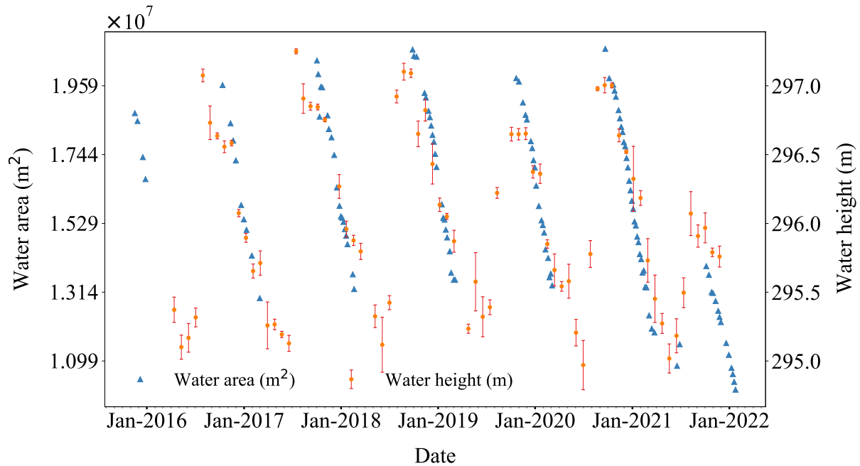
Figure 2. Time series of water areas (left y-axis, in blue) and water heights (right y-axis, in orange) with their associated median absolute deviation (orange bars), for the Tibin reservoir (see Table 1), located in the center north of the Burkina Faso.
