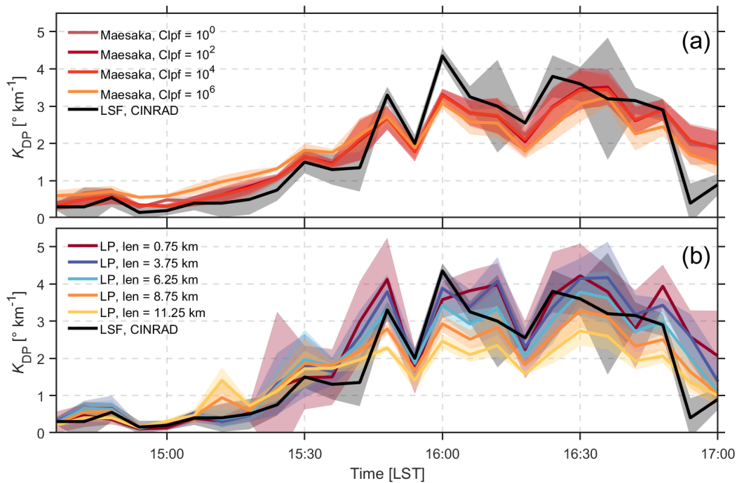
Figure 3. K_{DP} estimates using (a) Maesaka (2012) method and (b) LP over Zhengzhou national reference climatological station. Thick Thick lines and shading areas indicate the median values and standard deviations of K_{DP} at elevation angles of 1.5^\circ , 2.4^\circ , 3.3^\circ and 4.3^\circ . LP: linear programming method (Giangrande et al., 2013); LSF: least square fitting, the CINRAD's operational algorithm. Colored lines indicate different window length (len) used in LP.
