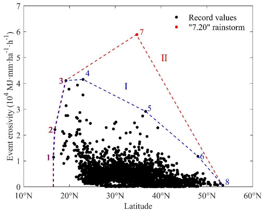
290 Figure 10. The maximum recorded event rainfall erosivity as a function of latitude for China. The point enclosed by the envelope curve I is the maximum event rainfall erosivity of each station from 1951 to 2020. The point enclosed by envelope curve II is the maximum event rainfall erosivity of each station from 1951 to 2021.
