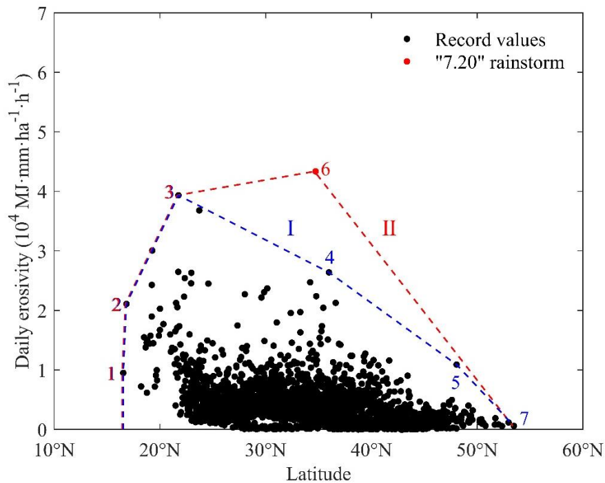
275 Figure 9. The maximum recorded daily rainfall erosivity as a function of latitude for China. The point enclosed by the envelope curve I is
