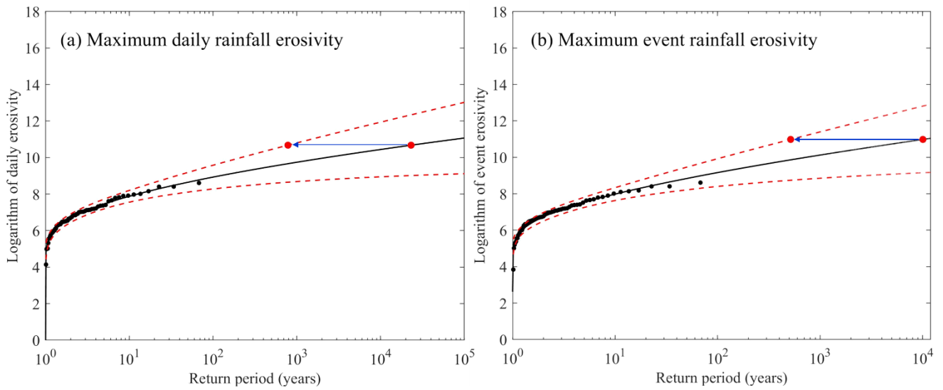
250 Figure 6. The logarithm of observed daily (a) and event (b) rainfall erosivity as a function of the return period assuming LP-III for Zhengzhou meteorological station. Black solid circles are observations from the period 1951-2020, the red solid circles indicate the “7.20” storm in 2021, the red dotted line is the upper and lower limit of 95% confidence interval, and the solid lines in black represent the fitted P-III distribution using the logarithm of observations from 1951-2020.
