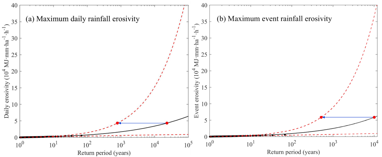
255 Figure 7. Observed daily (a) and event (b) rainfall erosivity as a function of the return period assuming LP-III for Zhengzhou meteorological station (Performed anti-logarithm conversion for Fig. 6)
