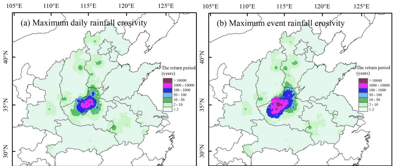
265 Figure 8. The return period of daily (a) and event (b) rainfall erosivity of the “7.20” storm in the study area.
