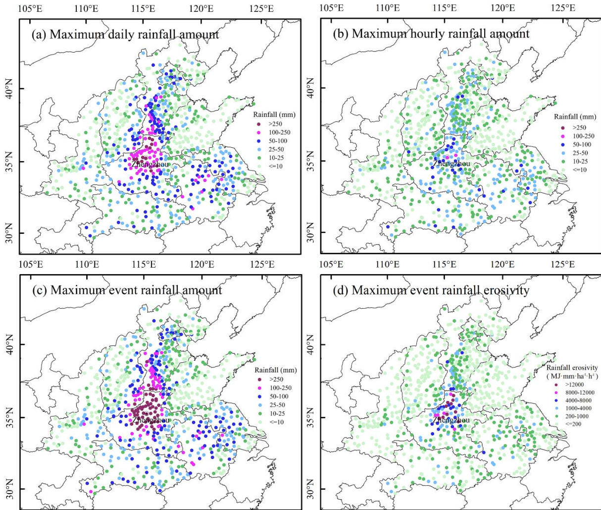
210 Figure 5. Spatial distribution of rainfall amount and rainfall erosivity associated with the “7.20” storm.
