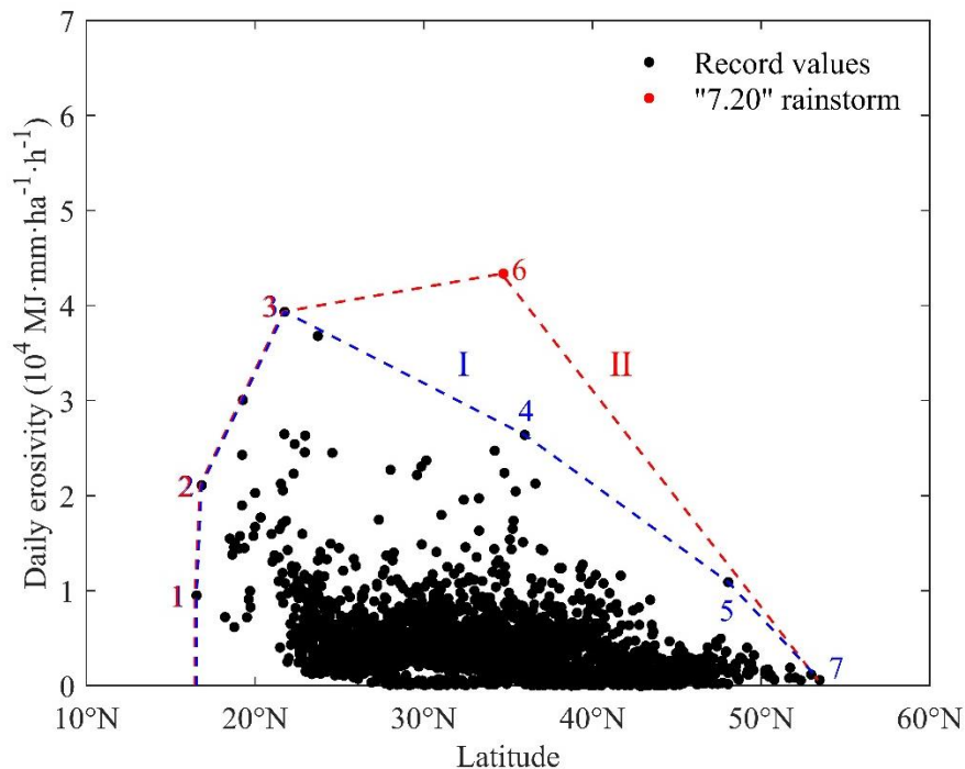
275 Figure 9. The maximum recorded daily rainfall erosivity as a function of latitude for China. The point enclosed by the envelope curve I is
