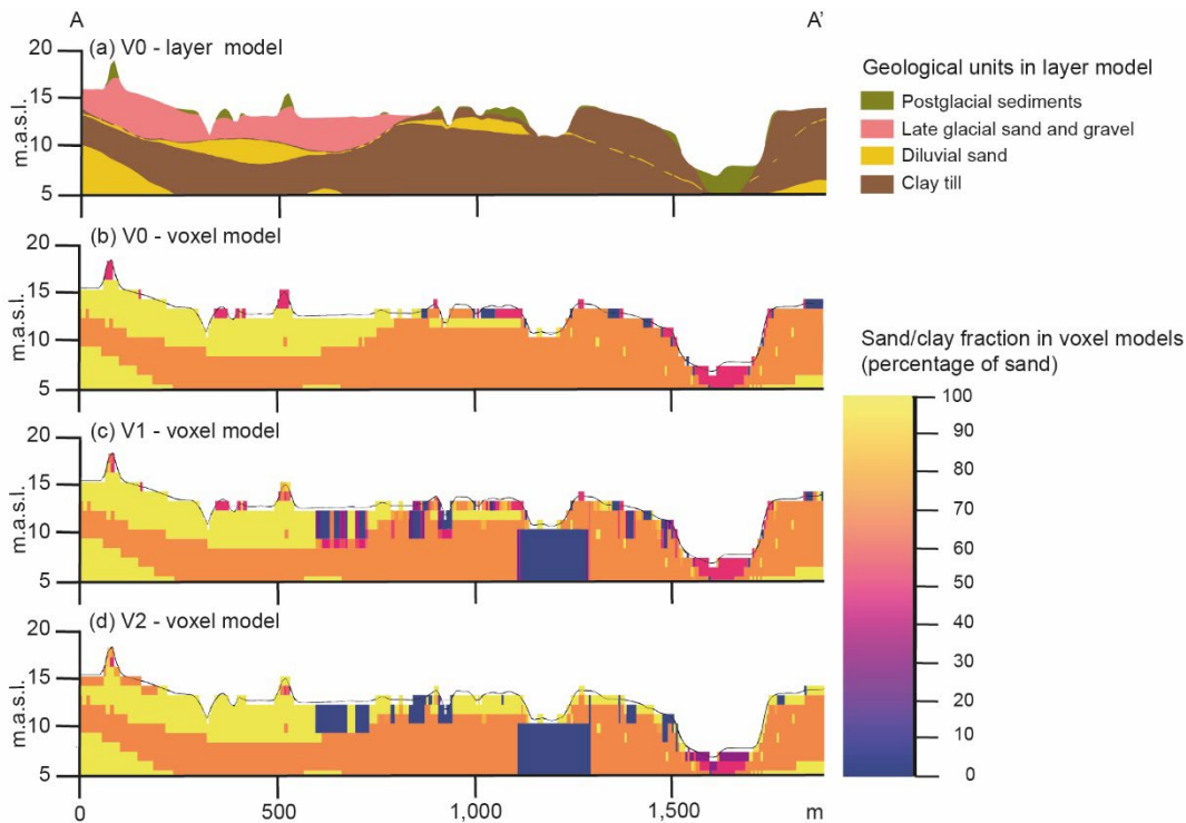
395 Figure 5. Profile A-A' from the geological models V0 – layer model (a), V0 – voxel model, (b) V1 – voxel model (c), and V2 – voxel model (d).
