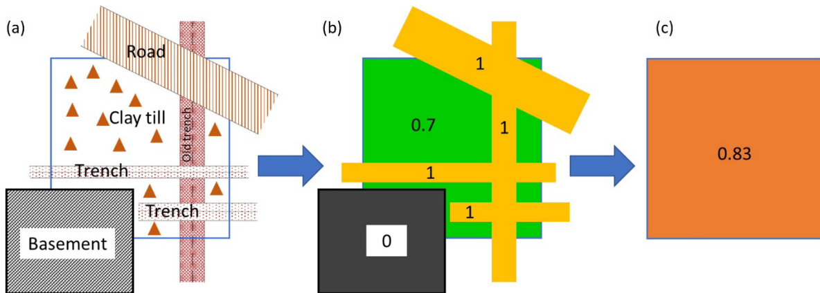
Figure 3. Workflow for setting the value of a voxel: (a) Voxel with clay till and anthropogenic subsurface infrastructures, (b) The corresponding sand/clay fractions, and (c) the resulting representative sand/clay fraction for the voxel, which is based on average according to volume.
