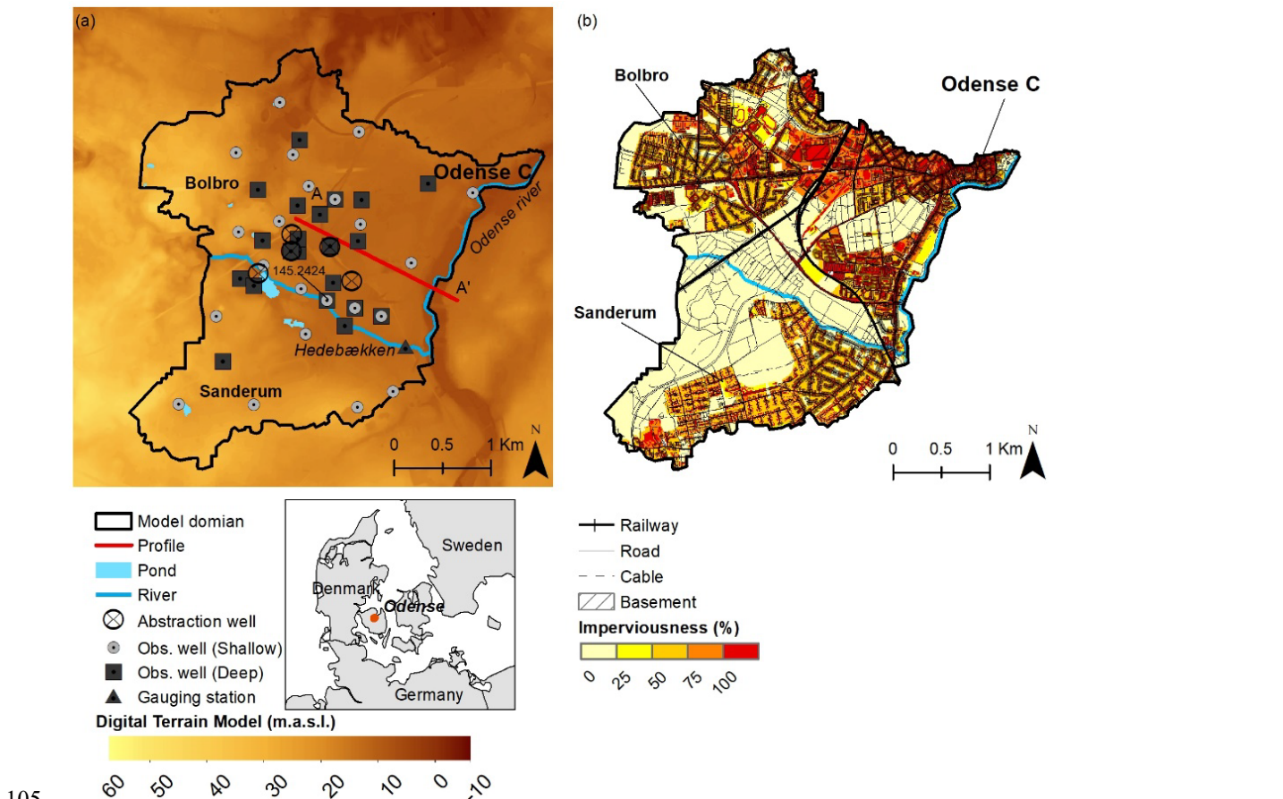
Figure 1. Maps of the model domain, a part of the city of Odense, Denmark. Panel (a) displays a digital terrain model from the Danish National Agency for Data Supply and Infrastructure (2019) with locations of observation points and abstraction wells provided by Vandcenter Syd A/S (2021). Panel (b) depicts the imperviousness of the land cover retrieved from Levin et al. (2012) and modified with data from Vandcenter Syd A/S (2019a) and subsurface infrastructure provided by Vandcenter Syd A/S (2019b) and the Danish Geodata Agency (2019).
