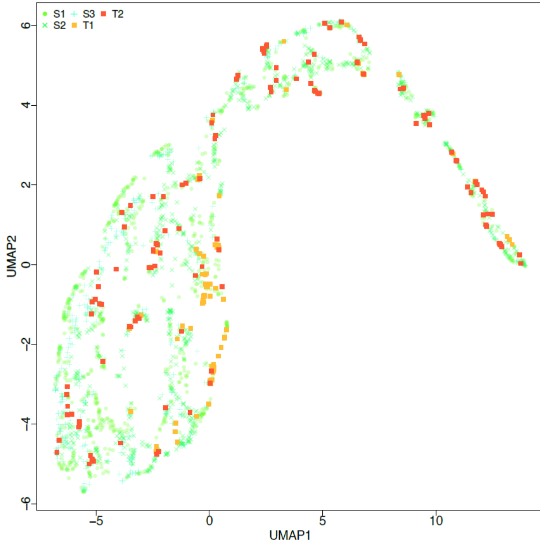
Figure 1. Uniform Manifold Approximation and Projection (UMAP) clustering of the source and target regions that are colored and symbolized by each catchment (Source Region 1 (S1)-North America, Source Region 2 (S2)-South America, Source Region 3 (S3)-Europe, Target Region 1 (T1)-South Africa, Target Region 2 (T2)-Central Asia)
