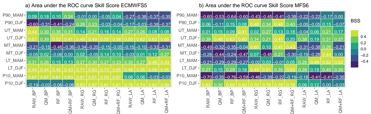
Figure 10. AUCSS of the detrended seasonal (DJF, MAM) snow depth forecasts in the lower (LT), middle (MT), upper (UT) tercile, as well as in the lower (P10) and upper (P90) extreme of the distribution, with respect to the climatological forecasts, using observations at the three stations as a reference, for a) ECMWF55 and b) MFS6 systems. Positive and negative AUCSSs are highlighted in shades of green and blue, respectively colors, respectively.
