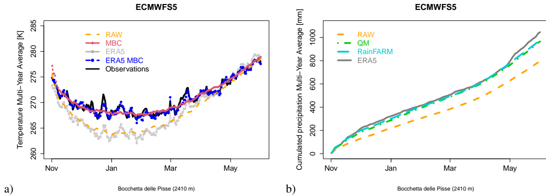
Figure 2. Multi-annual (1995-2015) averages at Bocchetta delle Pisse station (2410 m a.s.l.) of: a) daily air temperature in (gray) the ERA5 reanalysis, (blue) the ERA5 reanalysis bias-corrected with respect to observations with the delta method, (orange) ECMWF55 seasonal forecasts, (red) ECMWF55 seasonal forecast after the bias correction with respect to observation with the delta method, (black) observations; b) accumulated total precipitation in (gray) the ERA5 reanalysis and in ECMWF55 seasonal forecasts with different levels of post-processing: (green) after the bias correction with the quantile mapping with respect to ERA5 method at the monthly scale, (cyan) after the bias correction and the downscaling with the RainFARM method adapted for complex terrains.
