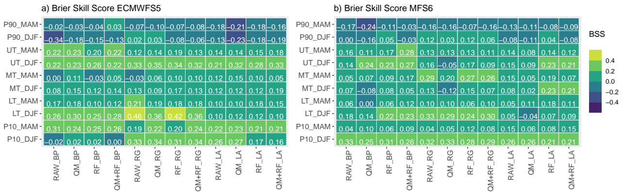
Figure 8. Brier Skill Score of the detrended seasonal (DJF, MAM) snow depth forecasts in the lower (LT), middle (MT), upper (UT) tercile, as well as in the lower (P10) and upper (P90) extreme of the distribution, with respect to the climatological forecasts, using observations at the three stations as a reference, for a) ECMWF55 and b) MFS6 systems. Positive and negative BSSs are highlighted in shades of green and blue, respectively.
