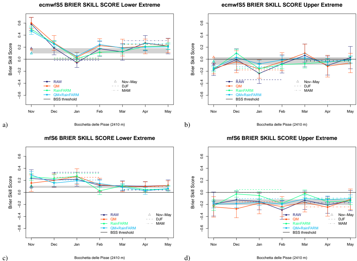
Figure 13. Brier Skill Score for seasonal forecasts of monthly- and seasonally-averaged snow depth (a,c) below the 10^{th} percentile (P10) and (b,d) above the 90^{th} percentile (P90), for (a,b) ECMWF5 and (c,d) MFS6 forcing, starting date November 1^{st} , lead times from 1 to 7 months, for the site of Bocchetta delle Pisse. Colored dots represent the BSS for each month and each experiment, horizontal dashed (dash-dotted) lines represent DJF (MAM) BSS values; the gray filled rectangle and the 4 colored triangles all refer to the seasonal (Nov-May) snow depth forecasts, and they precisely indicate the BSS spread among different experiments and the BSS values for each of the 4 experiments, respectively.
