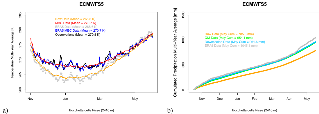
Figure 2. ECMWF5 multi-annual Multi-annual (1995-2016) average of a) daily air temperature daily air temperature b) accumulated total precipitation averages accumulated total precipitation averages at Bocchetta delle Pisse station (2410 m a.s.l.) of: a) daily air temperature in (gray) the ERA5 reanalysis, (blue) the ERA5 reanalysis bias-corrected with respect to observations with the delta method, (orange) ECMWF5 seasonal forecasts, (red) ECMWF5 seasonal forecast after the bias correction with respect to observation with the delta method, (black) observations; b) accumulated total precipitation in (gray) the ERA5 reanalysis and in ECMWF5 seasonal forecast data forecasts with different levels of post-processing: (orange) raw data; (green) after the application of bias correction with the quantile mapping with respect to ERA5 method at the monthly scale; (cyan) after the application of the quantile mapping at monthly scale and the correction of the seasonal average bias; (red) after the correction of and the 6-hourly mean temperature bias. For temperature we report downscaling with the observed climatology derived from the in-situ station (black); this information is not reported RainFARM method adapted for total precipitation since data are affected by large underestimation errors due to snow undercatch complex terrains .
