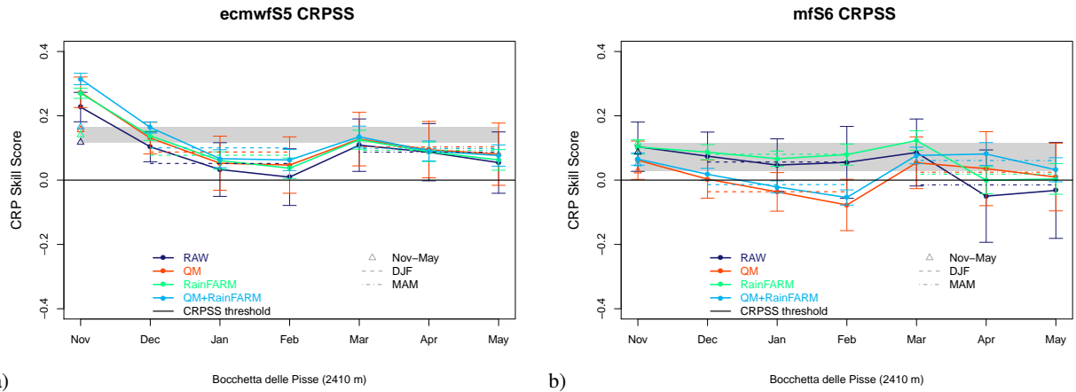
Figure 11. CRPSS for seasonal forecasts of monthly- and seasonally-averaged snow depth for (a) ECMWF5 and (b) MFS6 forcing, starting date November 1 st , lead times from 1 to 7 months, for the site of Bocchetta delle Pisse. Colored dots represent the scores for each month and each experiment; horizontal dashed (dash-dotted) lines represent DJF (MAM) scores; the gray filled rectangle and the 4 colored triangles all refer to the seasonal (Nov-May) snow depth forecasts, and they indicate the score spread among the 4 different experiments and the score for each of the 4 experiments, respectively.
