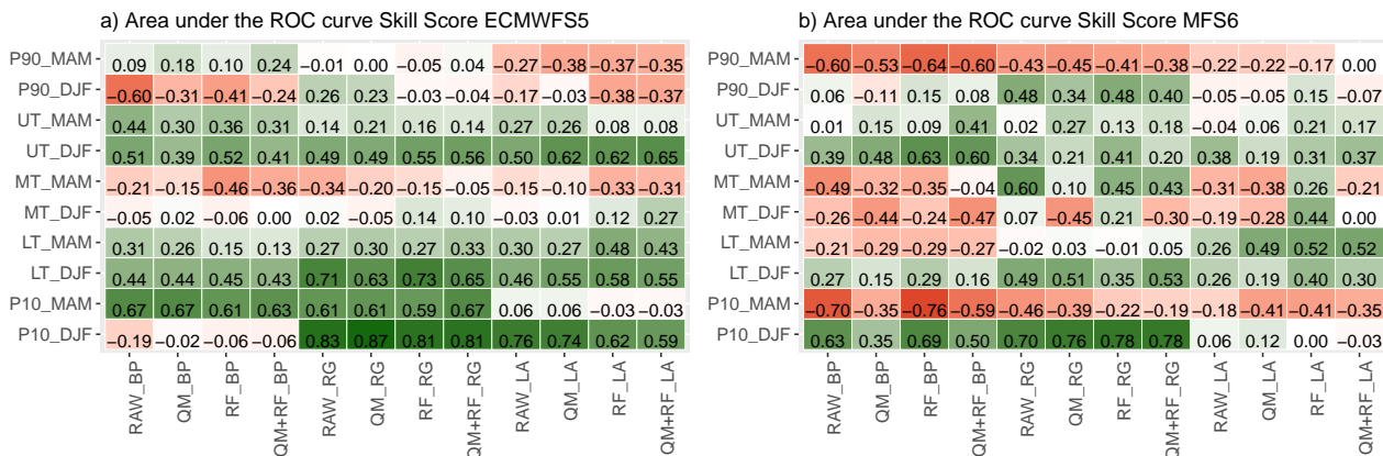
Figure 10. AUCSS of the detrended seasonal (DJF, MAM) snow depth forecasts in the lower (LT), middle (MT), upper (UT) tercile, as well as in the lower (P10) and upper (P90) extreme of the distribution, with respect to the climatological forecasts, using observations at the three stations as a reference, for a) ECMWF55 and b) MFS6 systems. Positive and negative AUCSSs are highlighted in greenish and reddish colors, respectively.
