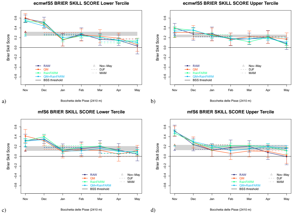
Figure 7. Brier Skill Score for seasonal forecasts of monthly- and seasonally-averaged snow depth in the (a,c) lower and (b,d) upper terciles, for (a,b) ECMWF5 and (c,d) MFS6 forcing, starting date November 1 st , lead times from 1 to 7 months for the site of Bocchetta delle Pisse. Colored dots represent the BSS for each month and each experiment; horizontal dashed (dash-dotted) lines represent DJF (MAM) BSS values; the gray filled rectangle and the 4 colored triangles all refer to the seasonal (Nov-May) values, indicating the BSS spread (min-max) and the single BSS values for the 4 experiments, respectively.
