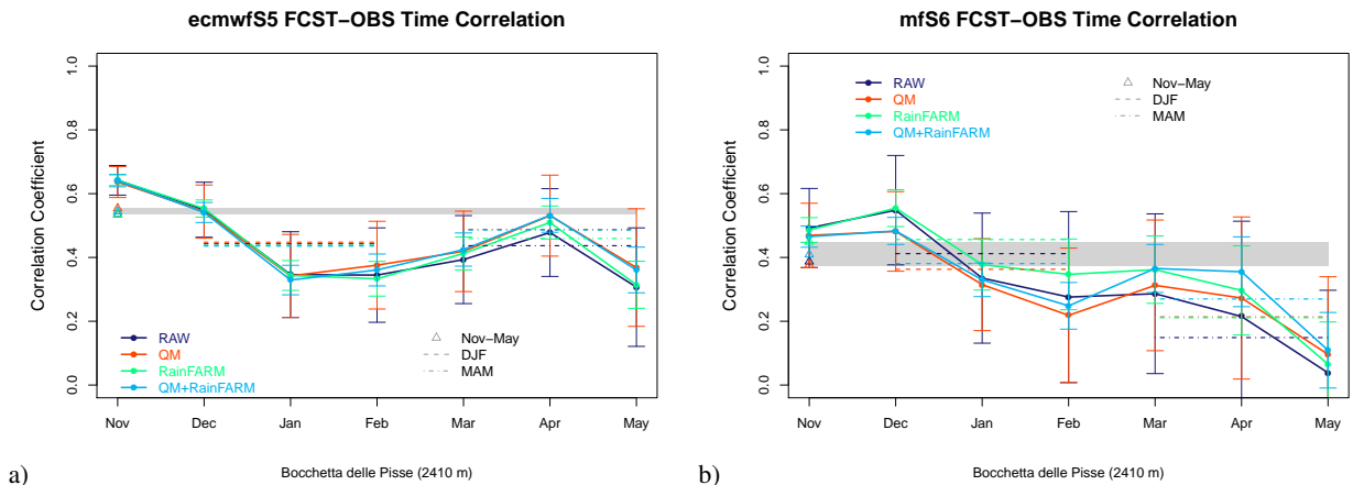
Figure 6. Pearson’s correlation coefficient between forecasts of ensemble-mean monthly-mean snow depth obtained with (a) ECMWF S5 and (b) MFS6 forcing and observations at the site of Bocchetta delle Pisse. Forecasts are initialized on November 1 st and run with a lead time of 7 months. Colored dots represent the correlation for each month and each experiment; horizontal dashed (dash-dotted) lines represent DJF (MAM) values; the gray rectangle and the 4 colored triangles represent seasonally-averaged (Nov-May) values. Error bars represent the 5-95 th percentile range of the distribution of 1000 bootstrap samples as described in Sect. 2.7.
