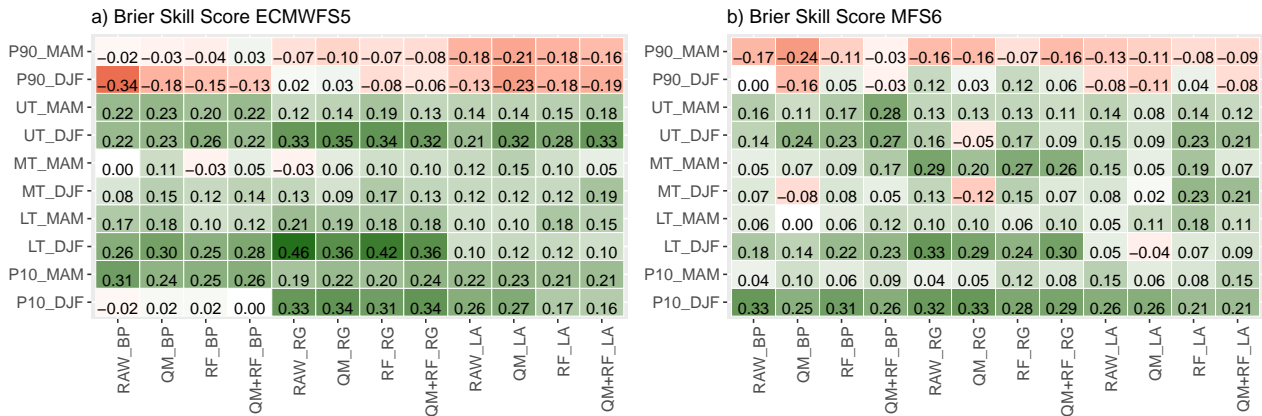
Figure 8. Brier Skill Score of the detrended seasonal (DJF, MAM) snow depth forecasts in the lower (LT), middle (MT), upper (UT) tercile, as well as in the lower (P10) and upper (P90) extreme of the distribution, with respect to the climatological forecasts, using observations at the three stations as a reference, for a) ECMWF55 and b) MFS6 systems. Positive and negative BSSs are highlighted in greenish hues of green and reddish colors red, respectively.
