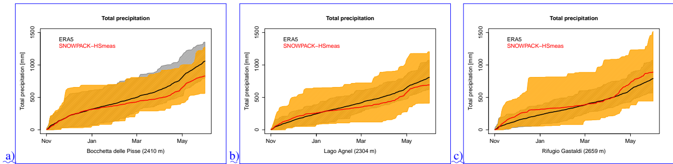
Figure 14. November-May accumulated total precipitation as estimated by (black) the ERA5 reanalysis and (red) the SNOWPACK model driven by the ERA5 forcing (all variables except for total precipitation) and the measured snow depth, for all the three stations.
