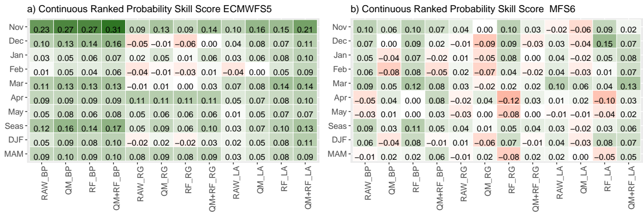
Figure 12. CRPSS of the detrended monthly and seasonal (DJF, MAM) snow depth forecasts with respect to the climatological forecasts, using observations at the three stations as a reference, for a) ECMWF5 and b) MFS6 systems. Positive and negative CRPSSs are highlighted in greenish and reddish colors, respectively.
