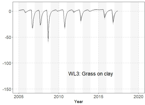
739 Figure 7: Calculated groundwater recharge for all scenarios and sampling locations with indication of vegetation and soil texture.
