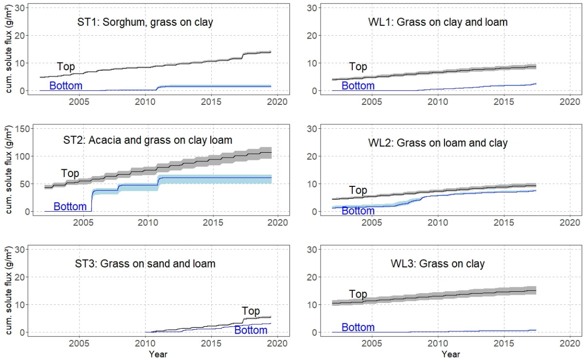
741 Fig. 8: Cumulative solute flux on the upper and lower boundary of the models. The shaded areas represent the standard deviation 742 of 100 randomly selected model runs. Note the different y-axis scales between sites.
