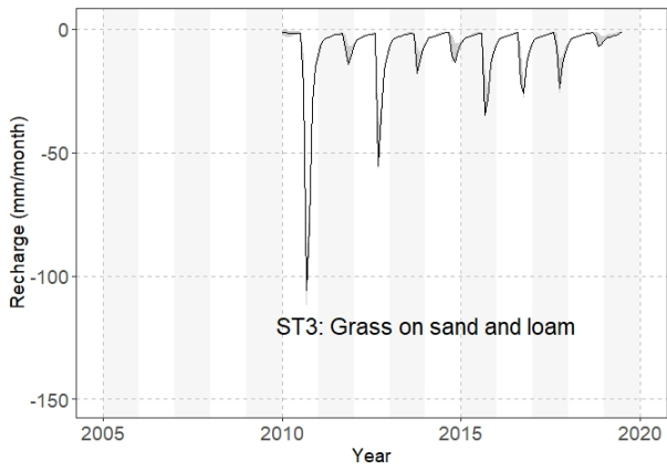
739 Figure 7: Calculated groundwater recharge for all scenarios and sampling locations with indication of vegetation and soil texture.
