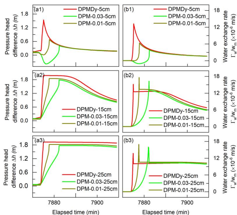
585 586 Fig. 18 Pressure head difference (a1-a3) and water exchange rate (b1-b3) between the two domains at the 5 cm, 15 cm and 587 25 cm depths during the 6 th rainfall event. The positive value of water exchange rate is for the water flowing from the crack 588 to the matrix domain, while the negative value for the opposite direction
