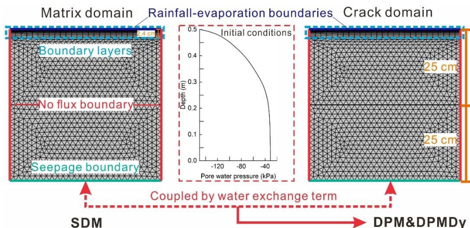
359 Fig. 9 Set-up of the 2-D numerical model for the SDM, DPM and DPMDy 360
