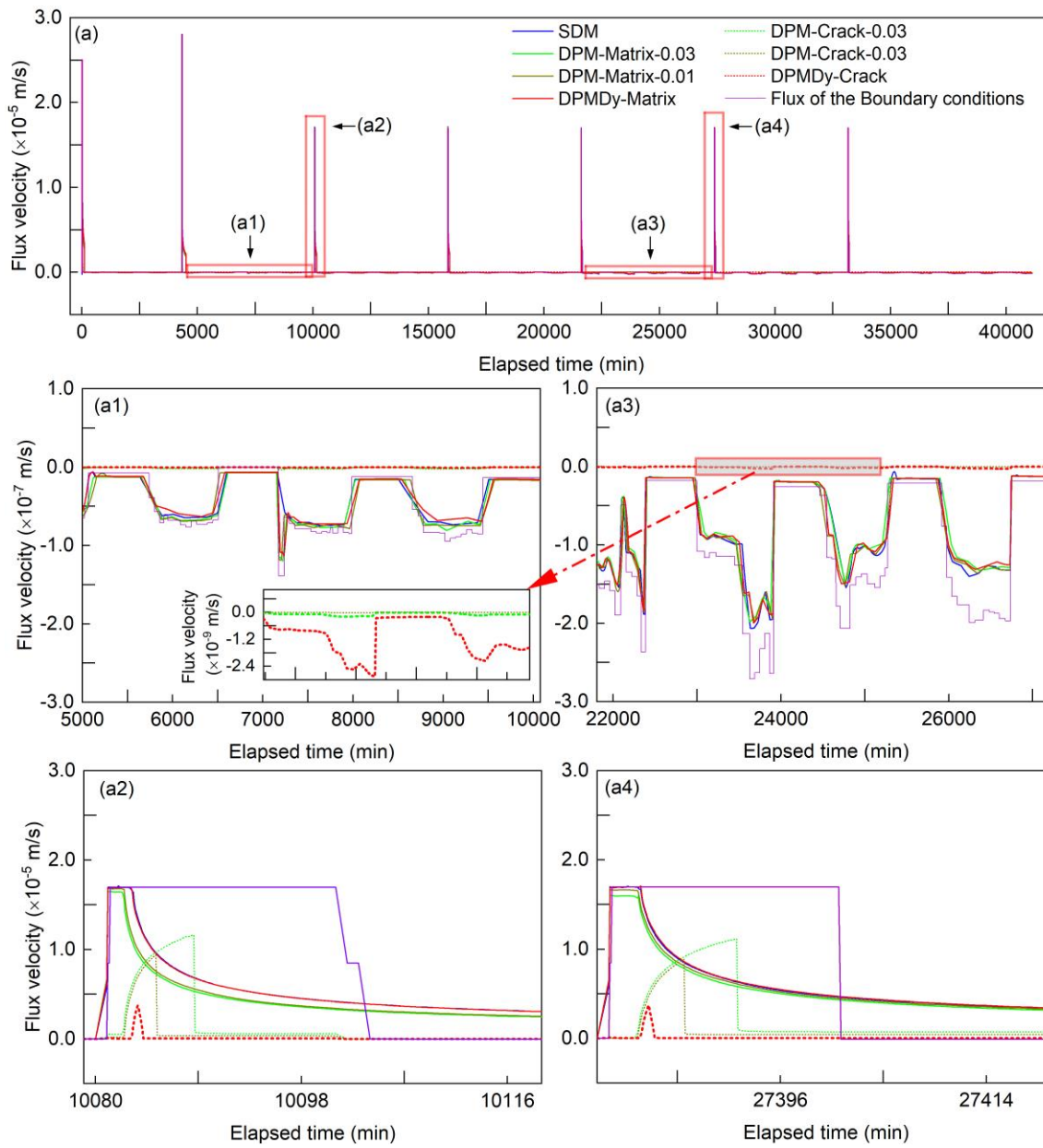
444 Fig. 13 Boundary flow simulated by the SDM, DPM and DPMDy. (a) Flow velocity of the boundary conditions and simulated 445 results; (a1) and (a2) are the enlarged images of the flow velocity during the 2 st drying and 3 rd wetting process, respectively; 446 (a3) and (a4) are the enlarged images of the flow velocity during the 5 th drying and 6 th wetting process, respectively. The 447 positive value is for infiltration and negative for evaporation. 448 449
