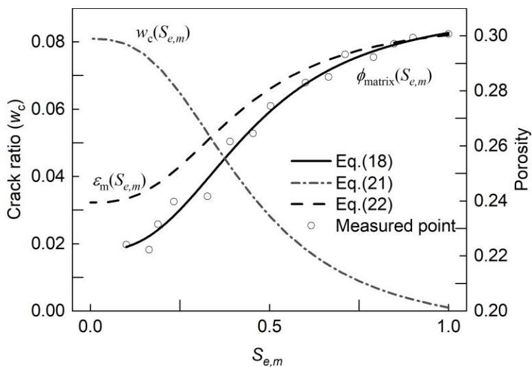
368 Fig. 10 Fitted shrinkage curve (solid line) and modeled porosity variation of matrix (dash line) and crack domains (dash-dot 369 line) 370
