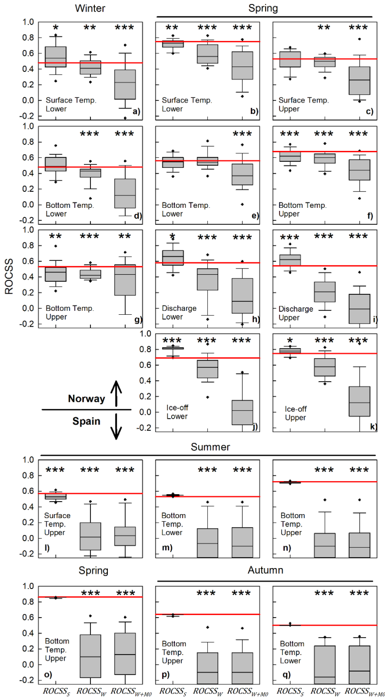
440 Figure 4: Box plots ( n = 25 ) of ROCSS_S , ROCSS_W and ROCSS_{W+M0} from sensitivity analysis runs S-SA (replacing target season SEAS5 data with random data), W-SA (replacing warm-up ERA5 data with random data) and W+M0-SA (replacing warm-up period – ERA5 and first lead month – SEAS5 data with random data) for each window of opportunity at the Norwegian (a–k) and Spanish (l–q) sites. ROCSS_{original} is given by the red line, so ROCSS_S , ROCSS_W and ROCSS_{W+M0} below the red line indicate a loss
