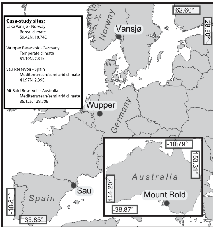
110 Figure 1: Location of the four case studies in Europe and Australia along with climate type and coordinates. Map is modified from Jackson-Blake et al. (2022). Detailed catchment maps are given in Jackson-Blake et al. (2022).
