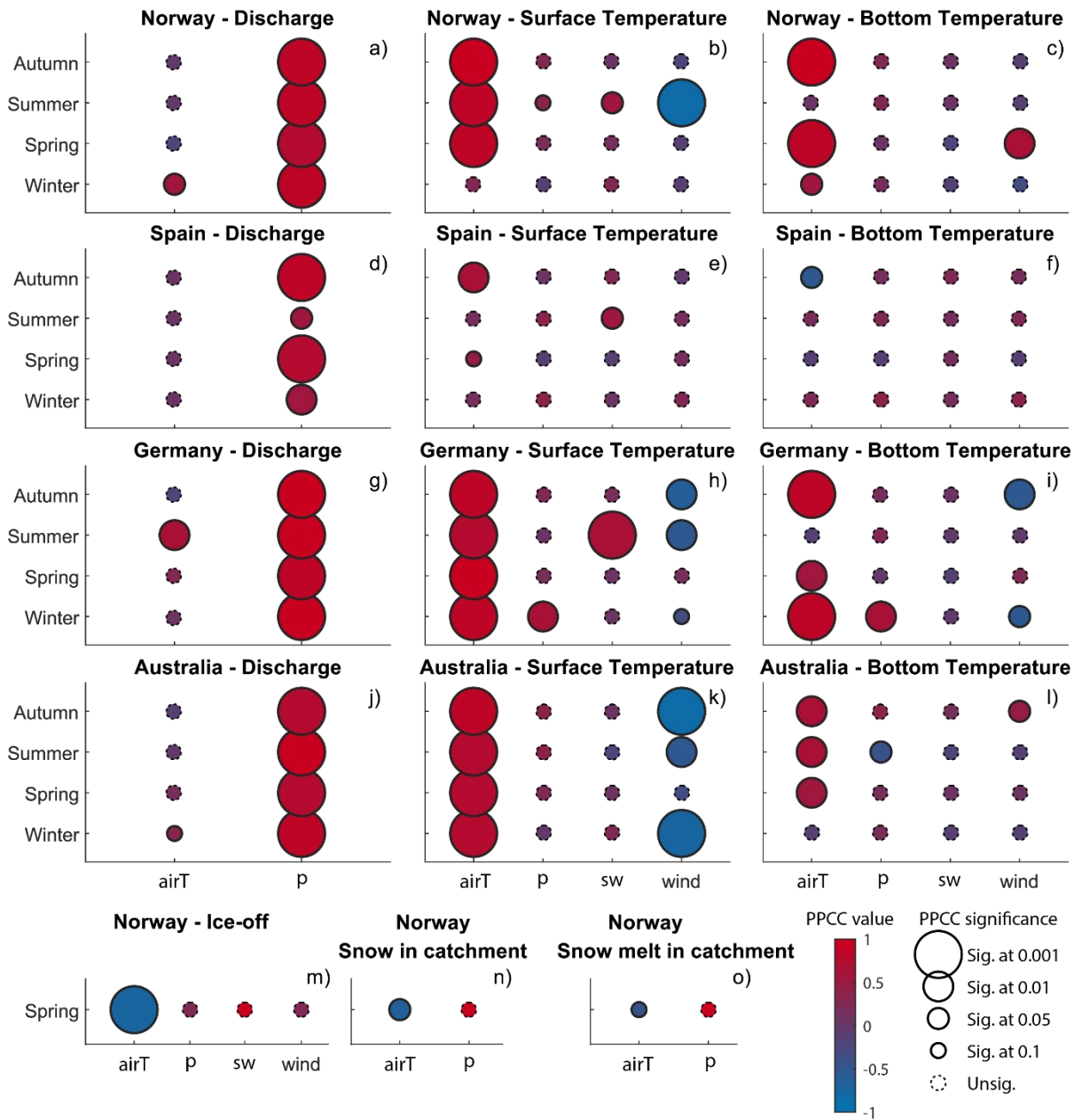
Figure 6: Pearson partial correlation coefficients (PPCC) between Lake_PO seasonal means and seasonal means of selected input variables. Circle color and size represent PPCC value (from -1 to 1) and significance, respectively. Meteorological variable abbreviations: airT, P, wind, cc, hum, and sw stand for surface air temperature, precipitation, wind speed, cloud cover, relative humidity (or dew-point temperature) and short-wave radiation, respectively. Only significance level at 0.1 or below were considered in the interpretation.
