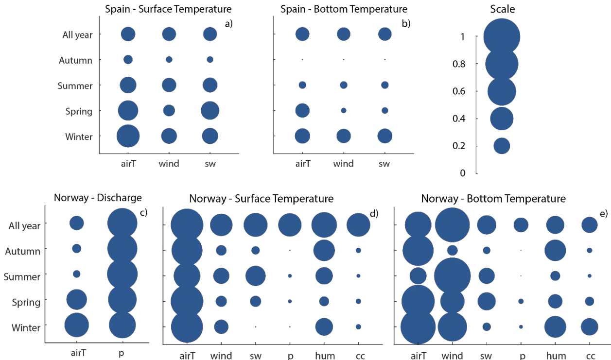
Figure 5: Relative sensitivity expressed as 1 - R^2 of Lake_PO seasonal means to specific input variables estimated following the OAT-SA (see section 2.2.3 and Table 3 in the Methods section for details). Circle size represent relative sensitivity on a scale from 0 to 1. Meteorological variable abbreviations: airT, p, wind, cc, hum, and sw stand for surface air temperature, precipitation, wind speed, cloud cover, relative humidity (or dew-point temperature) and short-wave radiation, respectively. Note that the relatively larger sensitivity of Lake_PO to specific input variables over the whole year can be larger compared to over a given season because of the strong seasonal cyclicity. Note that the OAT-SA was only performed for Sau Reservoir in Spain and Lake Vansjø in Norway.
