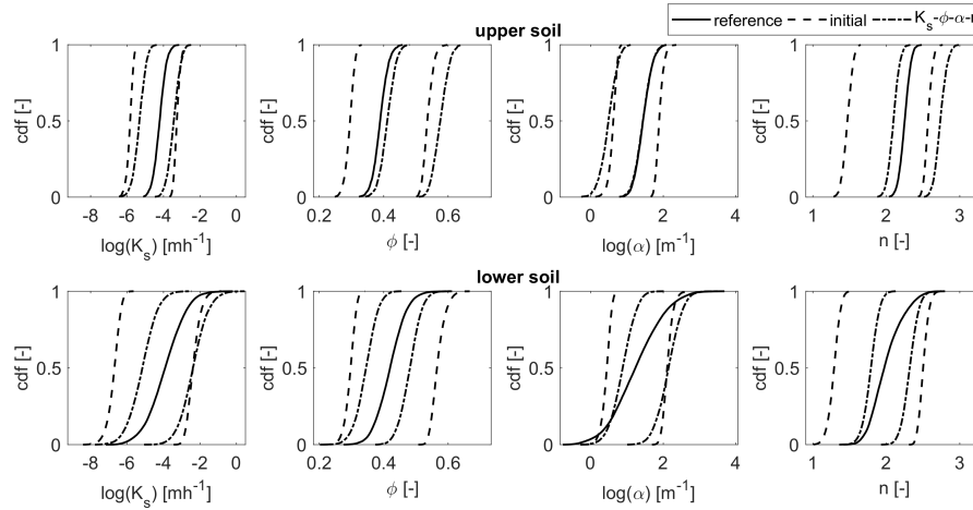
Figure 16. Cumulative density functions (cdf) of the parameter values for the two heterogeneous soil layers. The solid line denotes the cdf of the reference parameter field. For the initial (dashed) and estimated (dash-dotted) ensemble, two lines are plotted indicating the minimum and the maximum values of the ensemble.
