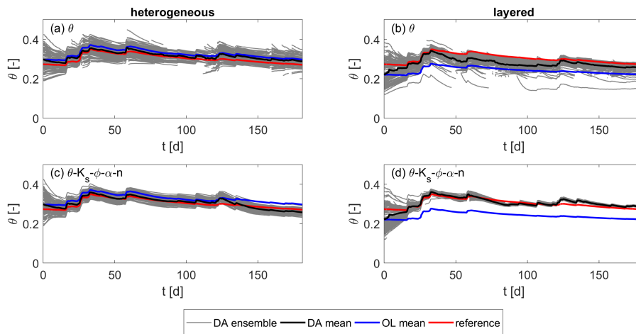
Figure 20. Root zone soil moisture over time for the heterogeneous scenario. Left: results using a heterogeneous structure in the ensemble; right: results using a simplified layered soil in the ensemble. Plots (a) and (b): updates of soil moisture only; plots (c) and (d): joint updates of soil moisture and all parameters.
