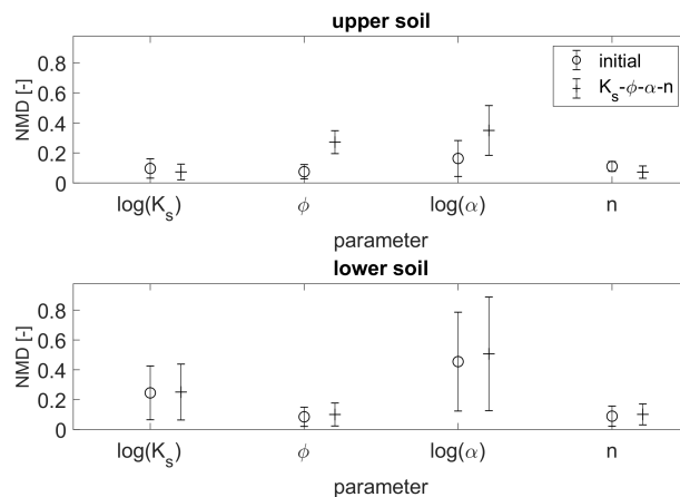
Figure 12. Normalized mean deviation NMD of the estimated parameter fields compared to the reference field for the two soil layers of the heterogeneous scenario. The error bars denote the standard deviation.
