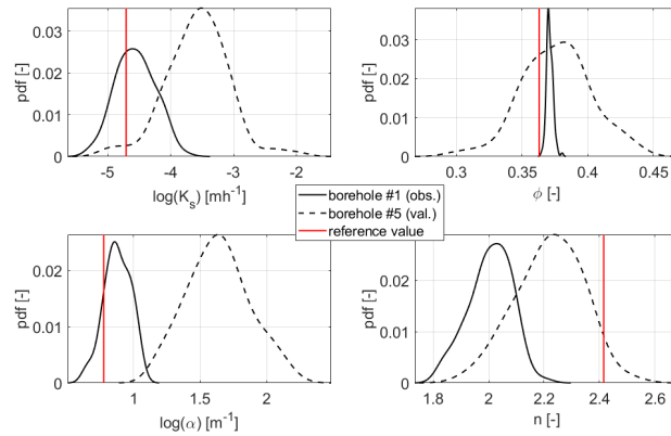
Figure 9. Estimated probability density functions (pdfs) of the four parameters for the heterogeneous scenario at one observation and one validation location and z_2 = 0.75 m below the surface after the last update. The reference values are plotted in red.
