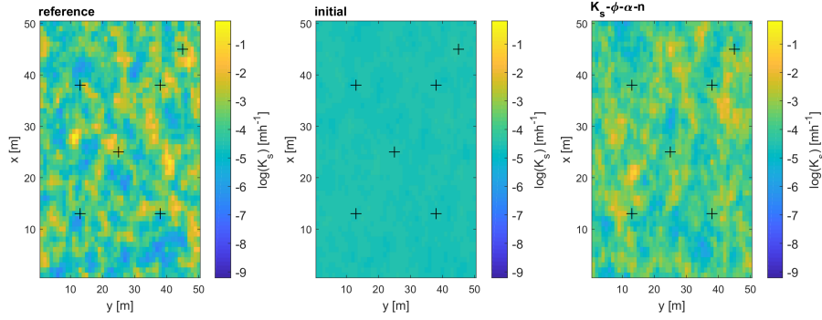
Figure 13. Horizontal cut of the saturated hydraulic conductivity field at z_2 = 0.75\text{m} below the surface for the reference run, the initial ensemble and the estimated field when updating all parameters. The crosses denote the locations of the observation and validation boreholes. Note that the middle and the right field are ensemble means.
