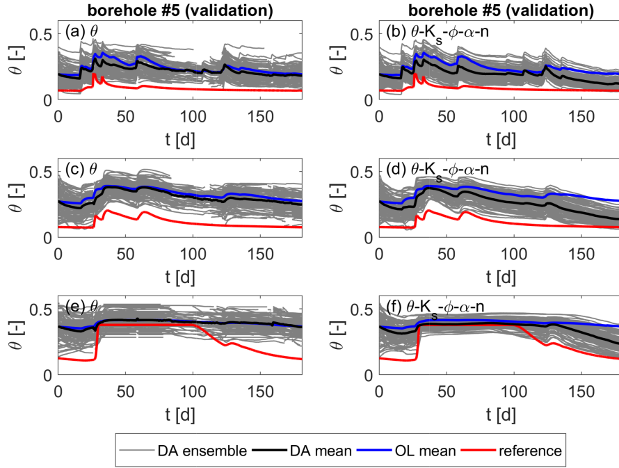
Figure 8. Soil moisture over time for the heterogeneous scenario at one validation location. Values are taken at z_1 = 0.33 m, z_2 = 0.75 m and z_3 = 0.95 m below the surface from top to bottom. Plots (a), (c) and (e): updates of soil moisture only; plots (b), (d) and (f): joint updates of soil moisture and all parameters.
