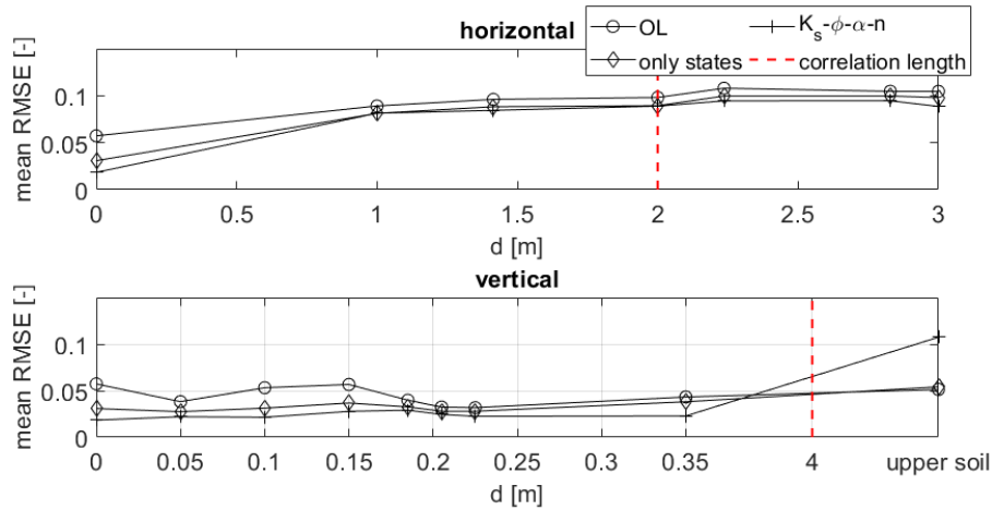
Figure 11. Spatially and temporally averaged RMSE values at horizontal distance d from the observation locations for the heterogeneous scenario. In the upper plot, d is the horizontal distance, in the lower plot the vertical distance. The red line indicates the correlation length of the parameter fields.
