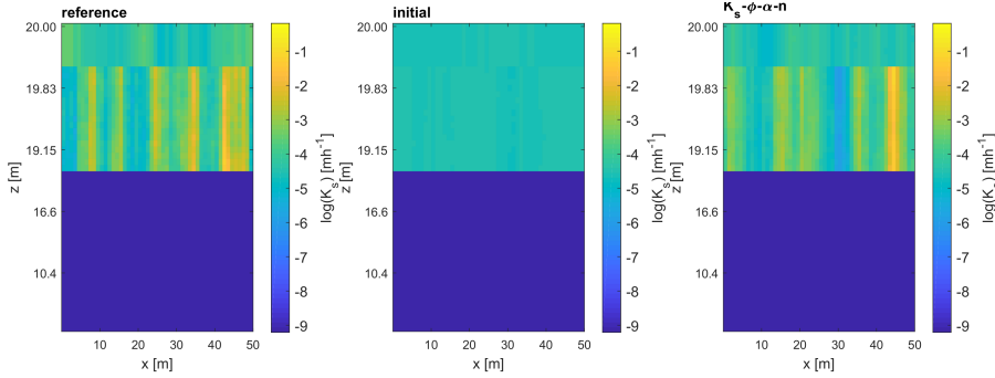
Figure 14. Vertical cut of the saturated hydraulic conductivity field at y = 25\text{m} for the reference run, the initial ensemble and the estimated field when updating all parameters. The z -axis is scaled for better visibility. Note that the middle and the right field are ensemble means.
