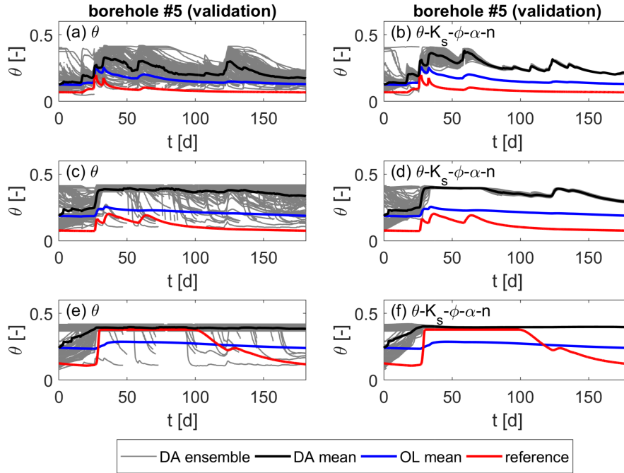
Figure 18. Soil moisture over time for the heterogeneous scenario with a simplified layered soil in the ensemble runs at one validation location. Values are taken at z_1 = 0.33\text{m} , z_2 = 0.75\text{m} and z_3 = 0.95\text{m} below the surface from top to bottom. Plots (a), (c) and (e): updates of soil moisture only; plots (b), (d) and (f): joint updates of soil moisture and all parameters.
