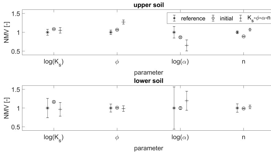
Figure 15. Statistics (mean and standard deviation) of the parameter fields of the two heterogeneous soil layers. All values are normalized by the mean value of the reference field. The statistics of the ensemble runs refer to the estimated parameter field (ensemble mean).
