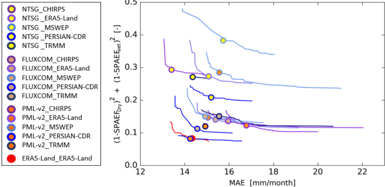
770 Figure 4: Calibration results for the 15 baseline models regarding the two defined objective functions: MAE and SPAEF. The lines represent the Pareto fronts, containing the dominant solutions, and the points of the selected parametrizations with the optimal trade-off between objective functions. Point colors represent the three reference models and line colours represent the five precipitation inputs. The color scheme is consistent with the legends in Figure 2.
