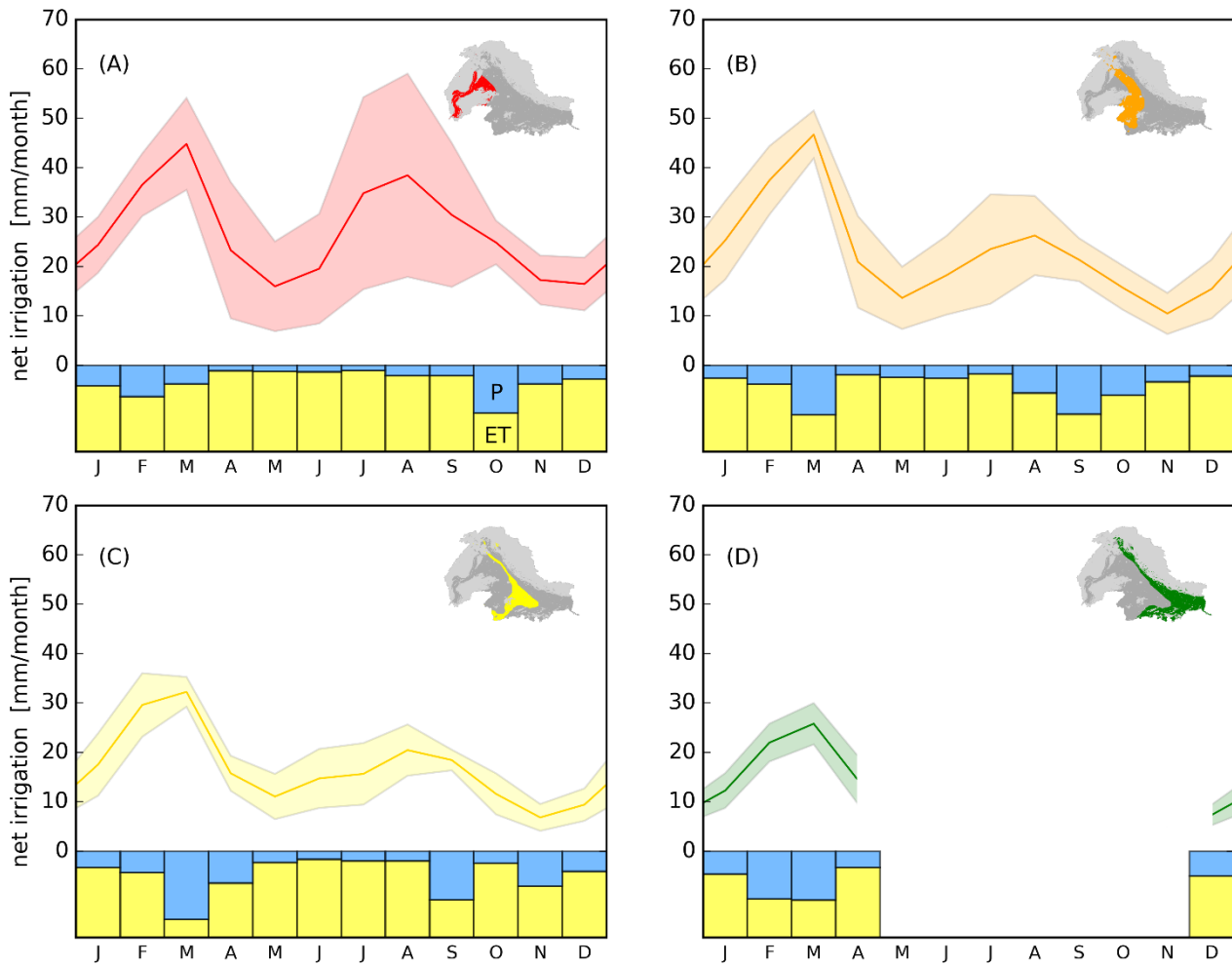
785 Figure 7: Temporal ensemble net irrigation estimates and precision for each climate zone, A: arid, B: semi-arid, C: dry, and D: humid. The solid line indicates the mean monthly net irrigation whereas the shaded envelope the precision as \pm 1 standard deviation. Lower bar charts illustrate results from the variance decomposition analysis and show to what degree evapotranspiration (ET, yellow) and precipitation uncertainty (P, blue) explain the ensemble variance.
