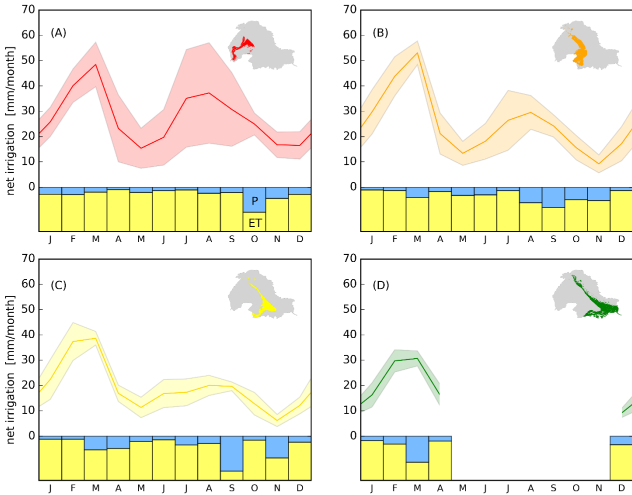
795 Figure 7: Temporal ensemble net irrigation estimates and precision for each climate zone, A: arid, B: semi-arid, C: dry and D: humid. The solid line indicates the mean monthly net irrigation whereas the shaded envelope the precision as \pm 1 standard deviation. Lower bar charts illustrate results from the variance decomposition analysis and show to what degree evapotranspiration (ET, yellow) and precipitation uncertainty (P, blue) explain the ensemble variance.
