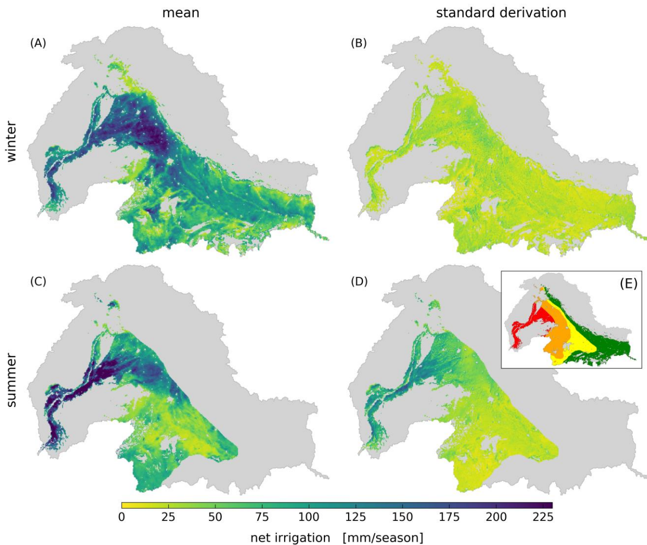
790 Figure 6: Mean ensemble net irrigation estimates (left panel) and ensemble standard deviation (right panel) for dry period (upper panel) and wet period (lower panel). E: Dryland classification by the Joint Research Center of the European Commission (Spinoni, 2015), red: arid, orange: semi-arid, yellow: dry, green: humid.
