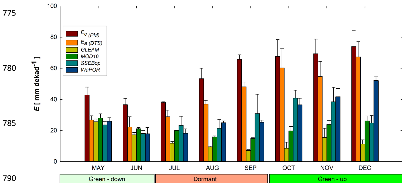
790 Figure 10. Bar graphs with standard deviation error bars comparing dekadal averages of E_a (DTS) and E_c (PM) with satellite-based evaporation estimates from May – December 2021. The WaPOR shows a similar trend to both E_a (DTS) and E_c (PM).
