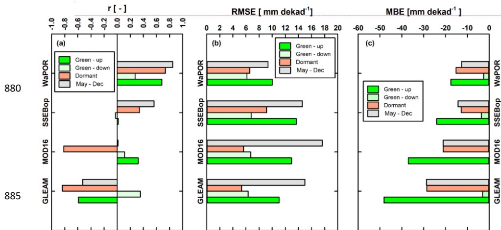
880 Figure 12: (a) statistics of the correlation of E_{a(DTS)} with satellite-based estimates and (b, c) 885 statistics of uncertainty in satellite-based evaporation estimates with reference to E_{a(DTS)} for each 890 phenophase and for the entire study period May-December, 2021.
