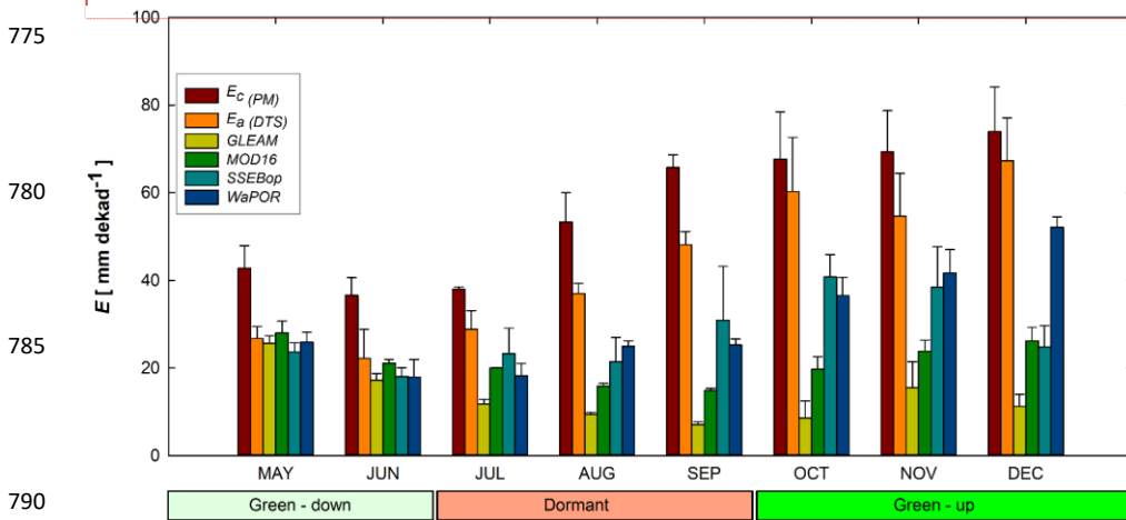
790 Figure 10. Bar graphs with standard deviation error bars comparing dekadal averages of E_a (DTS) and E_c (PM) with satellite-based evaporation estimates from May – December 2021. The WaPOR shows a similar trend to both E_a (DTS) and E_c (PM).
