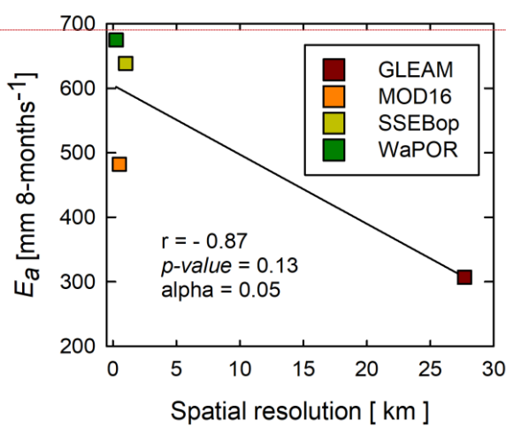
Figure 13. Point scale-based correlation of spatial resolution with estimates of actual evaporation of satellite-based evaporation estimates.
