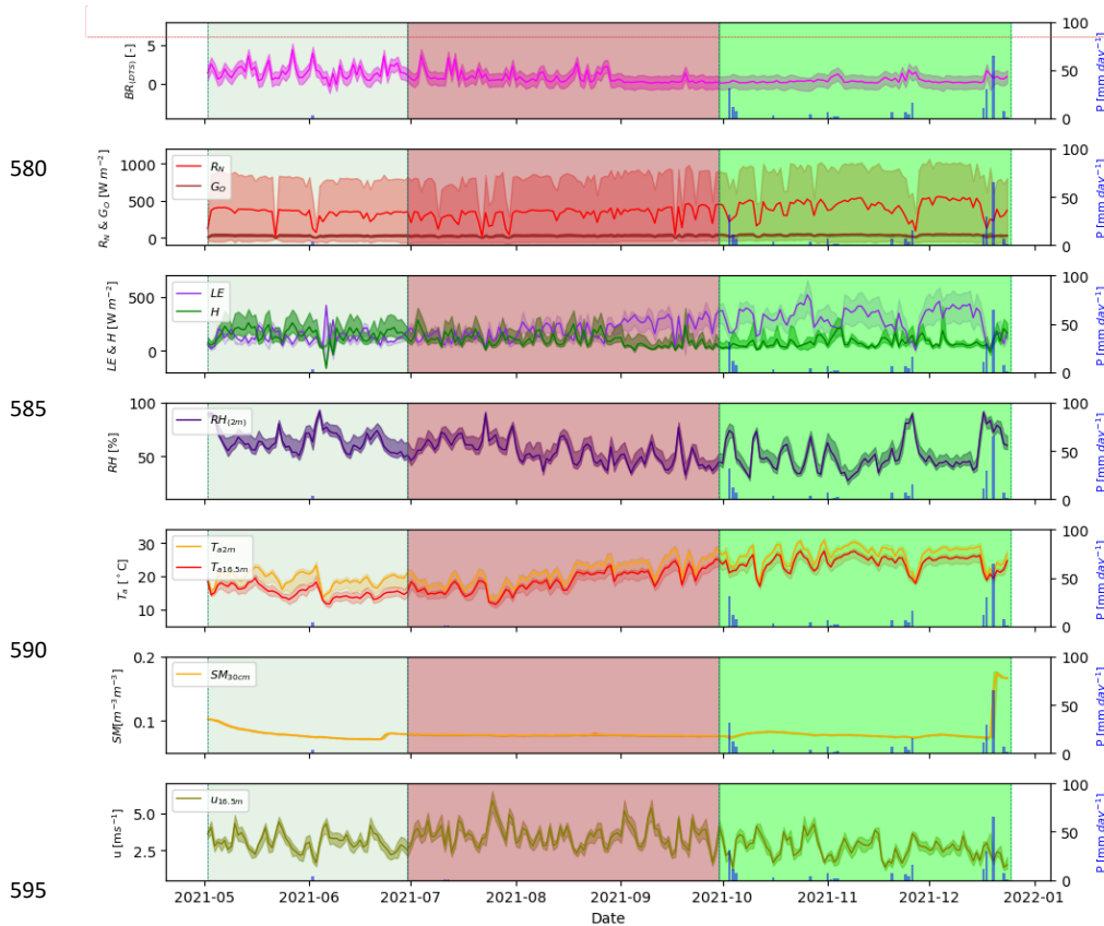
580 585 590 595 Figure 5. Daily meteorological conditions at the Mpika study site in the Luangwa Basin for the period May 2021 – December 2021. Shaded area for variables is the standard deviation. Shaded area May-June is the canopy Green-down phenophase, July-September is the dormant phenophase and October-December is the Green-up phenophase.
