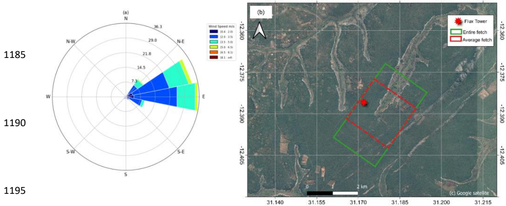
Figure A1. Analysis of the wind direction and wind speed using the wind rose (a) and the extent of the fetch for the DTS observations (b) based on the wind rose results.
