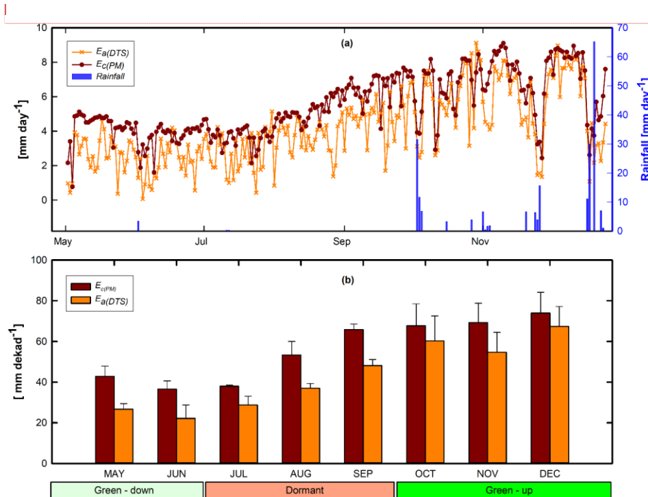
Figure 7. (a) May – December 2021 daily (6AM - 6PM) estimates of evaporation E_a(DTS) using the BR-DTS and E_c(PM) using the PM . (b) Comparison of dekadal evaporation estimates between E_a(DTS) estimates and E_c(PM) ( E_c = K_c \cdot E_o ). The E_a(DTS) and E_c(PM) show good agreement in both dry and rainy seasons as well as across canopy phenophases. Overall, at dekadal scale the E_c(PM) is relatively higher than E_a(DTS) (b). Phenophases classification: May-June is the green-down phenophase, July-September is the Dormant phenophase and October-December is the green-up phenophase.
