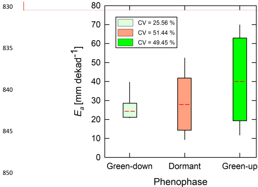
Figure 11: Box plots showing variations in satellite-based evaporation estimates at dekadal scale across phenophases. Dotted red line is the mean for each phenophase. Coefficients of variation (CV) were largest during the dormant and green-up phenophases.
