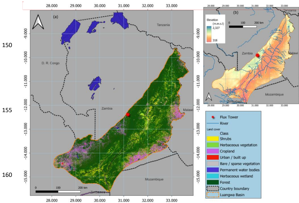
165 Figure 1. Land cover (a) and elevation (b) characterization in the Luangwa Basin and at the study site in Mpika. The ASTER Digital elevation model was used to depict elevation while the 2019 Copernicus Land cover for Africa was used for land cover characterization.
