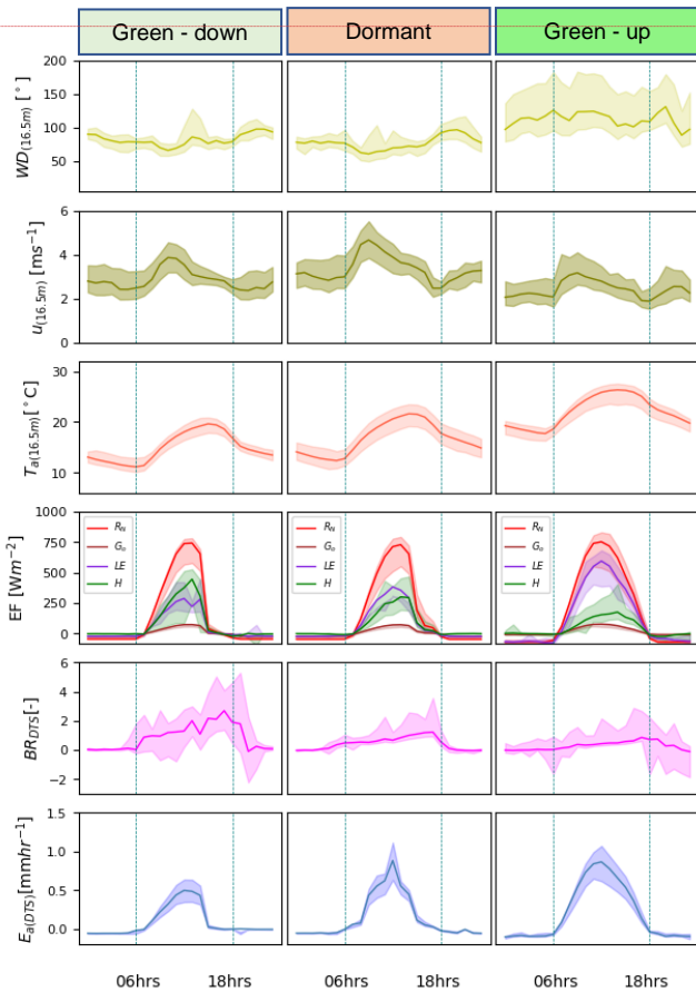
640 Figure 6. Forest canopy phenophase based hourly averages of wind direction ( WD ), wind speed ( u ), Energy flux ( EF ) (net radiation ( R_N ), ground heat flux ( G_o ), latent heat flux ( LE ) and sensible heat flux ( H )), Bowen ratio ( BR_{DTS} ) and actual evaporation ( E_{a(DTS)} ). Shaded area is the standard deviation.
