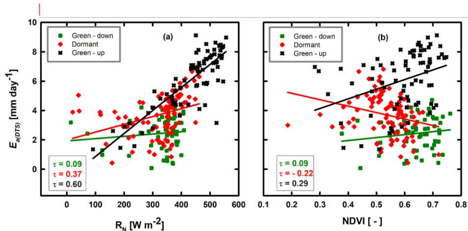
Figure 9. Kendall correlation of E_{a(DTS)} with R_N and NDVI in the Green-down, Dormant and Green-up phenophases of the Miombo forest at Mpika site, Zambia.
