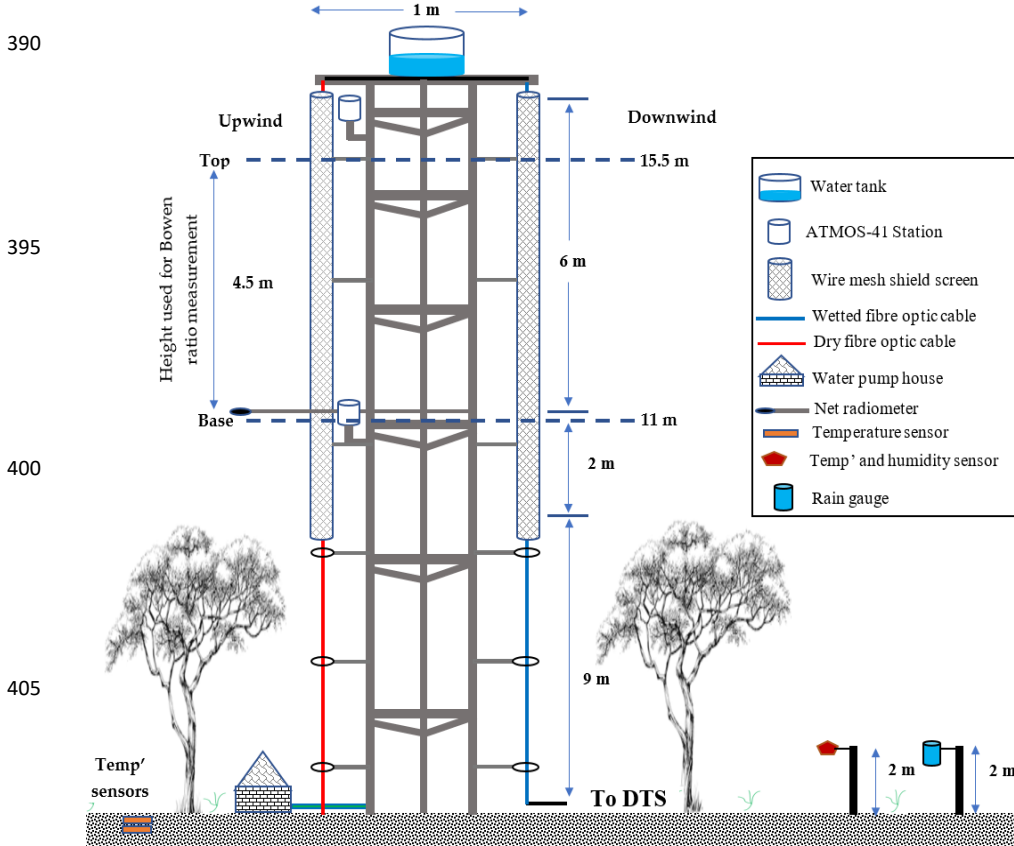
410 Figure 2. Schematic drawing (not to scale) of the field set-up of the observation tower at the study site in Mpika, Zambia.
