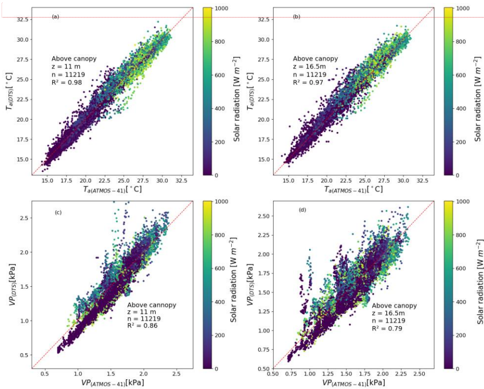
560 Figure 4. Comparison of DTS temperature ( T_{a(DTS)} ) and actual vapour ( VP_{(DTS)} ) measurements with the ATMOS-41 ( T_{a(ATMOS-41)} and VP_{(ATMOS-41)} ) measurements at 11 m and 16.5 m above the forest canopy.
