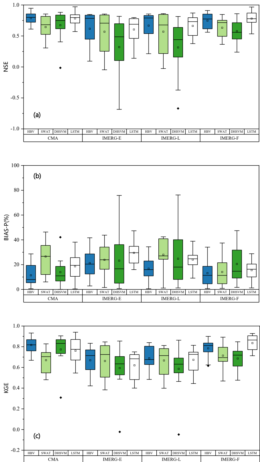
480 Fig. 9. The (a) NSE, (b) BIAS-P and (c) KGE of flood events simulation forced by CMA, IMERG-E, IMERG-L and IMERG-F using calibration strategies II. The box plots show the 25th, 50th, and 75th percentiles, and the mean value is given and shown by a square.
