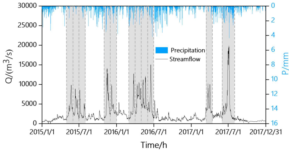
170 Fig. 2. Time series of observed hourly streamflow in Xiangtan station and basin-average precipitation from CMA, with eleven selected flood events covered by shaded areas.
