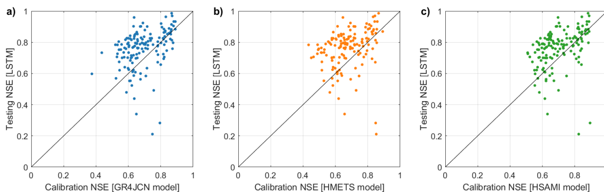
Figure 3: Performance of hydrological models calibrated at each of the 148 study basins individually against the performance of the LSTM model in leave-one-out cross-validation (LOOCV) where the basin in question is not included in the set of N-1 basins used to train the LSTM. The hydrological models' performance displayed is hence a calibration performance while the LSTM performance is the testing performance (on ungauged locations). The models are evaluated using all available streamflow data in the period 1979 to 2018. The results are compared between LSTM models (y-axis) and three hydrological models (x-axis), i.e., a) GR4JCN, b) HMETS and c) HSAMI.
