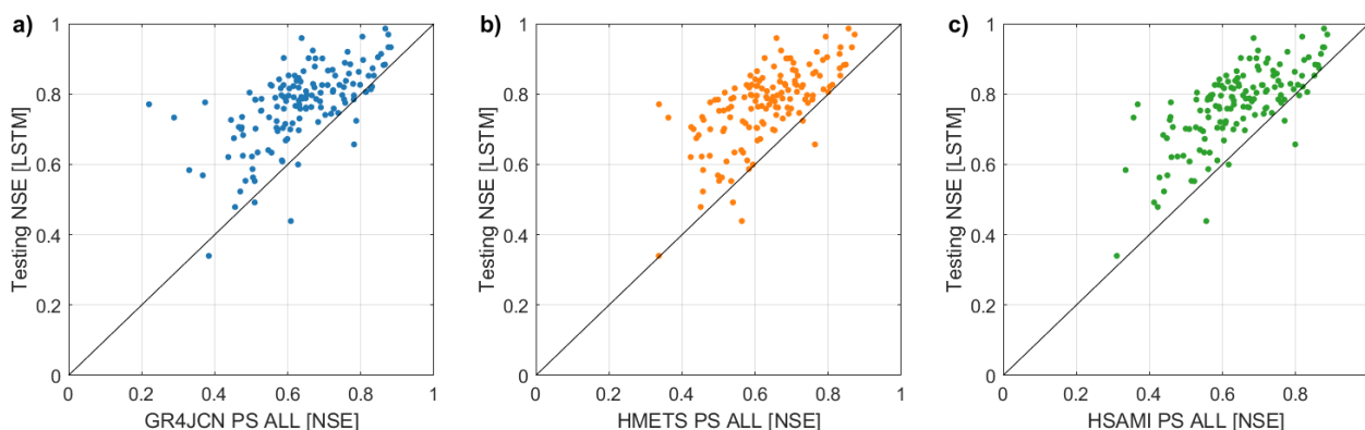
Figure 7: Hydrological model regionalization NSE compared against the LSTM model in testing for a) GR4JCN, b) HMETS and c) HSAMI. The regionalization method with the best overall median for each hydrological model was selected for the comparison (here PS ALL for all three models). One point per catchment is displayed in each panel, for a total of 148 points.
