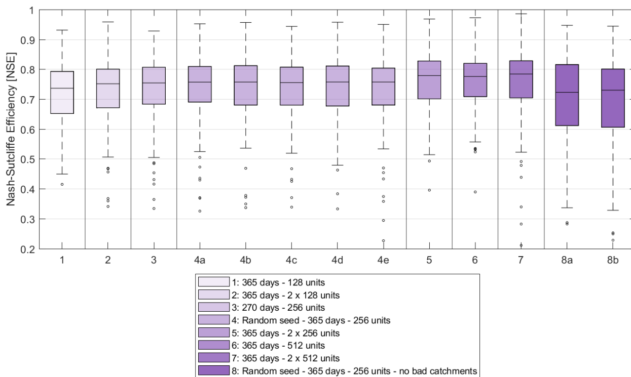
Figure 8: Distribution of LSTM performance in leave-one-out cross-validation (LOOCV) over the 148 basins using different hyperparameters. The distribution used in this study is model #7. Details about the hyperparameter variations can be found in Table 2.
