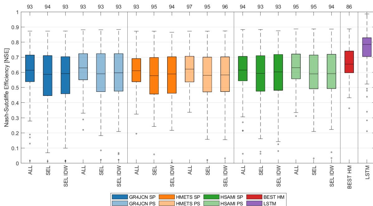
735 Figure 4: Boxplots of the regionalization results for GR4JCN (blue), HMETS (orange) and HSAMI (green) using the spatial proximity (SP; dark) and physical similarity (PS; light) regionalization methods on all (ALL) or a selection (SEL) of catchments based on performance and application of inverse distance weighting (IDW) on the 148 catchments. All hydrological model-based regionalization methods implemented a multi-donor approach using five donors. Two additional boxplots present the best value from all hydrological model approaches (out of 18) for each catchment (BEST HM; red) and for the LSTM model (purple). The 740 results displayed for the LSTM are the same results as they were used in Fig. 3. The models are evaluated on all available streamflow data available during the period 1979 to 2018. The box of each boxplot indicates the 25th and 75th percentile; the center line is the median; The whiskers represent the maximum and minimum non-outlier values, which are set at 1.5 times the interquartile range and covers 99.3% of the distribution. Values above each boxplot represent the percentage of basins for which the LSTM model performs better than the hydrology-model based regionalization method.
