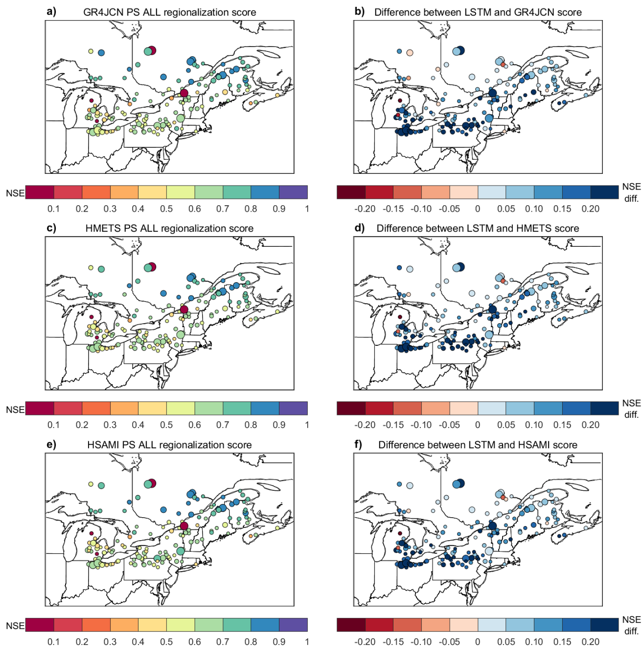
750 Figure 6: Spatial distribution of regionalization skill of the hydrological models (a, c, e) and difference between the LSTM testing and hydrological model regionalization skill (b, d, f) for the three models GR4JCN (a, b), HMETS (c, d) and HSAMI (e, f). Circle sizes represent the relative sizes of the catchments and are placed at the catchment centers. The regionalization method with the best overall median for each hydrological model was selected for the comparison (here PS ALL for all three models). Blue colors in panels (b, d, f) indicate the LSTM is outperforming the hydrological model, while red colors indicate the opposite.
