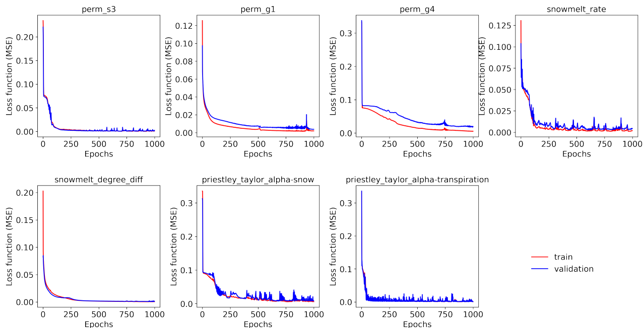
Figure 7. The mean squares error (MSE) loss functions of the training and validation data over 1000 epochs for the seven parameters, each of which is estimated by a knowledge-guided inverse mapping (mi-q-only-3yrs) by using the corresponding sensitive streamflow during the model calibration period (i.e., water years 2017 through 2019).
