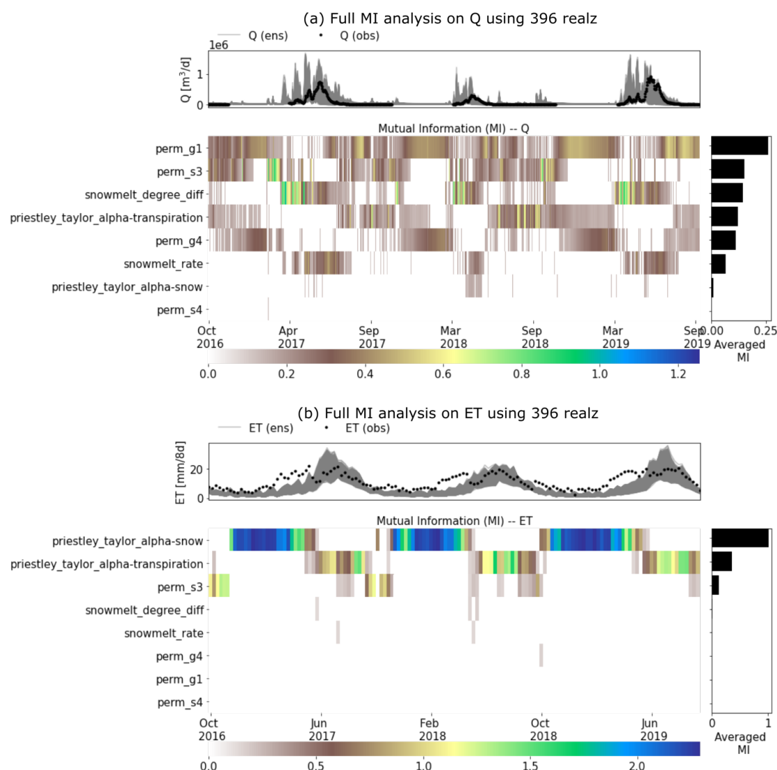
Figure 5. A full MI-based sensitivity analysis using 396 realizations of the Advanced Terrestrial Simulator (ATS) on (a) the discharge ( Q ) and (b) evapotranspiration ( ET ). The top panel of each subplot shows the ATS ensemble (gray) and the corresponding observations (black).
