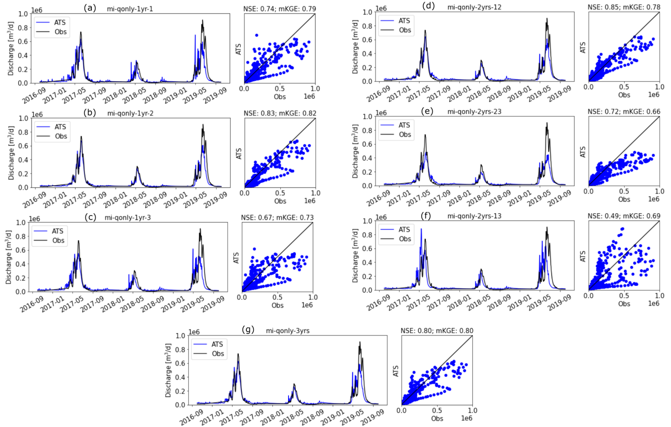
Figure 9. Forward runs of the Advanced Terrestrial Simulator (ATS) based on the estimated parameters from knowledge-informed inverse mappings using multiple years of discharge (Q) in Table 1. (a-c) are the simulated discharge (Q) using each of the three water years to calibrate (i.e., mi-qonly-1yr-1, mi-qonly-1yr-2, and mi-qonly-1yr-3). (d-f) are the simulated discharge (Q) using two of the three water years to calibrate (i.e., mi-qonly-2yrs-12, mi-qonly-2yrs-23, and mi-qonly-2yrs-13). (g) is the simulated discharge using all three years to calibrate (i.e., mi-qonly-3yrs).
