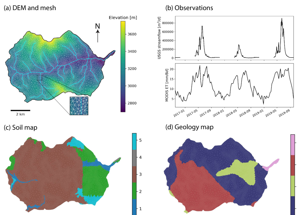
Figure 1. The Coal Creek watershed and the setup of the Advanced Terrestrial Simulator (ATS). (a) the river network, the digital elevation model (DEM), and the surface mesh of the watershed. (b) the time series of USGS streamflow observations (station number 09111250) at the watershed outlet and the Moderate Resolution Imaging Spectroradiometer (MODIS) 8-day composite evapotranspiration (ET) averaged across the watershed. (c) and (d) the delineated soil and geological layers, respectively.
