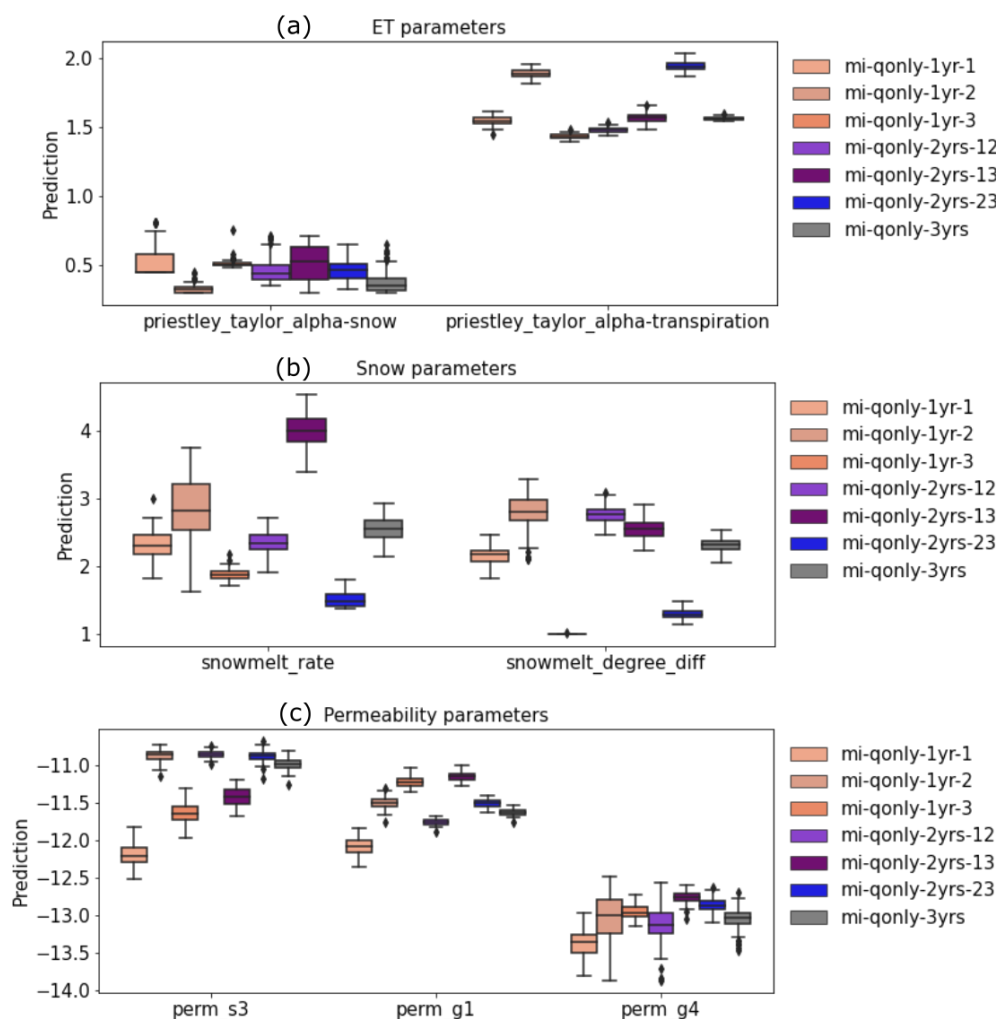
Figure 11. Box plots of ensemble parameters estimated knowledge-informed inverse mappings of multiple years of discharge (Q) using 100 realizations of noisy discharge observations with 5% observation error, categorized into (a) evapotranspiration (ET) parameters; (b) snow parameters; and (c) permeability parameters.
