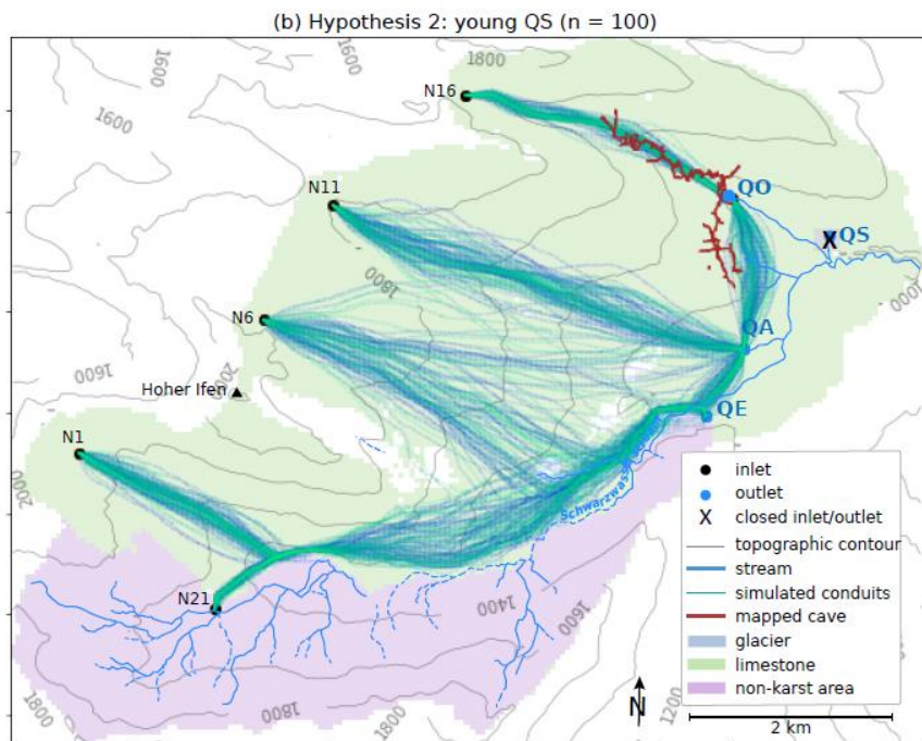
285 Figure 4: Probability maps for 100 simulations under each hypothesis, compared to the observed cave map. (a) Hypothesis 1 yielded no networks matching the mapped cave system. (b) Hypothesis 2 yielded networks matching the orientation of the inactive cave network, located slightly to the east of the mapped network. This suggests that hypothesis 2 is less probable than hypothesis 1.
