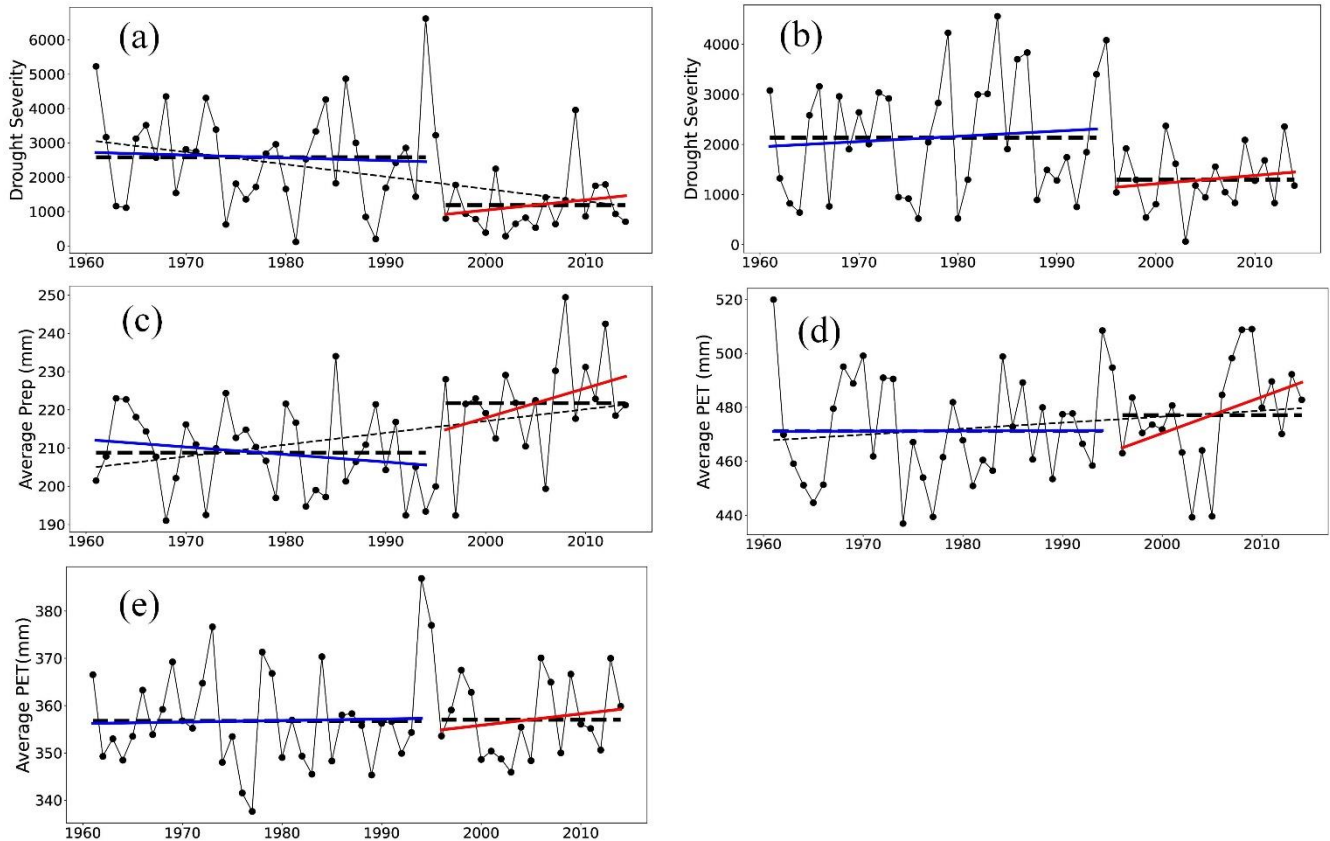
Figure 9. Variations of the total annual SM drought severity for (a) GLDAS and (b) ERA5, (c) yearly average precipitation (Prep) of CMA, and potential evapotranspiration (PET) of (d) GLDAS and (e) ERA5 over summer periods (May–September)
