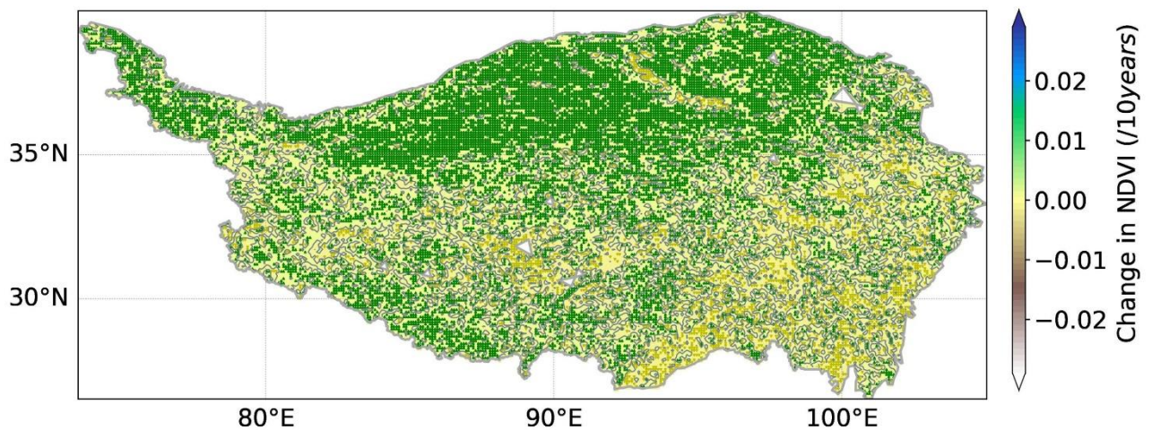
Figure 11. Variations of NDVI over summer periods of May–September from 1982 to 2015 for the Tibetan Plateau. The greed/brown \Delta/\nabla denotes the significant ( p < 0.05 ) increasing/decreasing trends.
