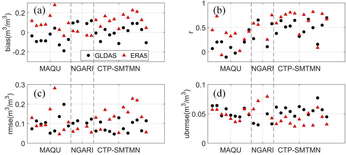
Figure 3. The (a) bias, (b) Pearson correlation coefficient ( r ), (c) root mean square error (rmse) and (d) unbiased rmse (ubrmse) for GLDAS and ERA5 soil moisture in summer periods of May-September over 2008-2014 based on the ISMN station measurements from the MAQU, NGARI, and CTP-SMTMN observation network.
