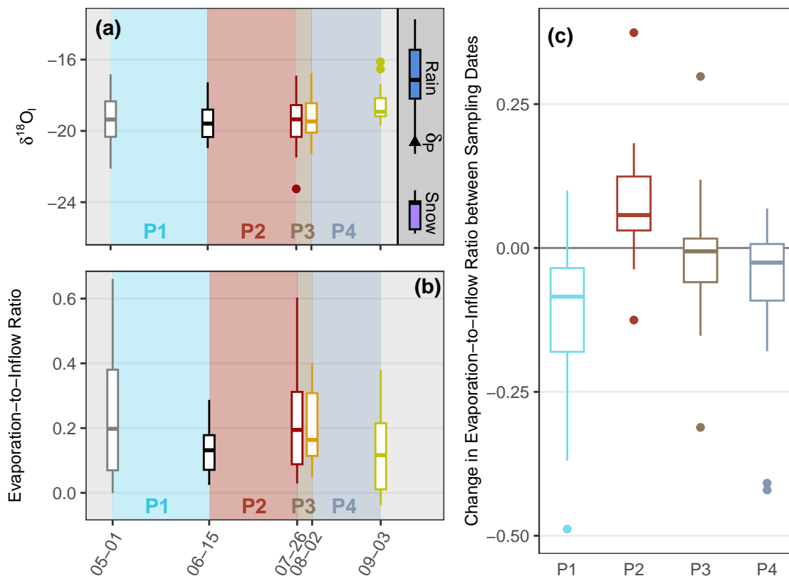
Figure 4. (a) The distribution of \delta^{18}\text{O}_\text{l} for each sampling date with rain and snow isotope compositions for reference. (b) The distribution of E/I values at all lakes across the five sampling dates. (c) The lake-specific change in E/I between the sampling dates was calculated as \Delta[E/I] = [E/I]_{t_2}^{Ln} - [E/I]_{t_1}^{Ln} , where Ln represents a specific lake, and t represents a sampling date.
