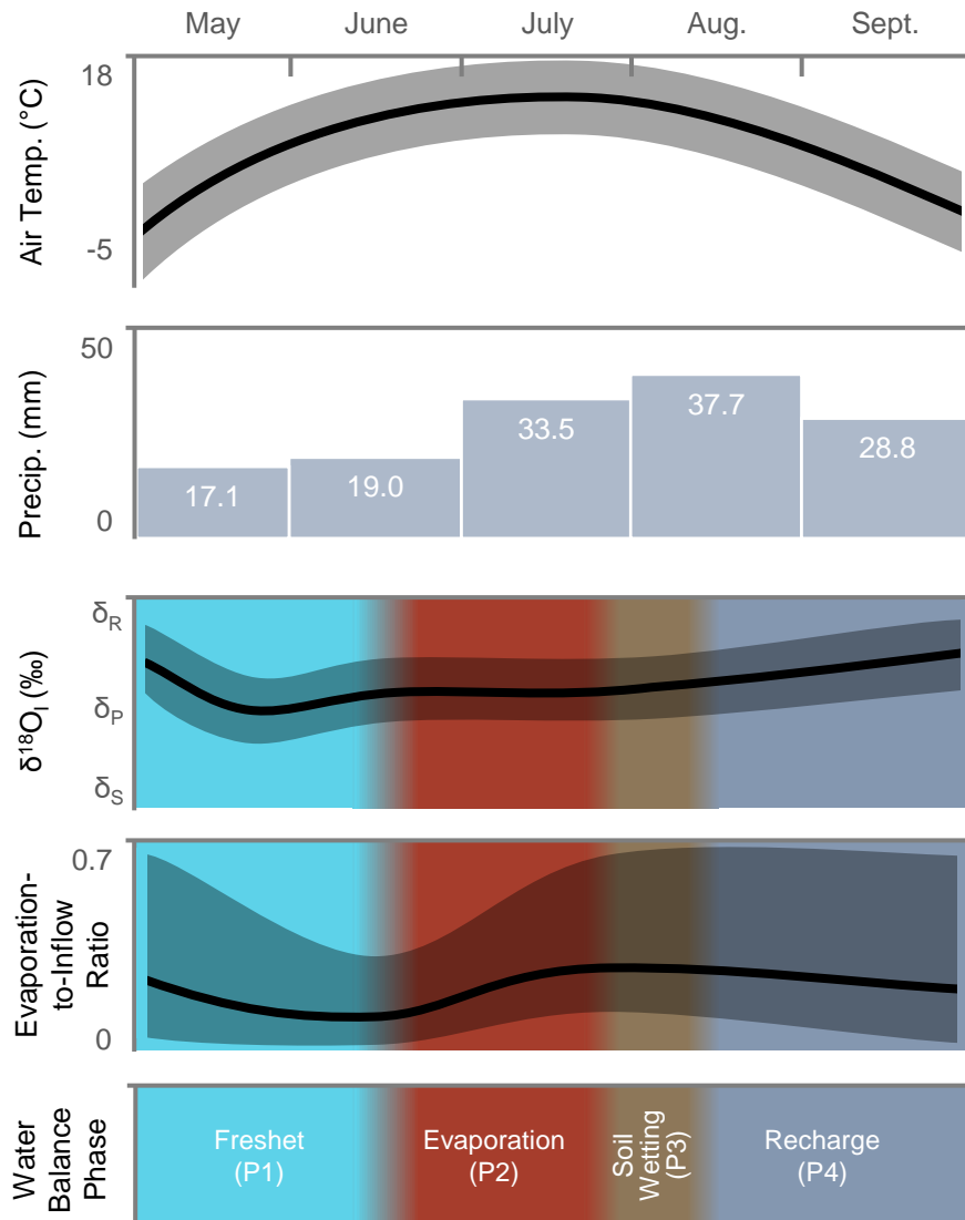
Figure 6. A simplified conceptual diagram showing the connections between comparing meteorological conditions and the response of \delta^{18}\text{O}_I and E/I used to designate water balance phases. Air temperature and precipitation data represent average values from 1980-2020 ( Environment and Climate Change Canada, 2019 ). Shaded areas around the \delta^{18}\text{O}_I and E/I lines represent the potential variability caused by lake and watershed attributes or meteorological conditions.
