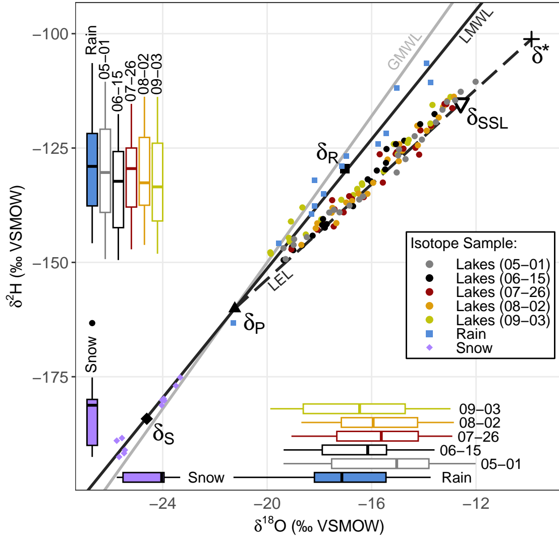
Figure 3. Isotope values and their respective ranges for all lake and precipitation samples are, with their respective ranges along each axis illustrated by boxplots, plotted in \delta^{18}\text{O} - \delta^2\text{H} space, as deviations per mil from Vienna Standard Mean Ocean Water (VSMOW). The Local Meteoric Water Line (LMWL, black solid line, \delta^2\text{H} = 7.1 * \delta^{18}\text{O} - 10.0 ) is calculated as a regression through snow samples collected throughout the study region and rain samples collected from Inuvik in 2018 ( n = 24 ). The average isotope composition of end-of-winter snow samples ( \delta_s ), rainfall samples ( \delta_r ), and the average of \delta_s and \delta_r ( \delta_p ) are labelled along the LMWL. The Local Evaporation Line (LEL, dark grey dashed line), the Global Meteoric Water Line (GMWL, light solid grey line), the isotope composition of a waterbody at total desiccation ( \delta^* ), and the point at which evaporation is equal to inflow ( E/I = 1 , \delta_{SSL} ) are added for reference.
