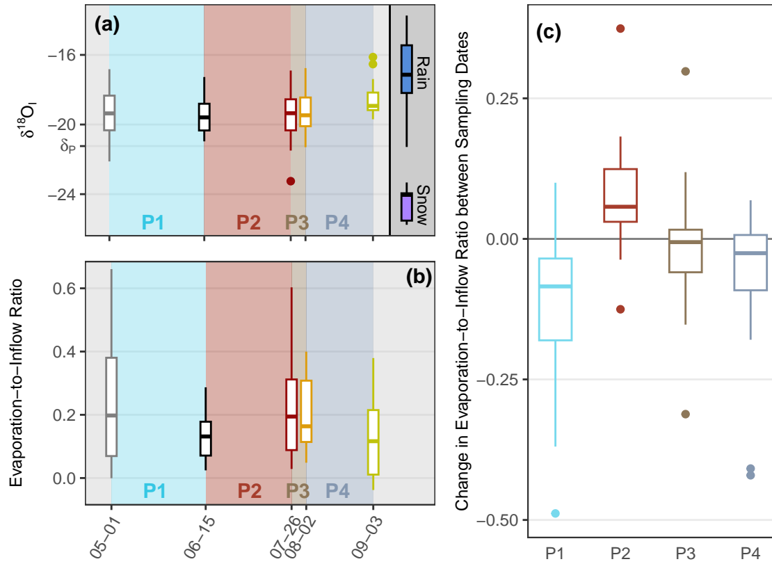
Figure 4. (a) The distribution of \delta^{18}O_1 for each sampling date with rain and snow samples isotope compositions for reference. (b) The distribution of E/I values at all lakes across the four five sampling dates. (c) The distribution of lake-specific change in E/I between the sampling dates was calculated as \Delta[E/I] = [E/I]_{t_2}^{L_n} - [E/I]_{t_1}^{L_n} , where L_n represents a specific lake, and t represents a sampling date.
