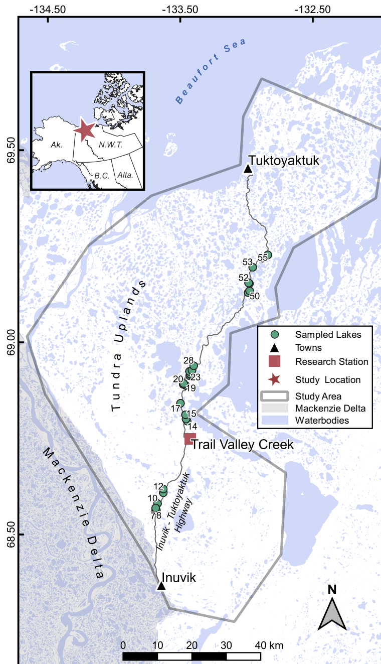
Figure 1. Study area showing locations of thermokarst lakes where water samples for isotope analysis were taken. The locations of the meteorological station study location relative to northwestern North America is shown in Inuvik and the Trail Valley Creek research station inset map. Not all lakes are also shown labeled on the map, but lakes are numbered sequentially from south to north.
