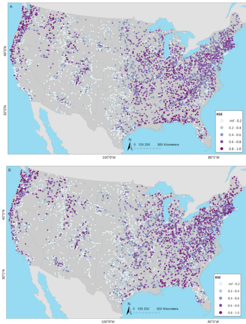
Figure 5: Kling–Gupta efficiency (KGE) based on daily streamflow at U.S. Geological Survey (USGS) gages for (A) National Water Model v2.1 (NWMv2.1) and (B) National Hydrologic Model v1.0 (NHMv1.0). Map Source: (Grannemann, 2010; Natural Earth Data, 2009; ESRI, 2022a; ESRI, 2022b).
