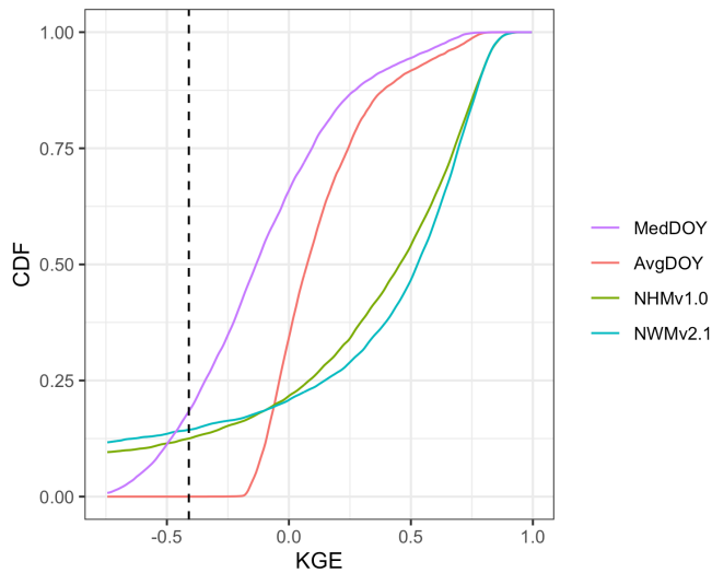
620 Figure 2: Cumulative density function (CDF) for Kling-Gupta efficiency (KGE) scores based on daily streamflow at U.S. Geological Survey (USGS) gages for seasonal benchmarks based on the median day-of-year flows (MedDOY) and average day-of-year flows (AvgDOY) and models: National Water Model v2.1 (NWMv2.1) and National Hydrologic Model v1.0 (NHMv1.0). Dotted vertical line is KGE mean flow benchmark (= -0.41). For sites (n=1 for NWMv2.1 and n=16 for NHMv1.0) for which a KGE could not be calculated (i.e., the modelled timeseries had all zero values for the entire timeseries), these are included as -Infinity in the CDFs.
