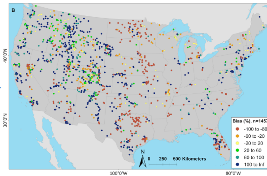
655 Figure 8: Percent bias (PBIAS) maps for National Water Model v2.1 (NWMv2.1) (A) and National Hydrologic Model v1.0 (NHMv1.0) (B), for sites where the KGE score is less than the average day-of-year flow (AvgDOY) benchmark. Cooler colors are where model application is overestimating volume and warmer colors are where model is underestimating volume. Map Source: (Grannemann, 2010; Natural Earth Data, 2009; ESRI, 2022a; ESRI, 2022b).
