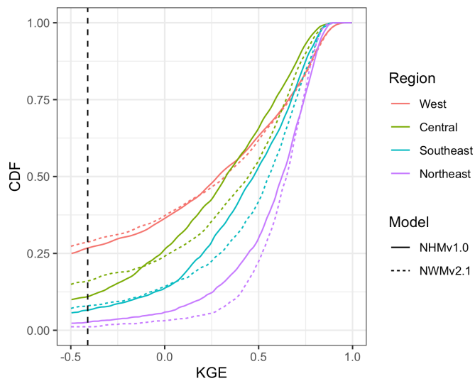
630 Figure 4: Cumulative density function (CDF) for Kling-Gupta efficiency (KGE) scores based on daily streamflow at U.S. Geological Survey (USGS) gages for models: National Water Model v2.1 (NWMv2.1) and National Hydrologic Model v1.0 (NHMv1.0). Dotted vertical line is KGE mean flow benchmark ( =-0.41 ). Regions are further combinations of aggregated ecoregions defined by Falcone (2010): Central ( n=1,450 ) includes Central Plains, Western Plains, and Mixed Wood Shield; Northeast ( n=1,218 ) includes Northeast and Eastern Highlands; Southeast ( n=1,212 ) includes South East Plains and South East Coastal Plains; and West ( n=1,510 ) includes 635 Western Mountains and West Xeric.
