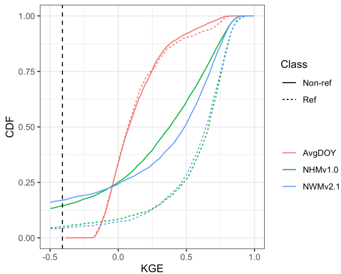
625 Figure 3: Cumulative density function (CDF) for Kling-Gupta efficiency (KGE) scores based on daily streamflow at U.S. Geological Survey (USGS) gages for seasonal benchmark based on average day-of-year flows (AvgDOY) and models: National Water Model v2.1 (NWMv2.1) and National Hydrologic Model v1.0 (NHMv1.0). Dotted vertical line is KGE mean flow benchmark (= -0.41). Reference (Ref, n= 1,115) and Non-Reference (Non-ref, n= 4,274) classifications are from Falcone (2010).
