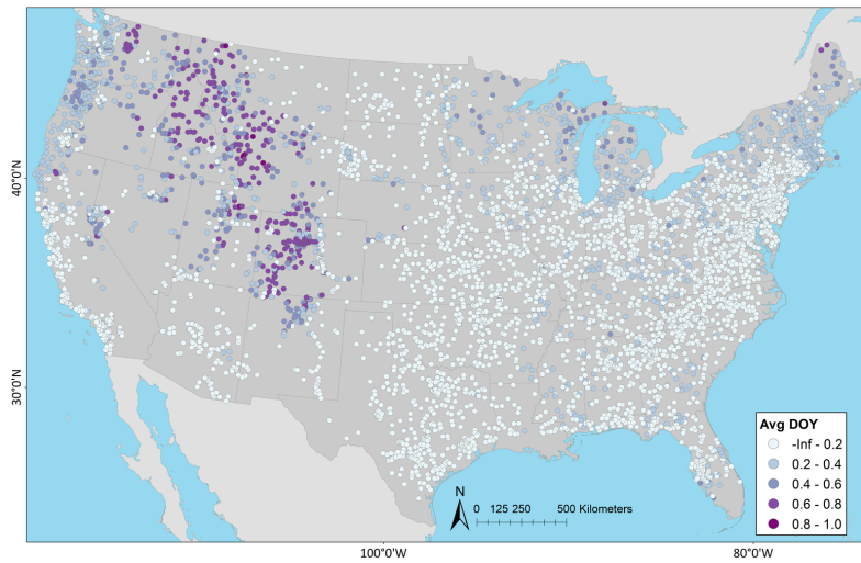
645 Figure 6: Kling–Gupta efficiency (KGE) based on daily streamflow at U.S. Geological Survey (USGS) gages using seasonal benchmark from average day-of-year flows (AvgDOY). Map Source: (Grannemann, 2010; Natural Earth Data, 2009; ESRI, 2022a; ESRI, 2022b).
