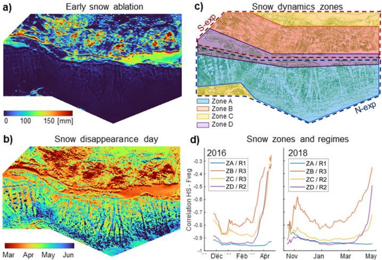
515 Figure 11: Conceptual subdivision of study domain into snow cover evolution regimes, the identification of which is based on maps of cumulative SWE ablation between mid-January and mid-March (a) and snow disappearance day (b) in WY 2018. Resulting zones (c) and evolution of the correlation coefficients between snow depth and vegetation cover fraction in these for WYs 2016 and 2018, resulting in the attribution to a specific regime (d).
