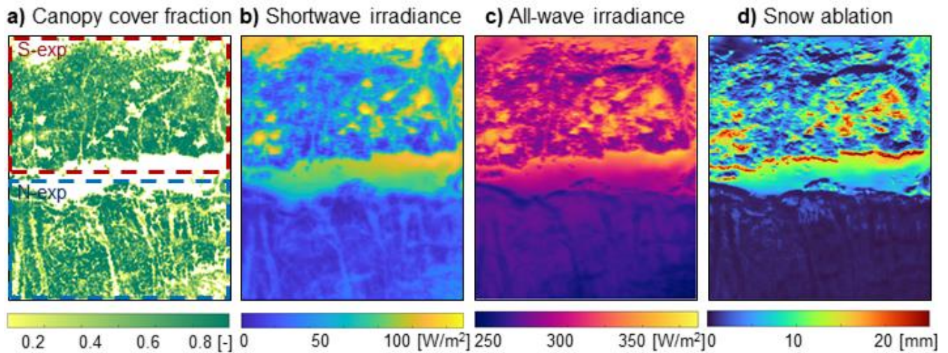
390 Figure 7: Canopy cover fraction and aspect in the sub-domain (a), average incoming shortwave (b) average all-wave irradiance (c), and cumulative SWE ablation (d) between mid-January and end of February for WY 2019.
