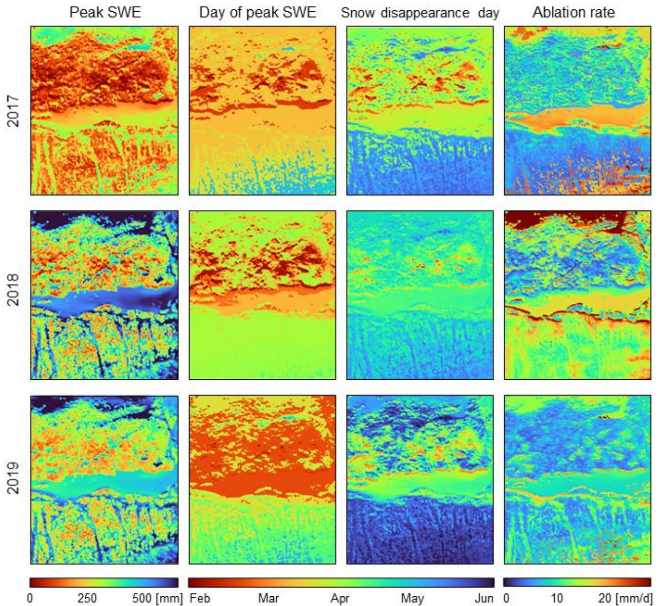
425 Figure 9: Spatial patterns of snow season descriptors for the sub-domain, including peak SWE (1st column), day of peak SWE (2nd col.), snow disappearance day (3rd col.) and ablation rate (4th col.) during three different WYs, namely 2017 (1st row), 2018 (2nd row) and 2019 (3rd row).
