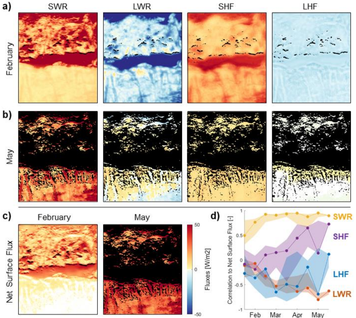
405 Figure 8: Energy flux partitioning into the four surface energy balance components ( net short- and longwave radiations, SWR and LWR; sensible and latent heat fluxes, SHF and LHF ) for two weeks in February (a) and May (b) 2019, respectively, as well as net energy flux at the snow surface (c), areas that have melted out by the time shown are marked black; Correlations (Pearson's R) between individual energy fluxes and net surface energy over the season (d), with lines showing WY 2019 and shaded areas the range of all modelled WYs.
