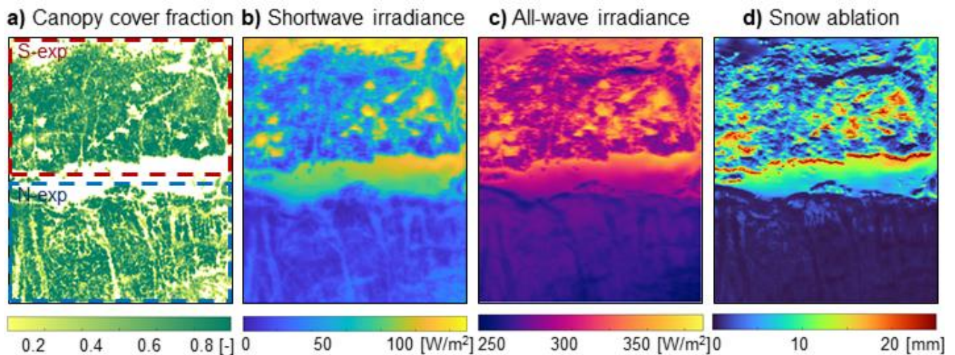
375 Figure 7: Canopy cover fraction and aspect in the sub-domain (a), average incoming shortwave (b) average all-wave irradiance (c), and cumulative snowmelt-SWE ablation (d) between mid-January and end of February for WY 2019.
