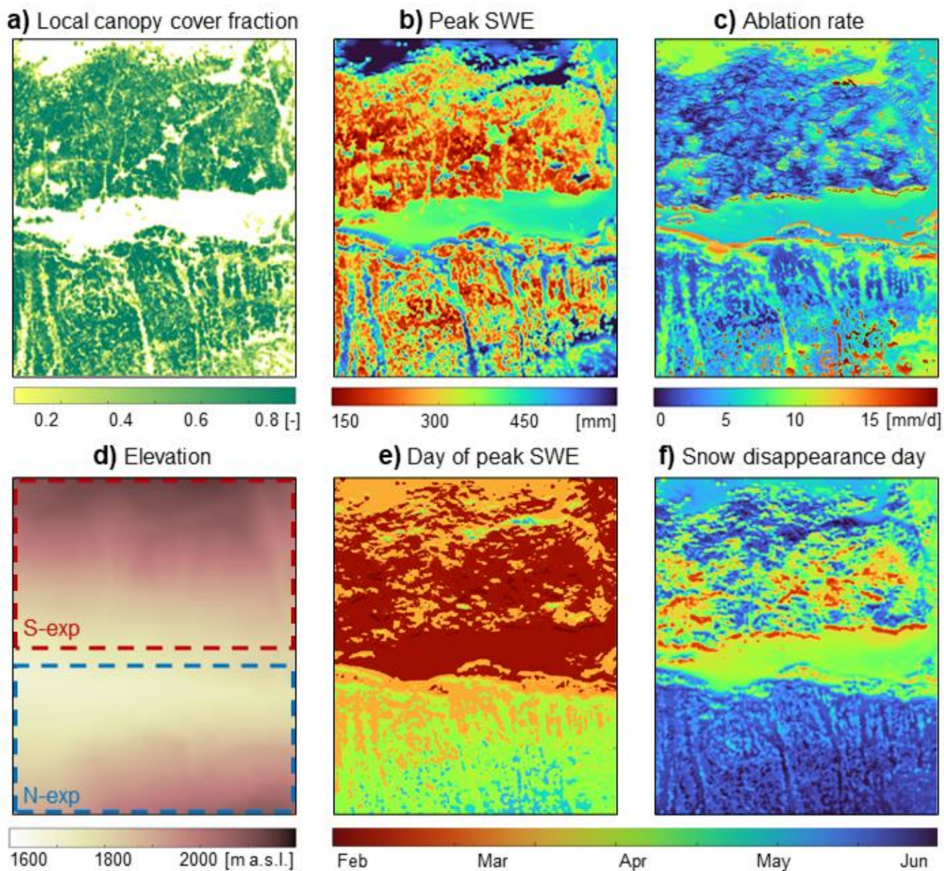
290 Figure 5: Canopy cover (a) and topographic (d) maps, as well as snow season descriptors including peak SWE (b), ablation rate (c), day of peak SWE (e) and snow disappearance day (f), for a sub-section of the model domain and WY 2019.
