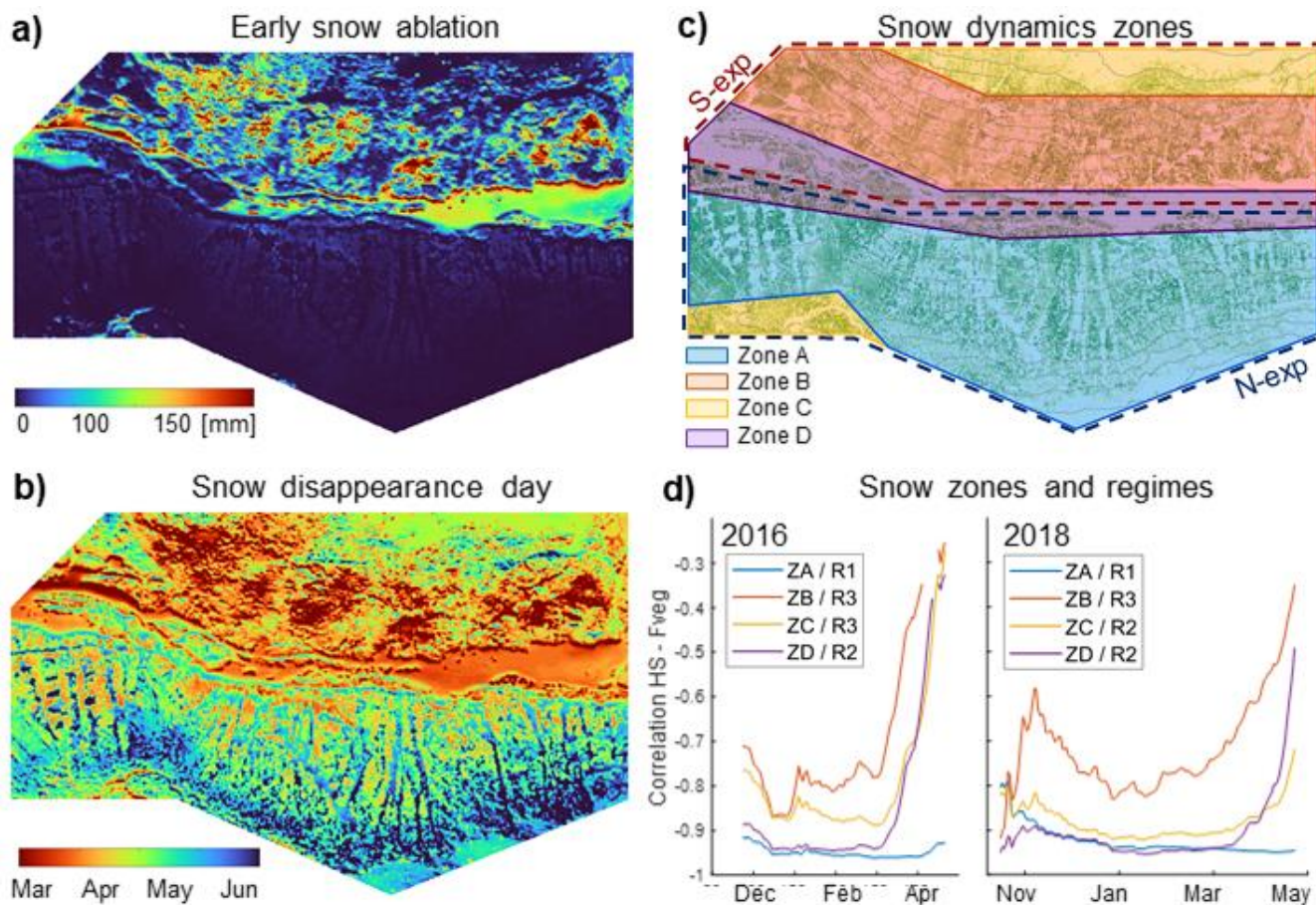
500 Figure 11: Conceptual subdivision of study domain into snow cover evolution regimes, the identification of which is based on maps of melt-cumulative SWE ablation between mid-January and mid-March (a) and snow disappearance day (b) in WY 2018. Resulting zones (c) and evolution of the correlation coefficients between snow depth and vegetation cover fraction in these for WYs 2016 and 2018, resulting in the attribution to a specific regime (d).
