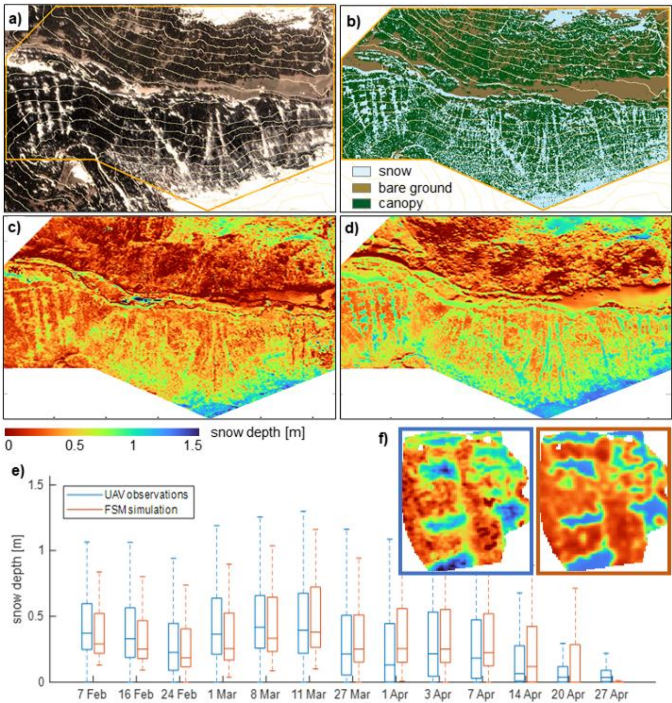
180 Figure 3: Examples of plausibility checks performed to verify the model use case, including comparisons of 1) satellite RGB imagery acquired by Planetscope on 28. April 2018 (a) and snow cover extent simulated by FSM2 on the same day (b); 2) snow depth distribution derived from ALS data (c) and simulated by FSM2 (d); and 3) snow depth statistics of UAV-LiDAR derived snow maps at the north-exposed site and resulting from FSM2 (e) and observed and modelled spatial distribution of the 8 March 2020 campaign (f).
