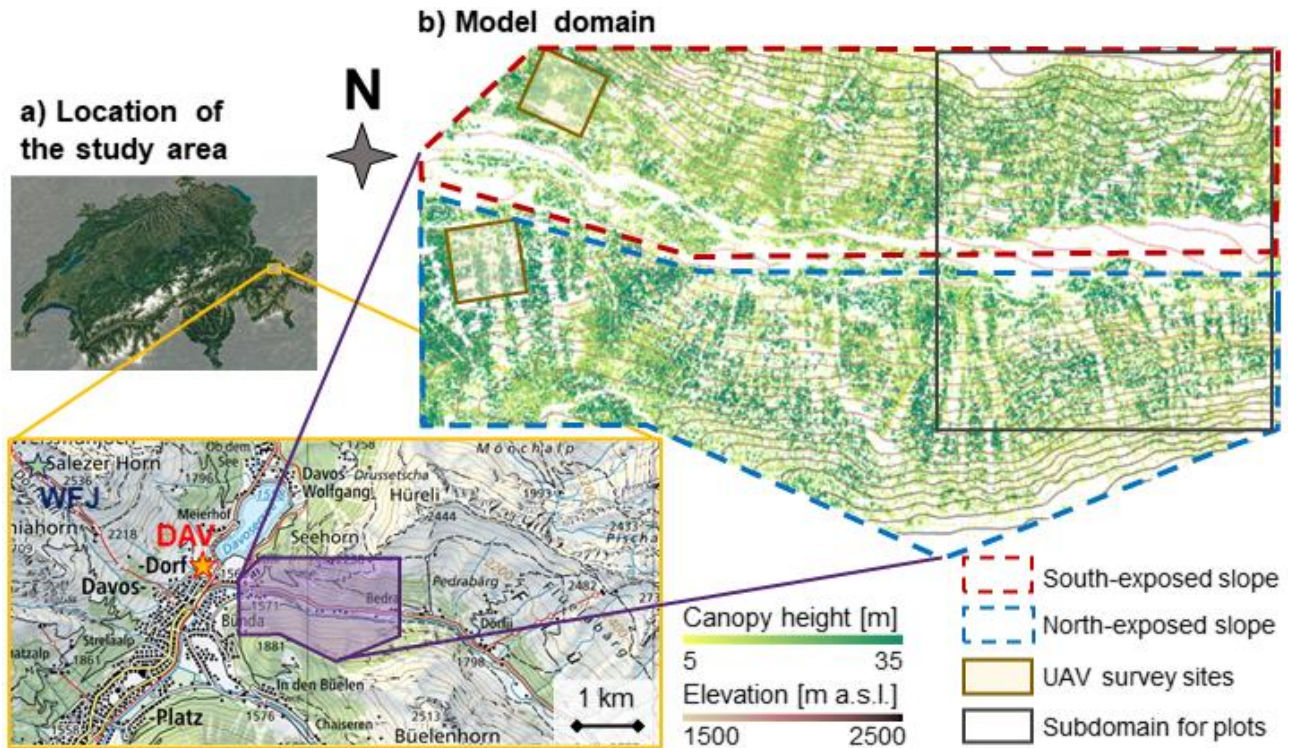
105 Figure 1: Overview of the study area: (a) Location of the model domain within Switzerland and on the topographic map of the Davos area (source: swisstopo), including locations of the automatic weather stations DAVSLF and WFJ; (b) Canopy height model and contour lines (equidistance: 50m), including locations of the sites from Koutantou et al. (2022) and of the subdomain shown in Figures 5 and 7-9.
