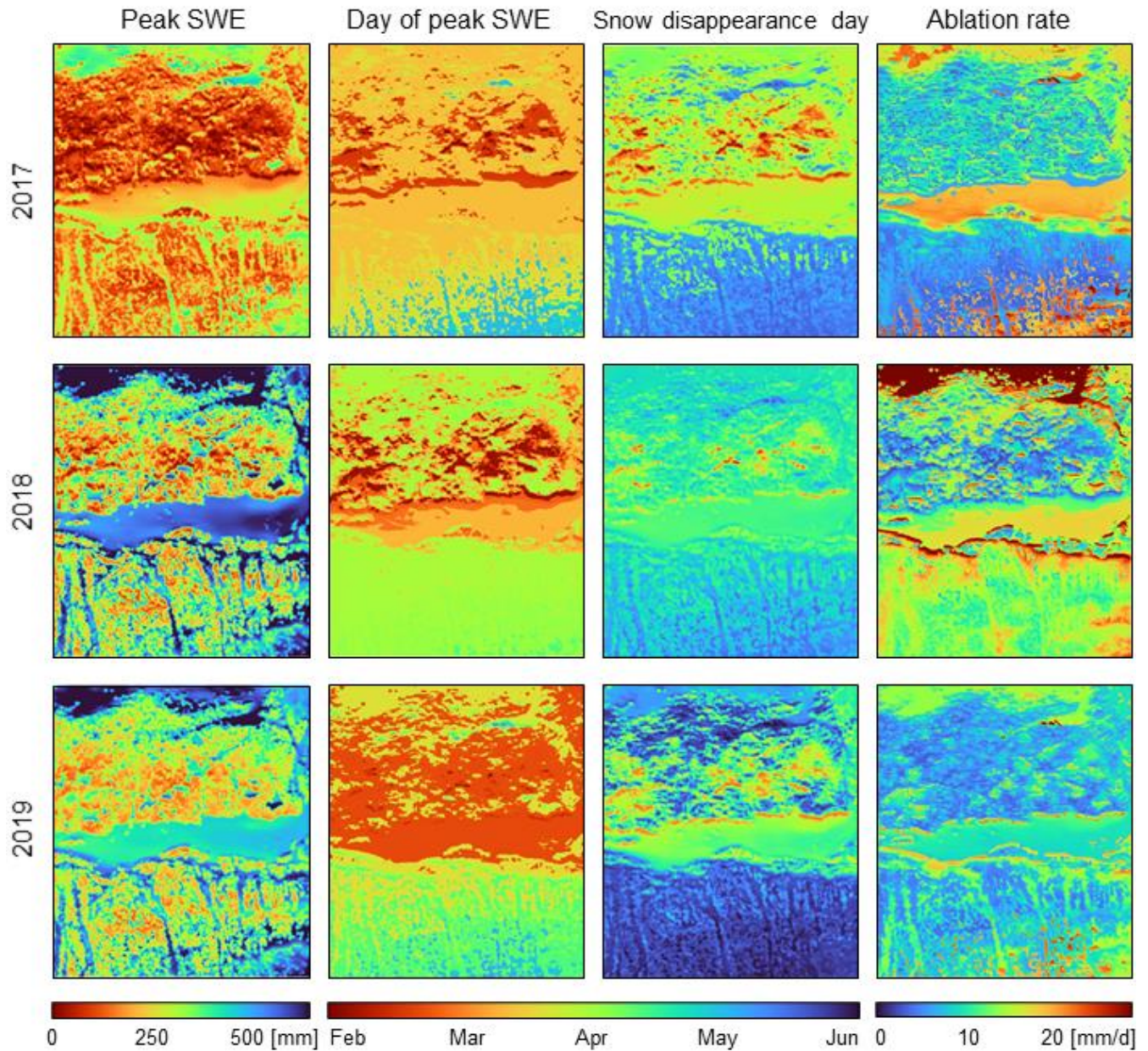
410 Figure 9: Spatial patterns of snow season descriptors for the sub-domain, including peak SWE (1st column), day of peak SWE (2nd col.), snow disappearance day (3rd col.) and ablation rate (4th col.) during three different WYs, namely 2017 (1st row), 2018 (2nd row) and 2019 (3rd row).
