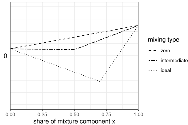
Figure 2. Mixing types of water retention characteristics in binary mixtures (adapted from concept for porosity in binary mixtures in Zhang et al. (2011)).
