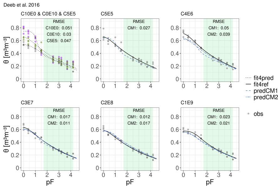
Figure 7. Water retention curves of all 7 binary mixtures of excavated deep soil horizon (C0E10) and green waste compost (C10E0). Observations („obs“) are represented by gray dots, fitted curves are represented by black lines (i.e reference curves as solid lines, „fit4ref“, see Tab. A3 for fitting parameters and model specification). The predicted curves („pred“) are represented by blue dashed lines. CM1 stands for the basic compositional model and CM2 for the extended scheme. The first panel (top, left) assembles the fitted water retention curves of the pure components and the intermediate mixture as dotted black lines („fit4pred“), which constitute the input for the compositional model. The particular RMSE describes the deviation between the predictions and the reference curves. Note that C5E5 is not predicted by the extended model scheme because it is considered the intermediate mixture.
