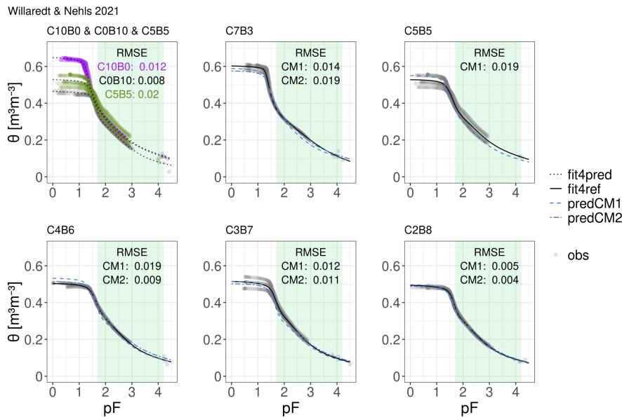
Figure 5. Water retention curves of all seven binary mixtures of ground bricks (C0B10) and green waste compost (C10B0). Observations („obs“) are represented by gray dots, fitted curves are represented by black lines (i.e reference curves as solid lines, „fit4ref“, see Tab. A1 for fitting parameters and model specification). The predicted curves („pred“) are represented by blue dashed lines. CM1 stands for the basic compositional model and CM2 for the extended scheme. The first panel (top, left) assembles the fitted water retention curves of the pure components and the intermediate mixture as dotted black lines („fit4pred“), which constitute the input for the compositional model. The particular RMSE describes the deviation between the predictions and the reference curves. Note that C5B5 is not predicted by the extended model scheme because it is considered the intermediate mixture.
