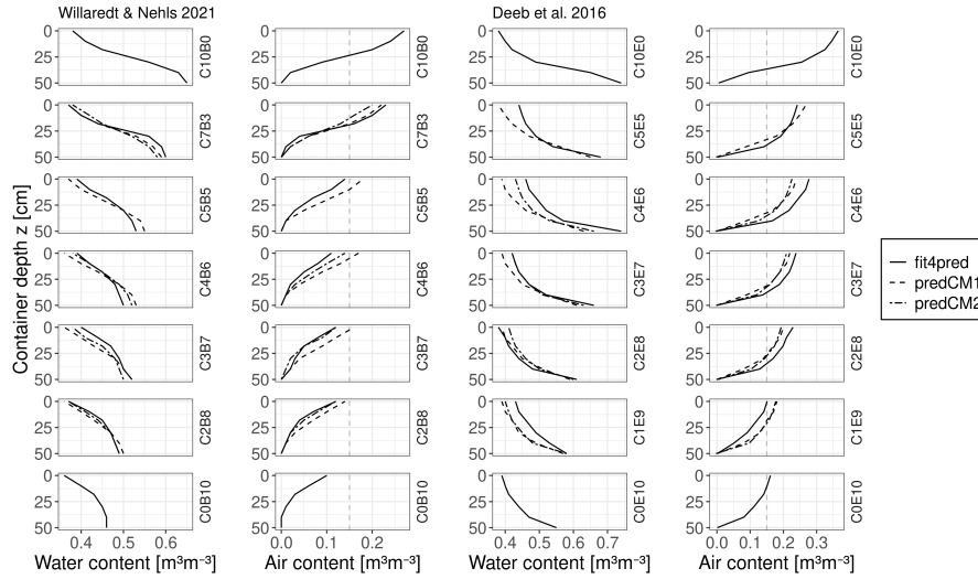
Figure 10. Distribution of volumetric water and air content over different depths at hydrostatic equilibrium in a container (corresponding to pF = 1.7 at the top of the container) filled with a constructed Technosol formulated as a binary mixture of: green waste compost and ground bricks (left) and green waste compost and excavated deep soil (right). The solid line indicates the reference WRCs, the dashed lines indicate predictions using the basic scheme (CM1) or the extended scheme (CM2) respectively. The grey vertical line indicates the minimum volumetric air content in horticultural substrates favourable for root growth (Caron et al., 2015).
