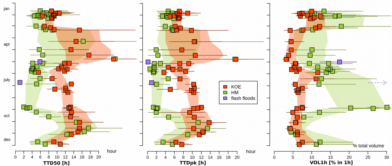
Figure 9: Properties of the simulated transfer time distributions: the median transfer time (TTD50 [h], left panel ), the peak flow lag time (TTDpk [h], center), the runoff response concentration in one hour (VOL1h [%], right panel). The events are ordered by calendar day. The orange and green envelopes correspond to the average calendar values, based on the 3 closest estimates and taking into account the uncertainties of the metric (TTD50, TTDpk or VOL1h) assessments. The purple arrow on the third panel points to VOL1H of the flash flood of July 2016 which exceeds the graph scale (VOL1H = 64.3%).
