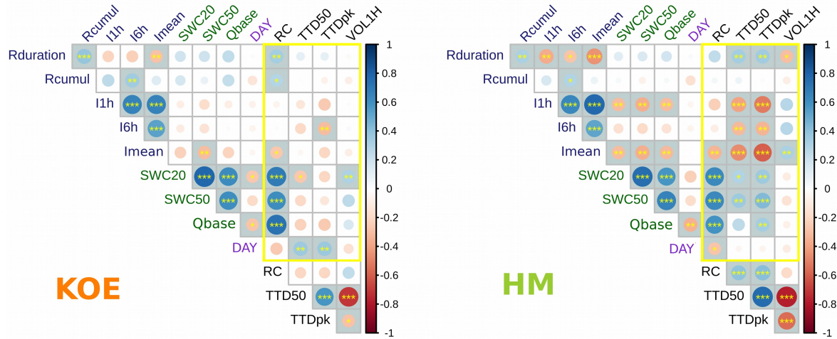
435 Figure 11: Kendall correlation coefficients between rainfall (blue), catchment hydrological states (green), seasonal cycle (DAY of the year) and outlet runoff properties (black). See section 3.2 for more details on properties. The left and the right panels refer to KOE and HM catchment section respectively. The size and the color of the circles are related to the Kendall coefficients. The yellow box highlights the scores of interest for our study. The blue background and the redstars indicate the significant correlations: *** when p\text{-value} < 10^{-3} ; ** when 10^{-3} < p\text{-value} < 10^{-2} ; * when 10^{-2} < p\text{-value} < 2 \cdot 10^{-2} .
