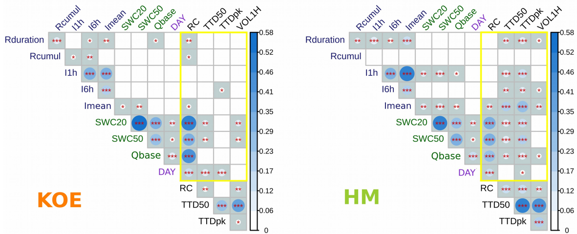
440 Figure 12: Hoeffding correlation coefficients between rainfall (blue), catchment hydrological states (green), seasonal cycle (DAY of the year) and outlet runoff properties (black). See section 3.2 for more details on properties. The left and the right panels refer to KOE and HM catchment section respectively. The size and the color of the circles are related to the Hoeffding coefficients. The yellow box highlights the scores of interest for our study. The blue background and the redstars indicate the significant correlations: *** when p\text{-value} < 10^{-3} ; ** when 10^{-3} < p\text{-value} < 10^{-2} ; * when 10^{-2} < p\text{-value} < 2 \cdot 10^{-2} .
