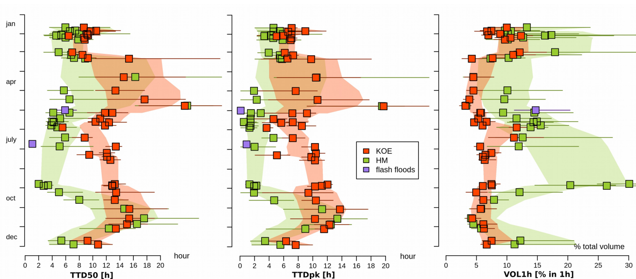
390 Figure 89: Properties of the simulated transfer time distributions: the median transfer time (TTD50 [h], left panel), the peak flow lag time (TTDpk [h], center), the runoff response concentration in one hour (VOL1h [%], right panel). The events are ordered by calendar day. The orange and green envelopes correspond to the average calendar values, based on the 3 closest estimates and taking into account the uncertainties of the metric (TTD50, TTDpk or VOL1h) assessments.
