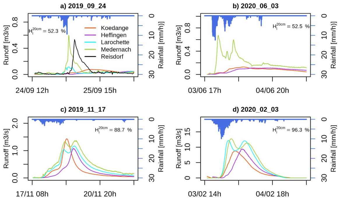
245 Figure 5: Four rainfall-runoff events that have occurred in the Ernz Blanche catchment with different soil moisture conditions. Rainfall amounts are calculated for the Ernz Blanche catchment at Medernach (79 km 2 ). The runoff time series are observed at Koedange (31.1 km 2 orange), Heffingen (48.8 km 2 , purple), Larochette (69.4 km 2 , cyan), Medernach (79 km 2 , green) and Reisdorf (100.6 km 2 , black). H_i^{20cm} correspond to the soil moisture conditions observed at 20 cm in depth before each event.
