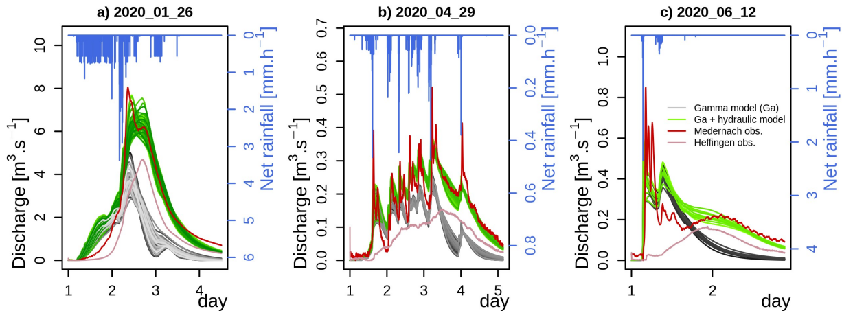
Figure 78: Examples of simulated events on the Heffingen-Medernach catchment section. The grey lines correspond to the HM runoff transfer only, while the green lines correspond to this runoff transfer + the hydraulic transfer of the Heffingen inflow.
