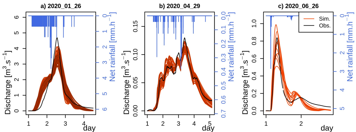
Figure 67: Examples of simulated events for the Koedange subcatchment. Event a) is representative of the winter event simulations. The displayed event on panel b) is representative of the well simulated events. On panel c) is displayed the summer event on 26/06/2020, where the peak discharge tends to be underestimated while the second moderate event is overestimated.
