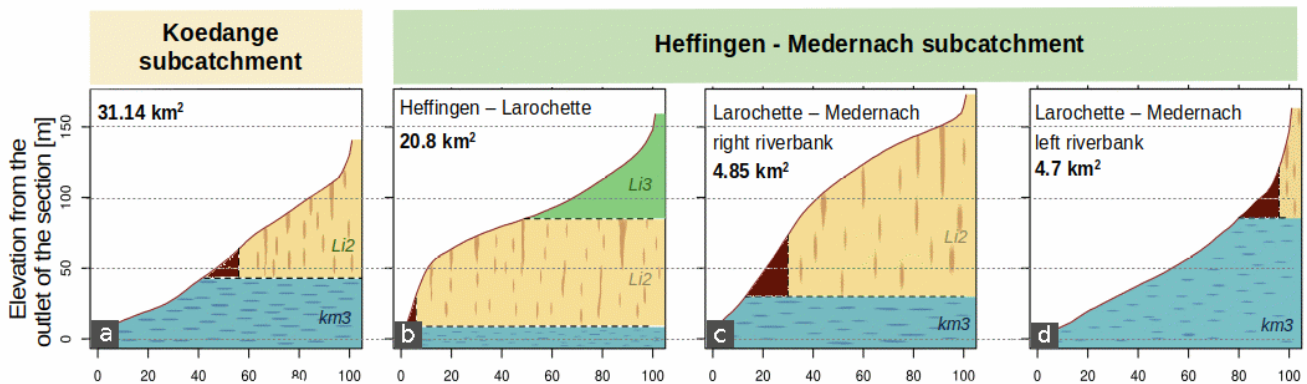
175 | Figure 3: Geological profiles in the Ernzt Blanche catchment. Elevation distribution of a) the Koedange subcatchment, b,c,d) 3 subsections of the Heffingen-Medernach area: b) the Larochette – Heffingen subsection; c) the right riverbank of the Medernach – Larochette subsection; d) the left riverbank of the Medernach – Larochette subsection. Elevation is counting-counted from the minimum elevation of each section. The geological substrates are designed according to their proportion in each section. Blue: Marls from middle Keuper (Km3); dark yellow: Luxembourg sandstone (Li2);- green: Strassen marls (Li3), darklight brown: conglomerates, marls and altered limestone-alteration.
