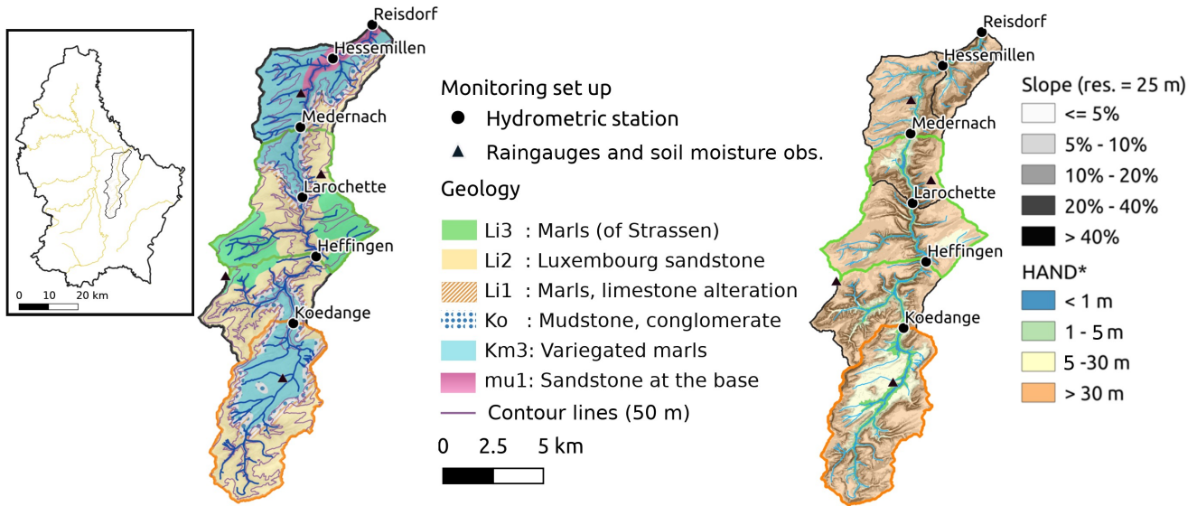
165 | Figure 1: Ernzt Blanche catchment (102 km 2 ). Discharge and rainfall monitoring network; Left: geological characteristics (see Kausch & Maquil (2018) for more details). Right: topographical properties: slopes and Height Above the Nearest Drainage (HAND, Nobre et al., 2011). The Koedange subcatchment (KOE) and Heffingen-Medernach section (HM) are highlighted with orange and green contours respectively.
