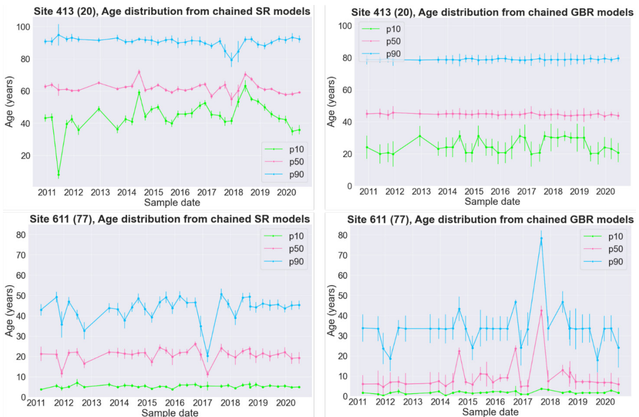
615 Figure 9: Temporal patterns in the estimated values for selected age percentiles at two sites based on SR models (left) and GBR models (right). Points and error bars represent the median and MAD for the relevant 40-member model ensemble, respectively. MapIDs in brackets link to the location of the sites on the map in Figure 5.
