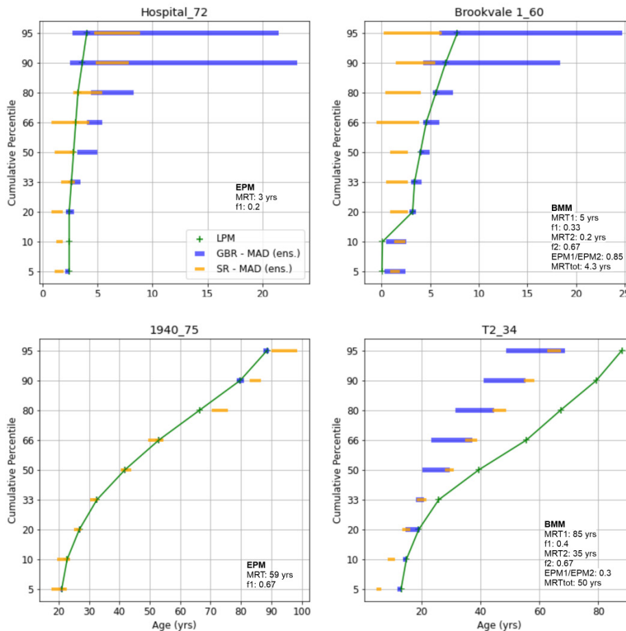
395 Figure 6: Age distributions for selected samples based on LPMs (Morgenstern et al. 2018) compared to the chained SR and GBR models developed in this study (bars represent ensemble MAD – see Supplementary Fig. S5 for further discussion of this). The legend in the upper left sub-figure is representative for all sub-figures. The mapID following the underscore links with the location of the site on Fig. 3. Age distribution parameters shown are: MRT (MRT1, MRT2) and the fraction (f1, f2) of exponential to total flow volume for each EPM; EPM1/EMP2 is the ratio between two EPMs in a BMM; and MRTtot is the 400 MRT between the two EPMs in a BMM.
