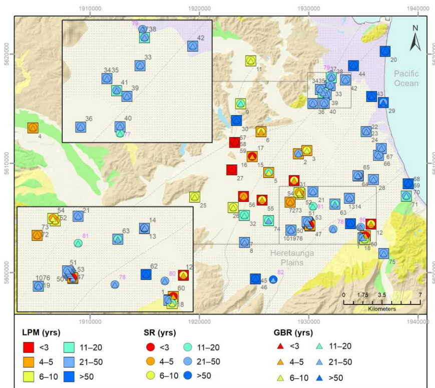
Figure 5: Comparison between the LPM, and the SR and GBR modelled ages for the 50th percentile. The geological formations shown on the background map (Heron, 2020) are explained in Fig. 1. Labels correspond to mapIDs for each site; +Grey numbers: sites used in the development of the metamodellers (mapIDs 1-76); Pink numbers: sites without LPM data, used for predictions (mapIDs 77-82).
