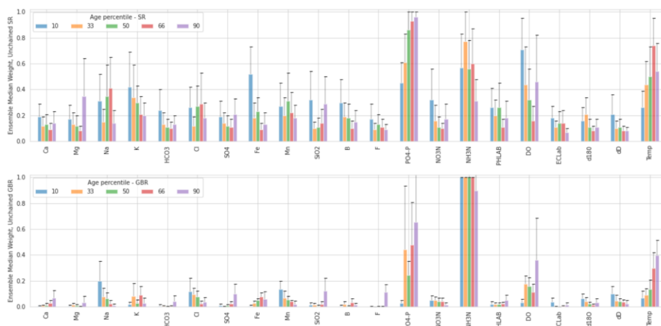
530 Figure 8: Ensemble median variable weights (scaled from 0 to 1) from unchained SR and GBR models, for selected percentiles in the age distribution (10th, 33rd, 50th, 66th and 90th, shown from left to right for each variable). Error bars represent the ensemble median absolute deviation.
